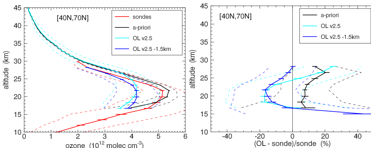
Fig. 10. Comparison of collocated OL2.5 (with and without a -1.5 km shift applied) and sonde ozone profiles in the Northern Hemisphere ( 40\text{--}70^\circ\text{N} ). Averaged ozone profiles and the averaged a priors used in the OL retrieval are shown in the left panel, percent differences with respect to sondes are shown in the right panel. Dashed lines indicate one standard deviation divided by the square root of the number (30) of collocations. Evidently, the OL2.5 data compare worse than their own a priors for altitudes of 24 km and lower.
