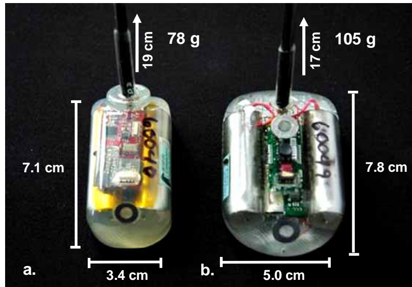
Fig. 3.2 Example of (a) a conventional satellite transmitter that provide animal positions (Spot5) and (b) a device that combined such a satellite transmitter with an archival tag to provide animal positins, dive depth, light and temperature data (Splash), both from Wildlife Computers, USA.
