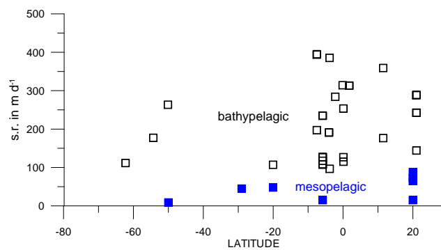
Fig. 5. Sinking rates of particles estimated for the mesopelagic zone (filled squares, from alkenone analysis, Müller and Fischer, 2001, 2003; see text) compared to sinking rates (normalized values from the correlation method, Table 1) determined from flux patterns of upper and lower traps (bathypelagic zone; open squares). Note that all sinking rates from the bathypelagic zone exceed those estimated for the upper water column suggesting increasing sinking rates with depth.
