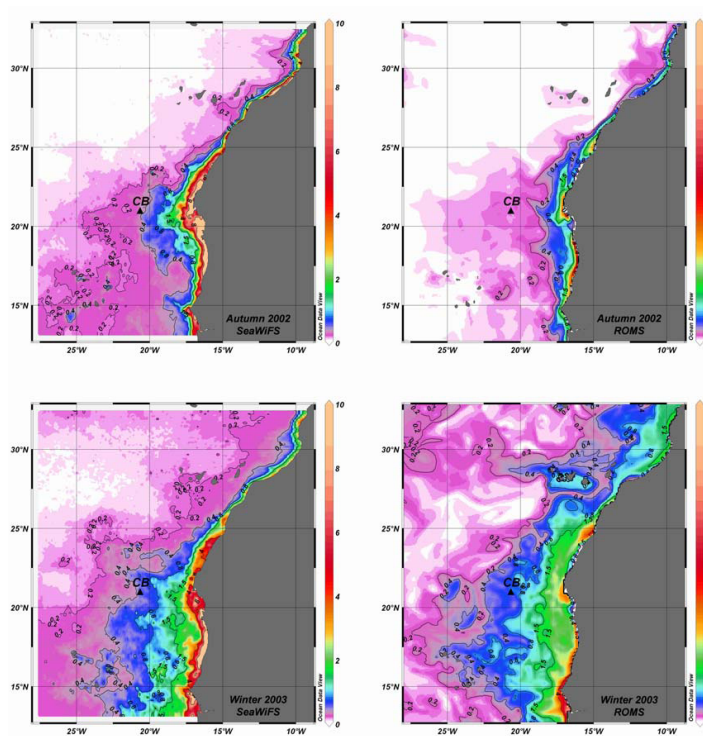
Fig. 8. (b) Seasonal surface chlorophyll distribution ( \text{mg m}^{-3} ) in autumn (mid-September to mid-December) 2002 and winter (mid-December to mid-March) 2003 as inferred by SeaWiFS and simulated by the model.
