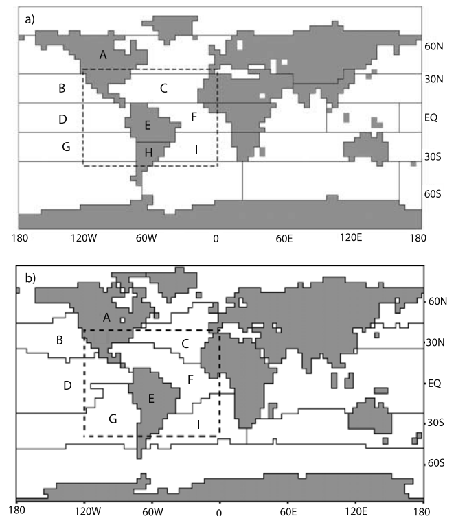
Figure 1. Source regions for tagging experiments of water vapor and \delta^{18}\text{O} of precipitation in (a) GISS II (1980–1997) and (b) ECHAM-4 T30 CTR simulation [Werner et al. , 2001]. Source regions relevant to the tropical Americas regions (outlined in dashed thick black line) are indicated with capital letters: A, North America; B, tropical North Pacific; C, tropical North Atlantic; D, equatorial Pacific; E, tropical South America; F, equatorial Atlantic; G, tropical South Pacific; H, subtropical South America; and I, tropical South Atlantic. Note that H forms part of region E in Figure 1b.
