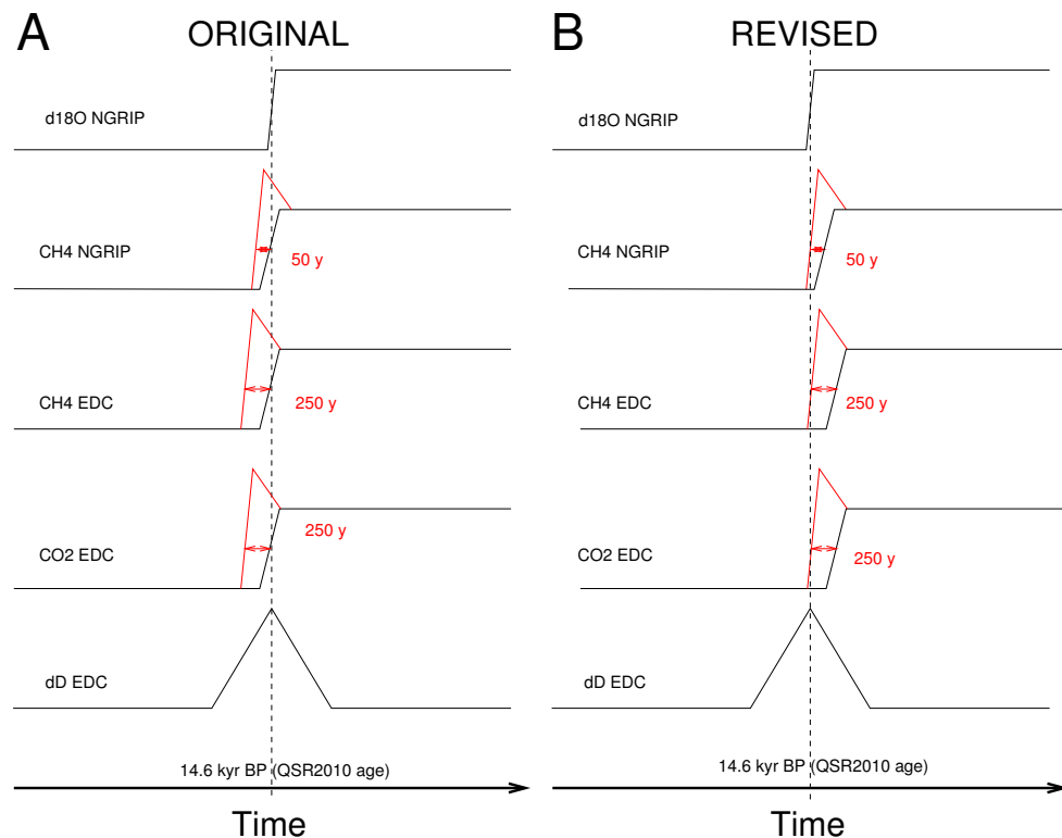
Fig. 3. Conceptual sketch of ice core synchronisation of NGRIP and EDC via CH 4 for 14.6 kyr BP, the onset of the Bølling/Allerød warm period. (A): Following the dating of Lemieux-Dudon et al. (2010). (B): Proposed revised dating, if not CH 4 measured in situ in ice cores, but potentially atmospheric CH 4 are taken for synchronisation. From top to bottom: NGRIP δ 18 O, NGRIP CH 4 , EDC CH 4 , EDC CO 2 , EDC δD. Black lines are in situ ice core measurements, red lines are potentially underlying atmospheric records. Red numbers indicate the dating offset at mid-transition points between ice core and atmospheric gas records.
