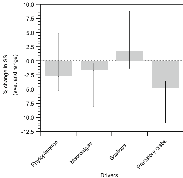
Fig. 5. Percent changes to sum of squares, SS, of the 1996–2003 simulation after the forcing of biomass changes of several functional groups ‘drivers’. Drivers were applied in all possible sequences and combinations and SS was corrected for artificial improvements caused by the fitting of the driver’s dynamics. Average change (bar) and range (line) are displayed. Negative values (i.e. decrease in SS) indicate an improvement in fit.
