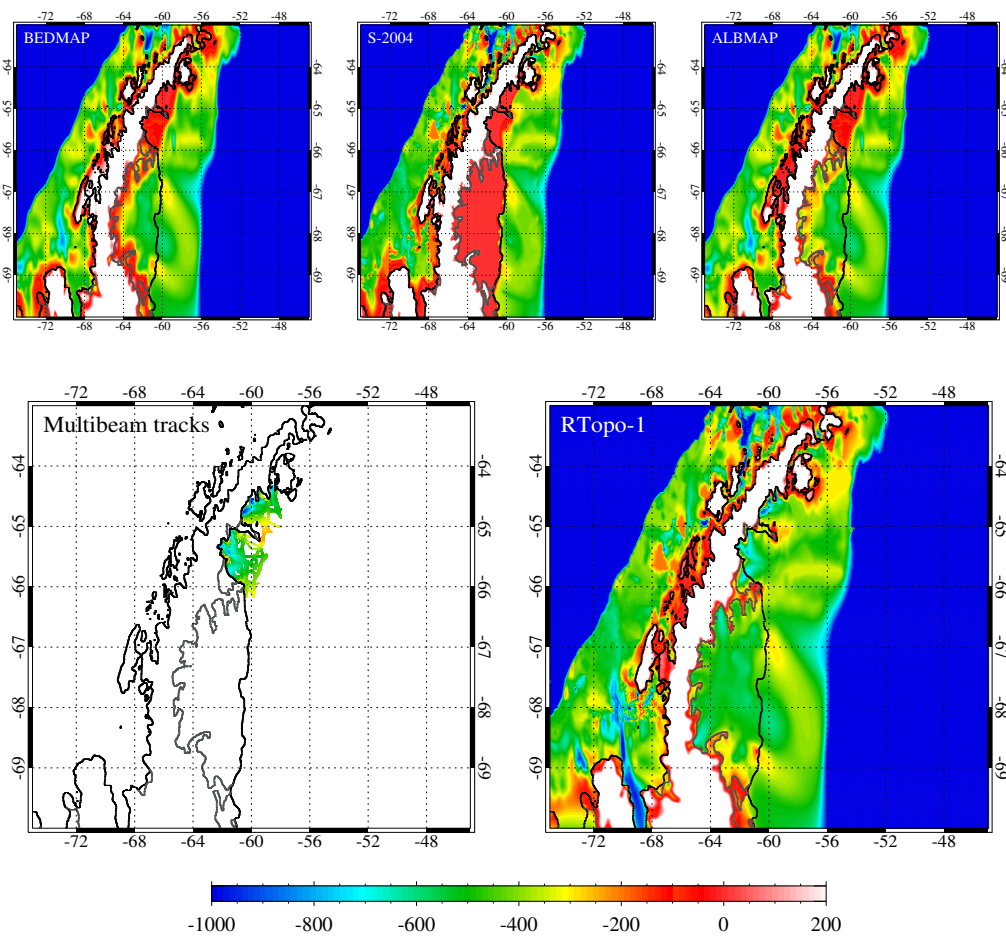
Figure 5: Different representations of bathymetry (bedrock topography) in the area of the Larsen Ice Shelves. Top row: BEDMAP (left), S-2004 (middle), and ALBMAP (right). Bottom row: Multibeam track data (left), and the RTopo-1 product (right). Ice shelf front and coastline are marked with a black line, ground-line location with a grey line.
