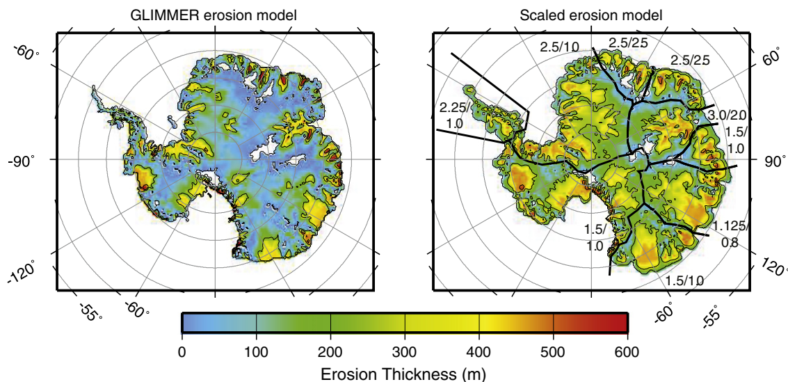
Fig. 4. Modeled erosion pattern before (left) and after (right) power-law scaling. Maximum and minimum scaling factors for each drainage system are noted outboard of each system. The scaling factors tune the erosion volumes to match the targets based on sediment volumes with the caveat that drainage valleys should not be overfilled.
