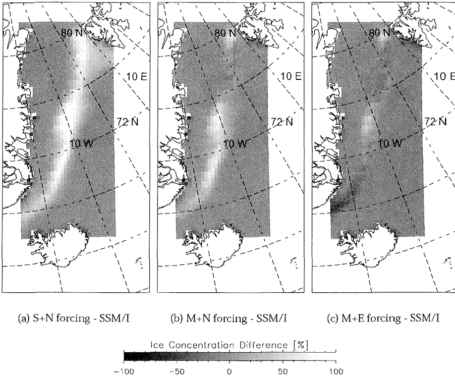
Figure 4.8: Sea ice concentration differences for mean sea ice concentrations in November 1994 as depicted in Figure 4.3 for different forcing combinations minus remote sensing data (SSM/I) for the Greenland Sea region. Bright areas indicate model overestimating sea ice concentrations as compared to SSM/I data, dark areas indicate model underestimation.
