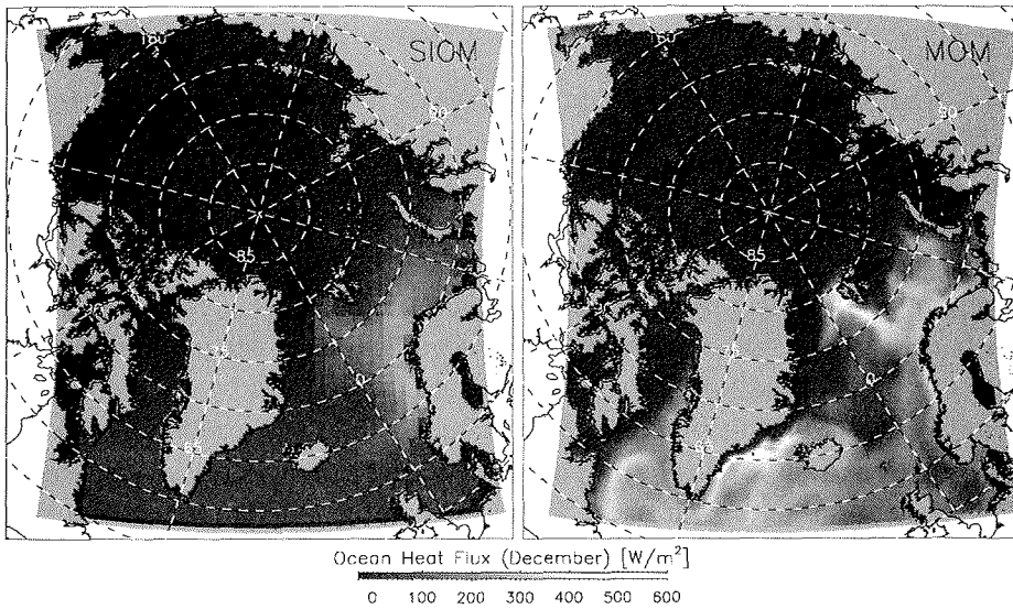
Figure 2.10: This Figure gives an example of a previous (SIOM, left) and a new (MOM, right) forcing field for the oceanic heat flux from the deep ocean into the mixed layer for December. The resolution is adopted to the new resolution of the ice model. The new fields show more variability in both regional pattern and absolute values.
