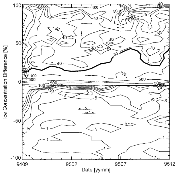
Figure 4.9: Monthly mean Greenland Sea sea ice concentration differences for the reference period as a contour plot of numbers of occurrence for the SIOM oceanic and NCEP atmospheric forcing combination (S+N setup).
