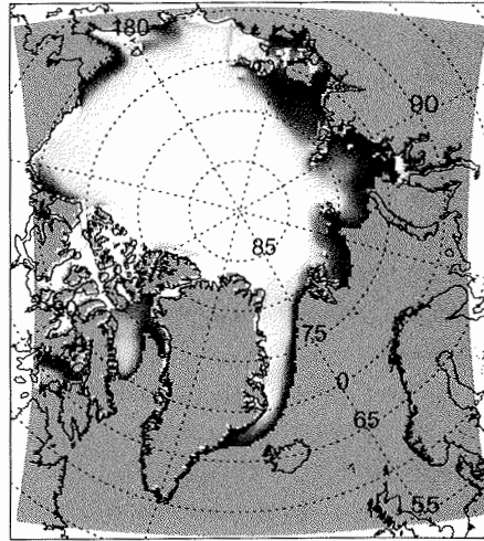
(b) MOM ocean + NCEP atmosphere
