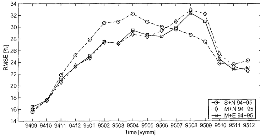
Figure 4.1: Root-Mean-Square Error of sea ice concentration for the reference period of September 1994 to December 1995. The mean RMSE for the S+N set-up is 26.26 \pm 4.93\% , for the M+N set-up 25.65 \pm 4.97\% , and for the M+E set-up 25.51 \pm 4.64\% .
