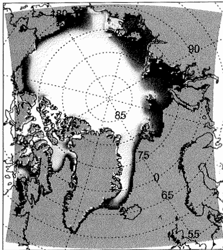
(a) SIOM ocean + NCEP atmosphere
