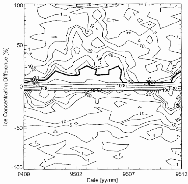
Figure 4.14: Monthly mean Barents Sea sea ice concentration differences for the reference period as a contour plot of numbers of occurrence for the MOM oceanic and NCEP atmospheric forcing combination (M+N setup).
