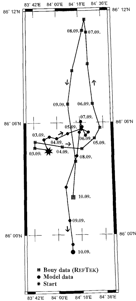
Figure 6.8: Twelve-hourly positions of a geophysical REFTEK-Buoy deployed during ARKTIS XVII/2 marked with squares. Corresponding modelled sea ice drift positions are marked with circles.
