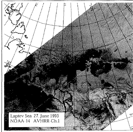
Figure 2.1: Satellite image of the Laptev Sea taken by the NOAA-14 satellite with AVHRR Channel 1 on 27 June 1995. (J. Bareiss, 2003, pers. comm.)
