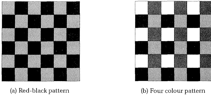
Figure 2.7: Illustration of the relaxation scheme. The two colour relaxation is commonly known as red-black relaxation, the four colour pattern shows that the four point sets are decoupled.
