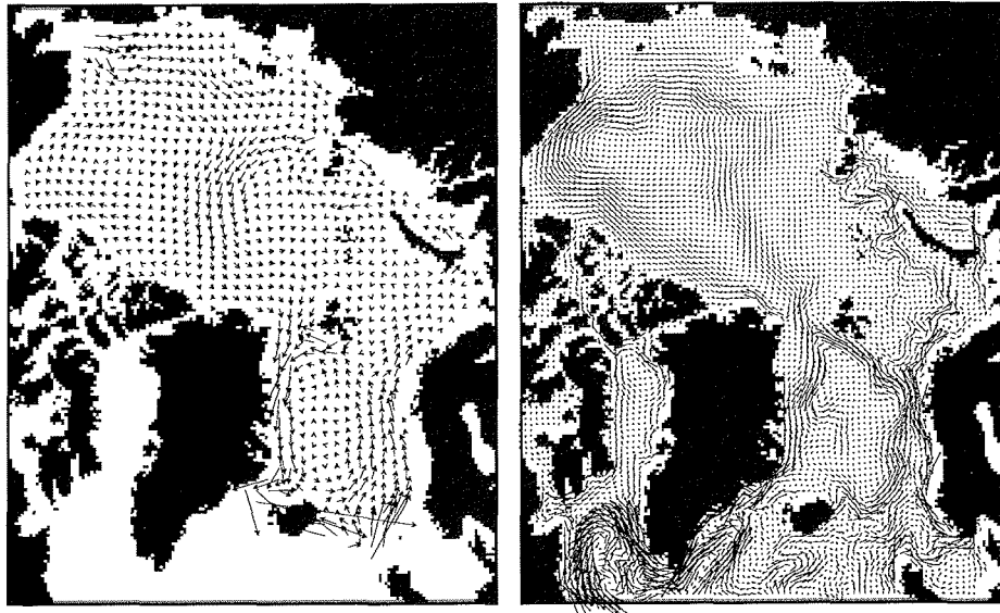
(a) Previous ocean current field for all seasons
