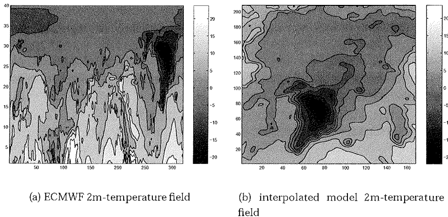
Figure 2.8: Example of an original gridded forcing field for 2 m-air temperature from ECMWF analysis data for the Northern Hemisphere (a) and an interpolated field for the model forcing (b). The numbers on the axis give the x- and y-coordinates for the grids. The ECMWF data are on a 320 \times 161 points grid, but only the northern part of the Northern Hemisphere is displayed. The sea ice model has 169 \times 209 grid points.
