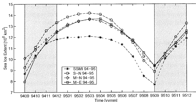
Figure 4.7: Sea ice extent for the reference period of September 1994 to December 1995. The freezing season is shaded grey.
