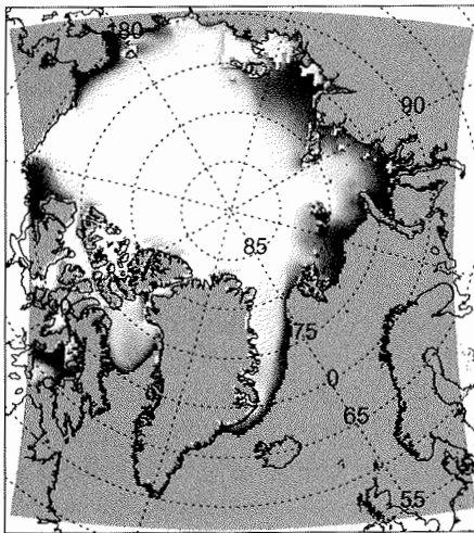
(c) MOM ocean + ECMWF atmosphere
