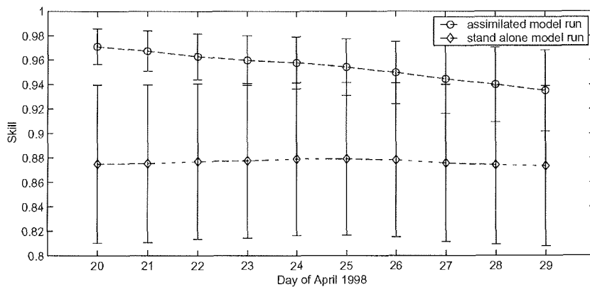
Figure 6.2: Skill of sea ice concentration model results and SSM/I data for an assimilated and a stand alone model run for the whole Arctic for late April 1998. Also shown are the standard deviations as defined in (6.2).
