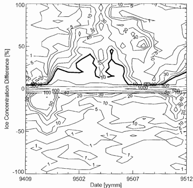
Figure 4.15: Monthly mean Barents Sea sea ice concentration differences for the reference period as a contour plot of numbers of occurrence for the MOM oceanic and ECMWF atmospheric forcing combination (M+E setup).
