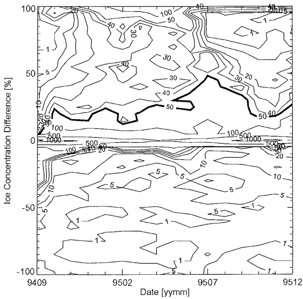
Figure 4.10: Monthly mean Greenland Sea sea ice concentration differences for the reference period as a contour plot of numbers of occurrence for the MOM oceanic and NCEP atmospheric forcing combination (M+N setup).
