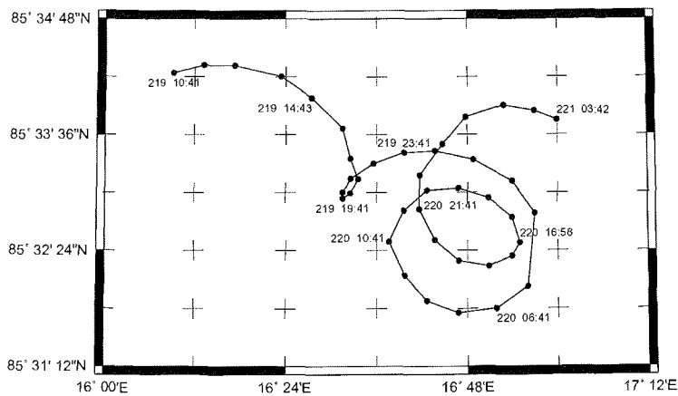
Figure 7.1: Drift of a REFTEK station deployed on sea ice during RV POLARSTERN cruise ARKTIS XVII/2 in summer 2001 for 41 hours. The drift starts at day 219 (07 August 2001) at 10:41 h and ends at day 221 (09 August 2001) at 03:42 h. The dots mark hourly position recordings.
