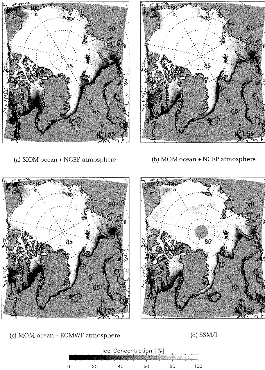
Figure 4.3: Same as Figure 4.2 but for November 1994 as an example of early winter conditions.
