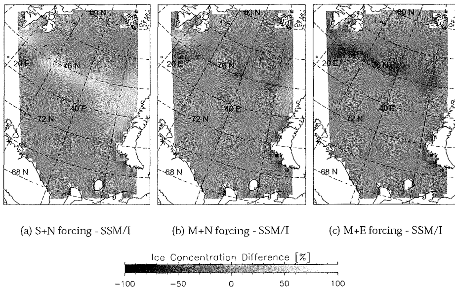
Figure 4.12: Sea ice concentration differences for monthly mean sea ice concentrations as depicted in Figure 4.3 for different forcing combinations minus remote sensing data (SSM/I) for the Barents Sea region. Bright values indicate model overestimating sea ice concentrations as compared to SSM/I data, dark values indicate model underestimation.
