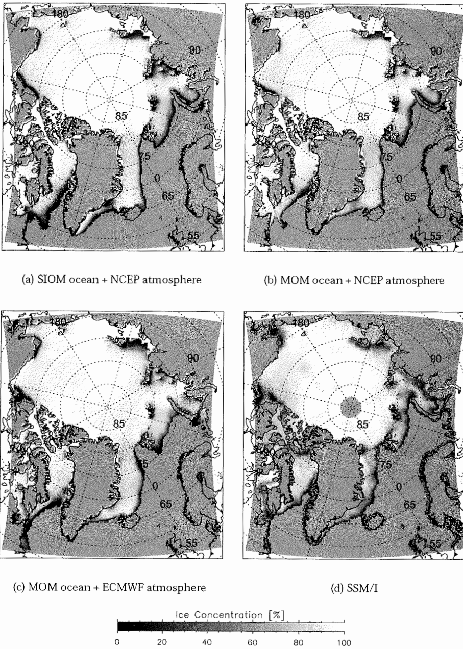
Figure 4.5: Same as Figure 4.2 but for June 1995 as an example of meltdown conditions.
