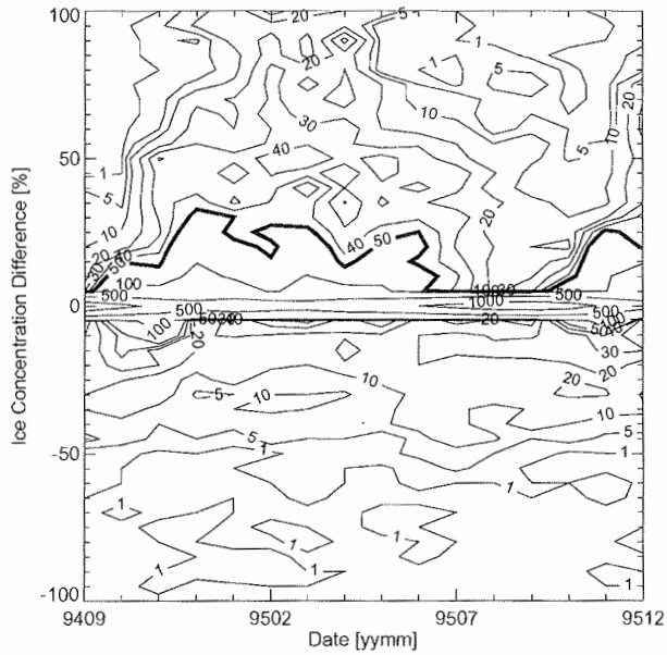
Figure 4.13: Monthly mean Barents Sea sea ice concentration differences for the reference period as a contour plot of numbers of occurrence for the SIOM oceanic and NCEP atmospheric forcing combination (S+N setup).
