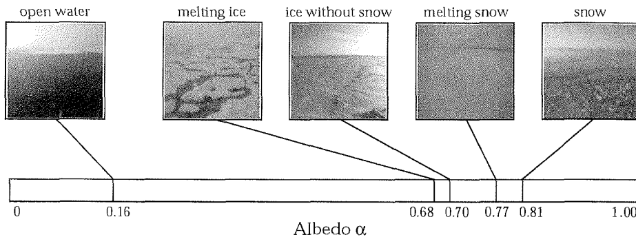
Figure 2.3: Values for different surface types in the Arctic Ocean as used in the numerical model. The sample images are taken from Haas and Lieser (2003).
