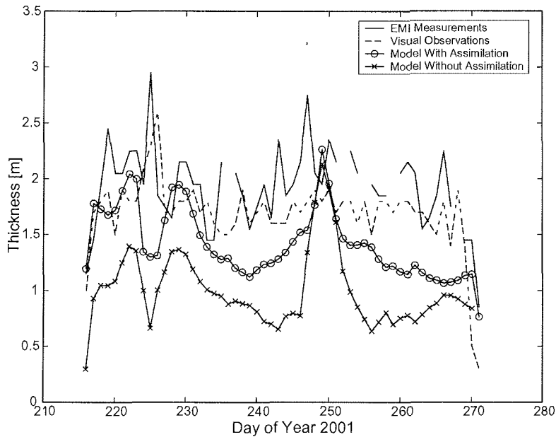
Figure 6.7: Comparison of the daily mean sea ice thickness estimates along the cruise track of RV POLARSTERN during the expedition ARKTIS XVII/2. The solid line shows measured EMI values, whereas the dashed line presents the visual observations. Lines with marks are model calculations with data assimilation (o) and without data assimilation (x). The ship entered the sea ice on day 217 (05 August 2001) and left it on day 271 (28 September 2001).
