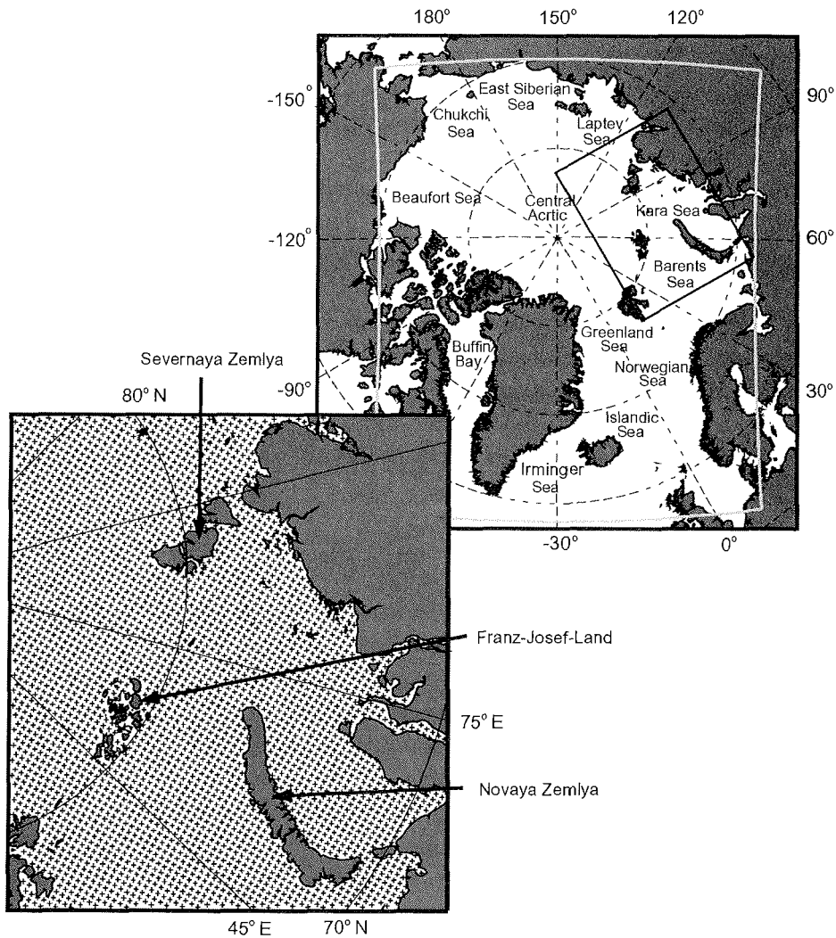
Figure 2.6: The model domain covers the complete Arctic Ocean, the Nordic Seas, and the northern North Atlantic and is indicated by the grey rectangle in the upper right part. The black rectangle indicates the location of the lower left panel, which gives an impression of the density of grid points in this recent model setup as an example for the Barents and Kara Seas.
