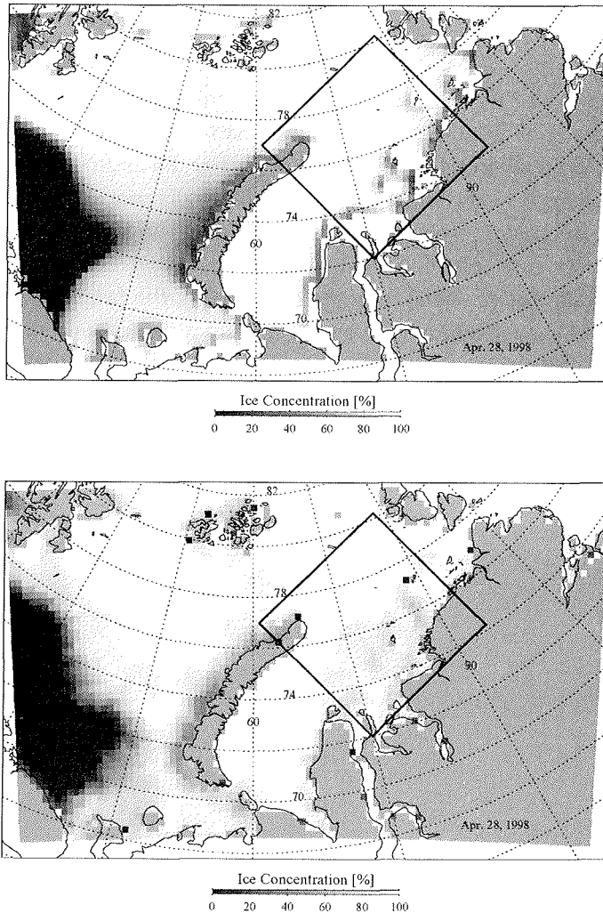
Figure 6.4: Result of a model forecast run for 28 April 1998 in the Kara Sea. The upper panel shows the calculated ice concentration. The lower panel shows the SSM/I data for comparison. The black rectangle indicates the location of the satellite image shown in Figure 6.3 provided by the Russian ice pilots.
