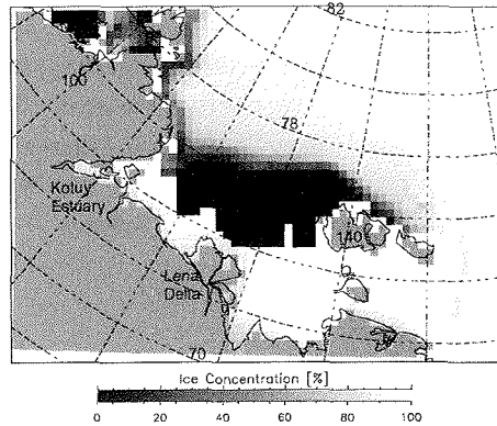
Figure 2.2: Model result of sea ice concentration for a simulation for 27 June 1995 showing the Laptev Sea region with fast ice and a polynya.
