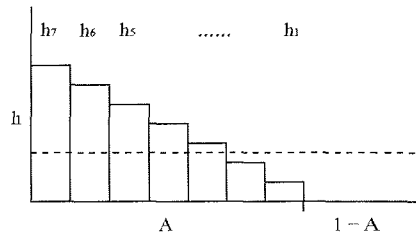
Figure 2.5: Ice volume distribution in seven ice classes for the calculation of the mean heat flux. The distribution is assumed to be uniform in the interval between 0 and 2h/A . The mean ice thickness (dashed line), calculated as h/A , is the reference for the relative ice thicknesses for all classes.
