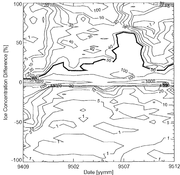
Figure 4.11: Monthly mean Greenland Sea sea ice concentration differences for the reference period as a contour plot of numbers of occurrence for the MOM oceanic and ECMWF atmospheric forcing combination (M+E setup).
