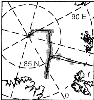
Figure 6.6: This figure shows the noon positions of R/V POLARSTERN cruise ARKTIS XVII/2 with respect to the grid-cells of the numerical model. The ship entered the Arctic Ocean from the Barents Sea, turned to the south-west (towards Greenland), turned back to north-east, made a transect to the geographical North Pole and took the same route back to the Barents Sea.
