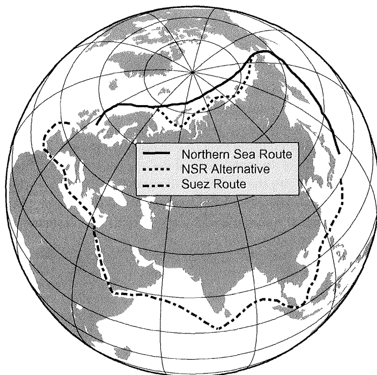
Figure 1.5: The Northern Sea Route connects northern Europe with South East Asia via the Arctic Ocean. This Figure shows an example of a track from the North Sea to Japan (approx. 6900 nautical miles). The solid line indicates a possible track in favourable ice conditions if the route along the Siberian Coast (dotted alternative) is impassable due to closed key locations (e.g. , Kara Gate or Vilkitsky Strait). The dash-dotted line shows the conventional track through the Mediterranean, the Gulf of Suez, and the Indian Ocean (approx. 11100 nautical miles).
