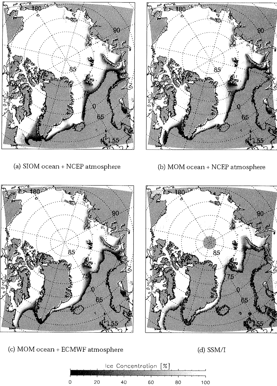
Figure 4.4: Same as Figure 4.2 but for February 1995 as an example of late winter conditions.
