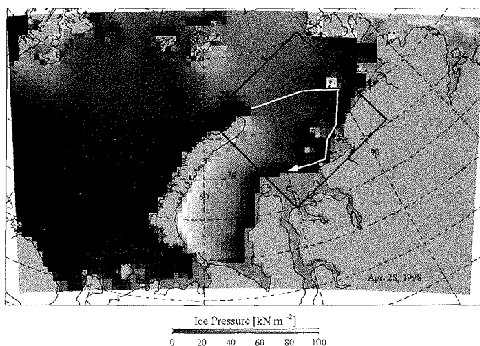
Figure 6.5: Horizontal ice pressure deduced from model results for 28 April 1998. The black rectangle indicates the location of the satellite image shown in Figure 6.3. The arrow shows the suggested Route No. 1 provided by the Russian ice pilots.
