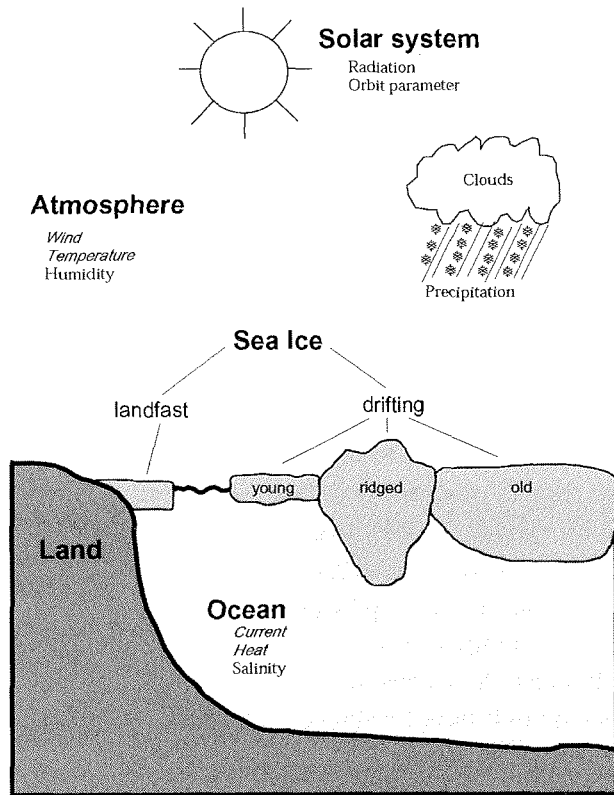
Figure 1.1: Sea ice in the climate system. Sea ice forms on the sea surface at high latitudes and thus modifies the interaction between the atmosphere and the ocean. Thermodynamic growth and decay are prescribed through the energy balance (including atmospheric and oceanic heat fluxes and heat conduction), whereas dynamic variables (e.g. drift velocities) can be determined from the momentum balance (including the effects of wind and ocean currents).
