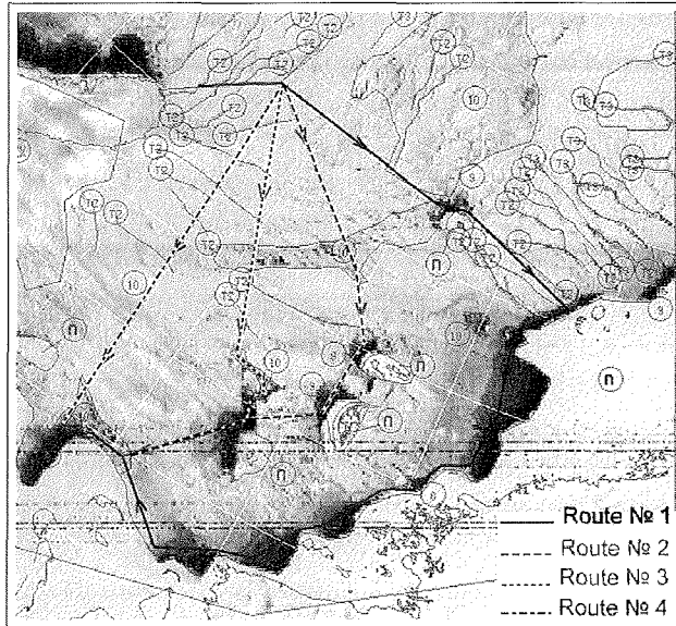
Figure 6.3: During ARCDEV four possible route alternatives from the northern tip of Novaya Zemlya to the Ob Bay were developed by AARI (Arctic and Antarctic Research Institute, Russia) ice pilots. The convoy followed Route No.1 making best use of the ice situation by going through leads and polynyas (image taken from http://arcdev.neste.com ). Data courtesy of AARI, image adapted.
