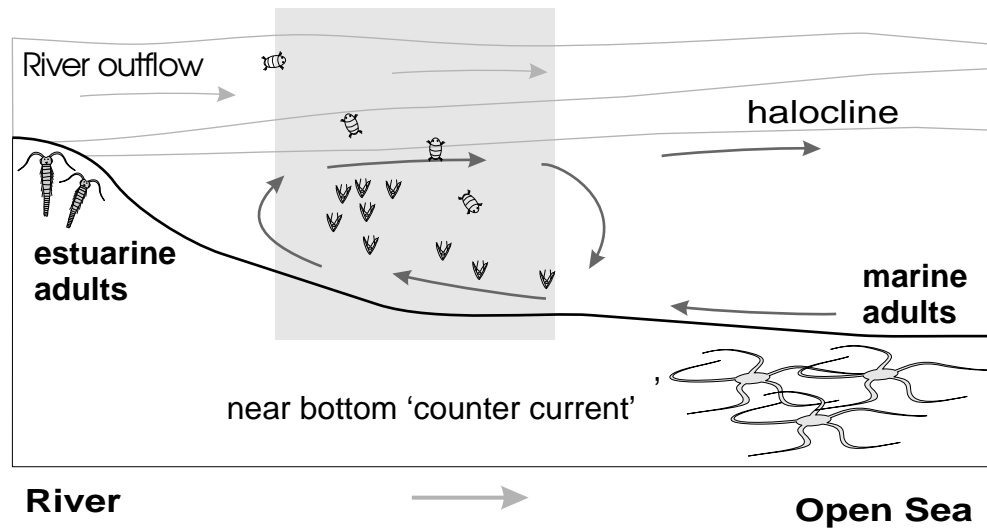
Figure 13: A near bottom counter current is established by strong river run off. The resulting hydrographic flow pattern concentrates larvae in the mixing zone
