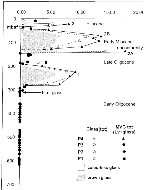
Fig. 2 - Diagram showing the proportion of fresh volcanic detritus in sand-grade samples from CRP-2/2A. Modal indices illustrated are total glass, proportion of brown and colourless glass, and total volcanic detritus (glass plus fresh volcanic lithic grains). All the glass present above 307 mbsf (metres below sea floor) is believed to be derived from the McMurdo Volcanic Group. Prominent volcanic periods are indicated by shading and labelled 1-3. P1-P4 refers to petrofacies 1-4 described in the text.
