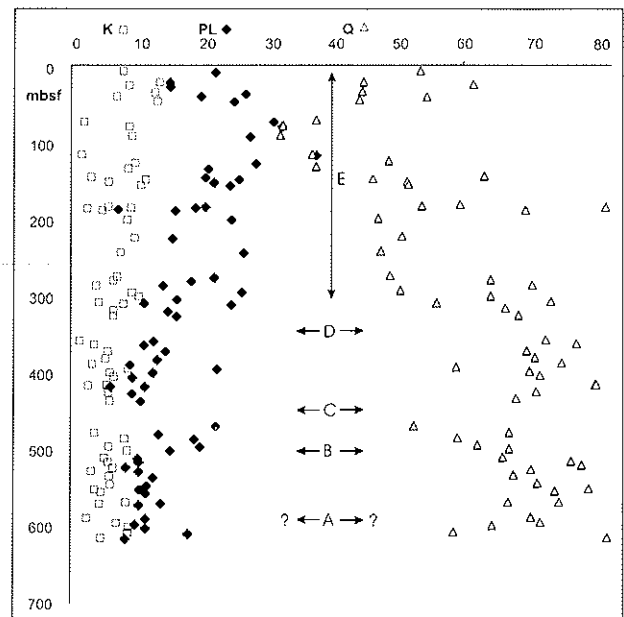
Fig. 1 - Down-core distribution of alkali feldspar (K), plagioclase (PL) and quartz (Q) in CRP-2/2A. Below 300 mbsf, the data for each mineral vary stepwise, and abrupt transitions occur between data "blocks" (indicated by boxes). Positions of the step-like transitions in the data are labelled A-D. Above c. 300 mbsf (metres below sea floor; labelled "E"), the modes are strongly affected by debris derived from coeval volcanism, which affects the absolute values of these indices and any transitions controlled by non-volcanic provenance variations are thus masked. Each box depicted includes most of the samples within selected depth intervals, to illustrate the major modal differences between adjacent depth intervals. Over each interval distinguished, plagioclase and alkali feldspar abundances vary sympathetically, whereas quartz variations are antithetic to the feldspars. By contrast, the prominent lack of a covariation between the feldspar types above 300 mbsf suggests two independent feldspar sources for that depositional period.
