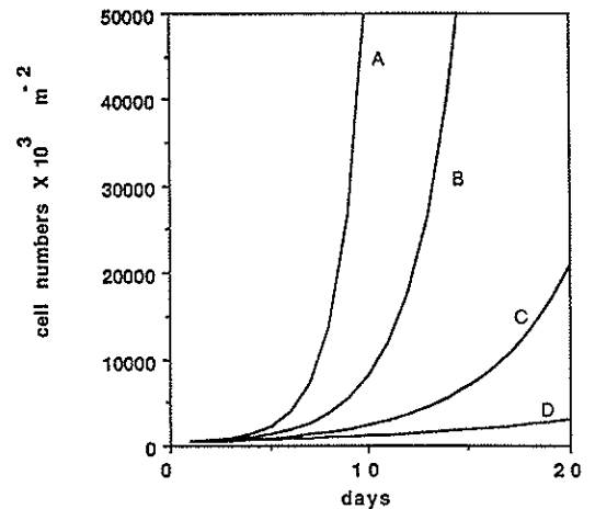
Fig. 2. Curves A-D represent population growth rates in a 50-m water column with mixing depths of 10, 20, 30, and 50 m (levels A, B, C, D from Fig. 1). Cell division rates explained in text. An initial seed stock of 10 cells liter -1 for the entire water column has been used.
