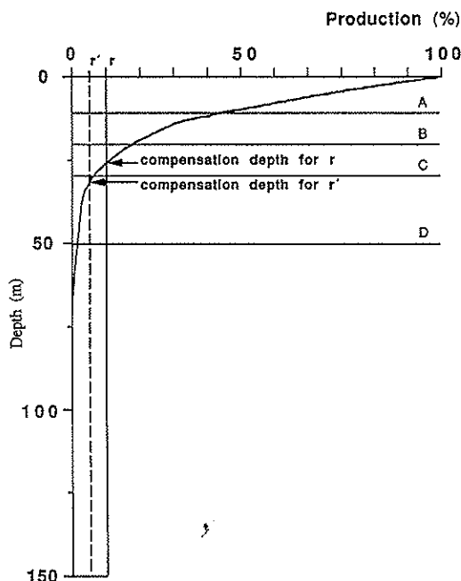
Fig. 1. Sverdrup's model in its modern rendition, where r and r' represent phytoplankton respiration at 10 and 5% of P_{max} ( =100\% ). Whereas compensation depth increases by only 6 m (by a factor of 0.23) from r to r' , critical depth doubles from 150 to 300 m (latter not shown). A, B, C, and D levels correspond to Fig. 2.
