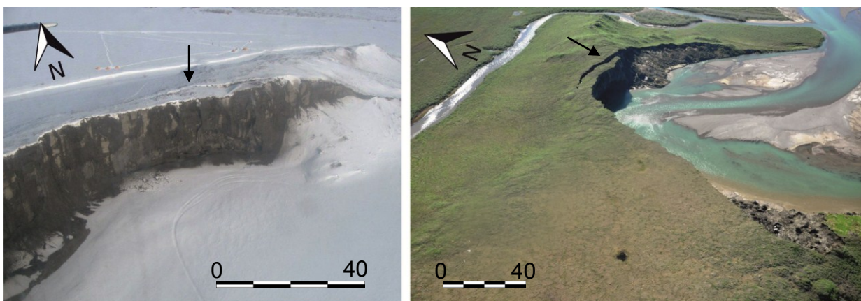
Fig. 1.5: Aerial view on Itkillik River exposure during spring (left) and summer (right) 2012. The arrows on both pictures mark a crack at the eastern part of the bluff. Scale in meter. Pictures from K. Bjella (left, May 2012) and A. Breen (right, June 2012)
