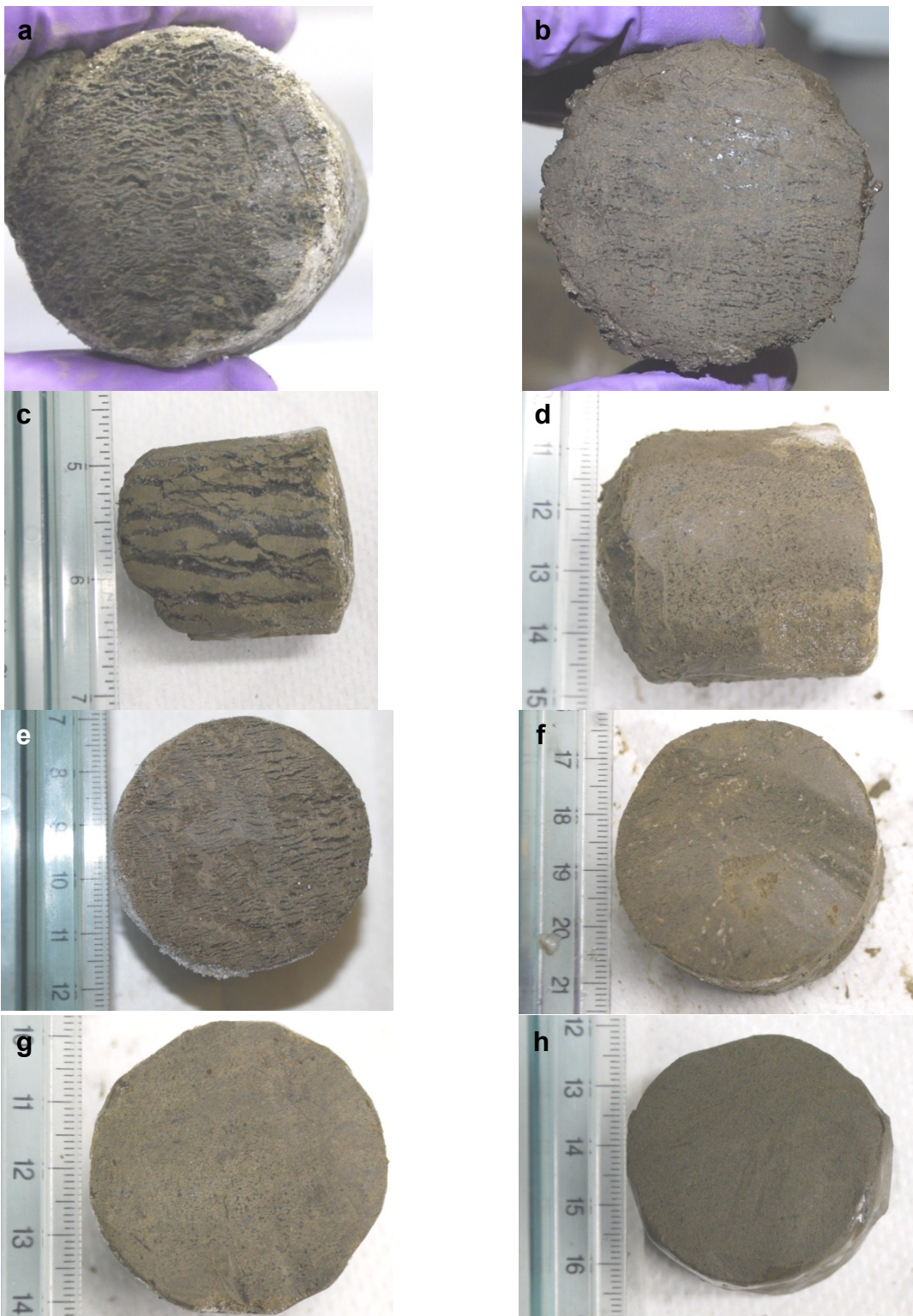
Fig. 1.14: Pictures of the sediment samples and their cryostructure; a) It-1 (2.1 m b.s.l.), micro-braided to micro-ataxitic cryostructure; b) Itk-B-02 (27.5 m b.s.l.), micro-lenticular to micro-braided cryostructure; c) Itk-D-03 (24.8 m b.s.l.), braided to ataxitic (suspended) cryostructure; d) Itk-E-03 (9.2 m b.s.l.), latent micro-lenticular cryostructure to porous visible, e) Itk-F-02 (20.2 m b.s.l.), latent micro-lenticular; f) Itk-G-02 (15.9 m b.s.l.), micro-lenticular to micro-braided cryostructure; g) Itk-I-02 (10.6 m b.s.l.), micro-porphyrritic cryostructure; h) Itk-J-02 (28.9 m b.s.l.), structureless cryostructure. All pictures by D. Fortier (May 2012)
