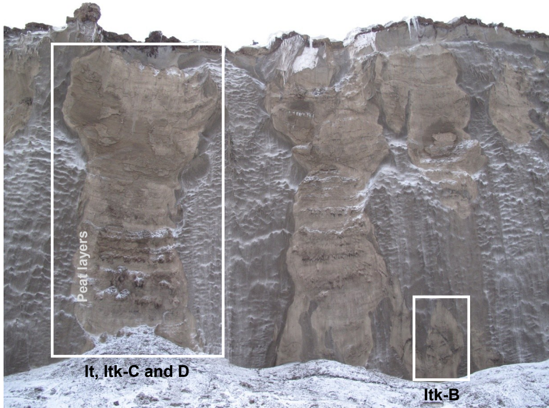
Fig. 1.17: Overview of the major profile. The sampling areas are identified by white boxes. A schematic of this profile is shown in Fig. 1.16. Picture by J. Strauss (May 2012).
