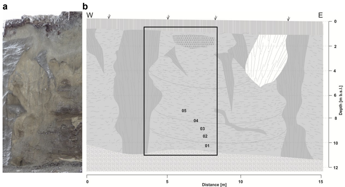
Fig. 1.21: a) Picture and b) schematic of sub-profile Itk-E; the box in b marks the extent of the photograph in a. The sampled baidzharakh Fig. 1.19 is below this profile. Picture a by J. Strauss (May 2012).
