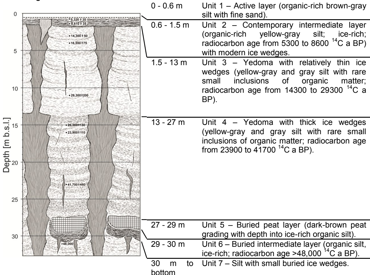
Fig. 1.23: Cryostratigraphical units of the Itkillik Yedoma (ice wedges width not to scale) and radiocarbon age of deposits, 14 C a BP, modified from Kanevskiy et al. [2011].
