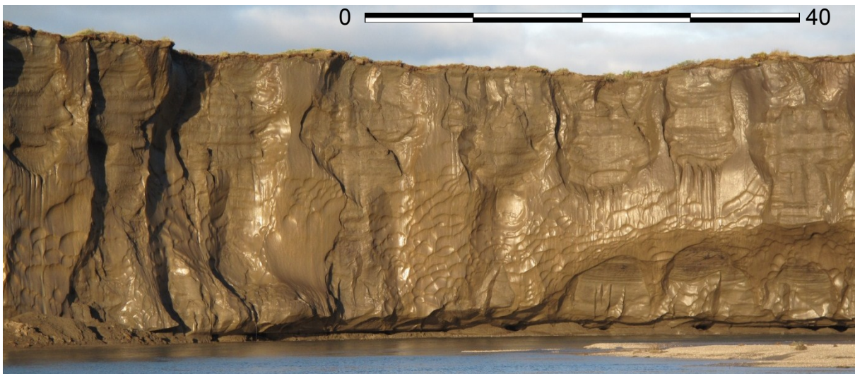
Fig. 1.6: Itkillik exposure during summer 2011. Scale in meter. Picture by M. Kanevskiy (August 2011)
