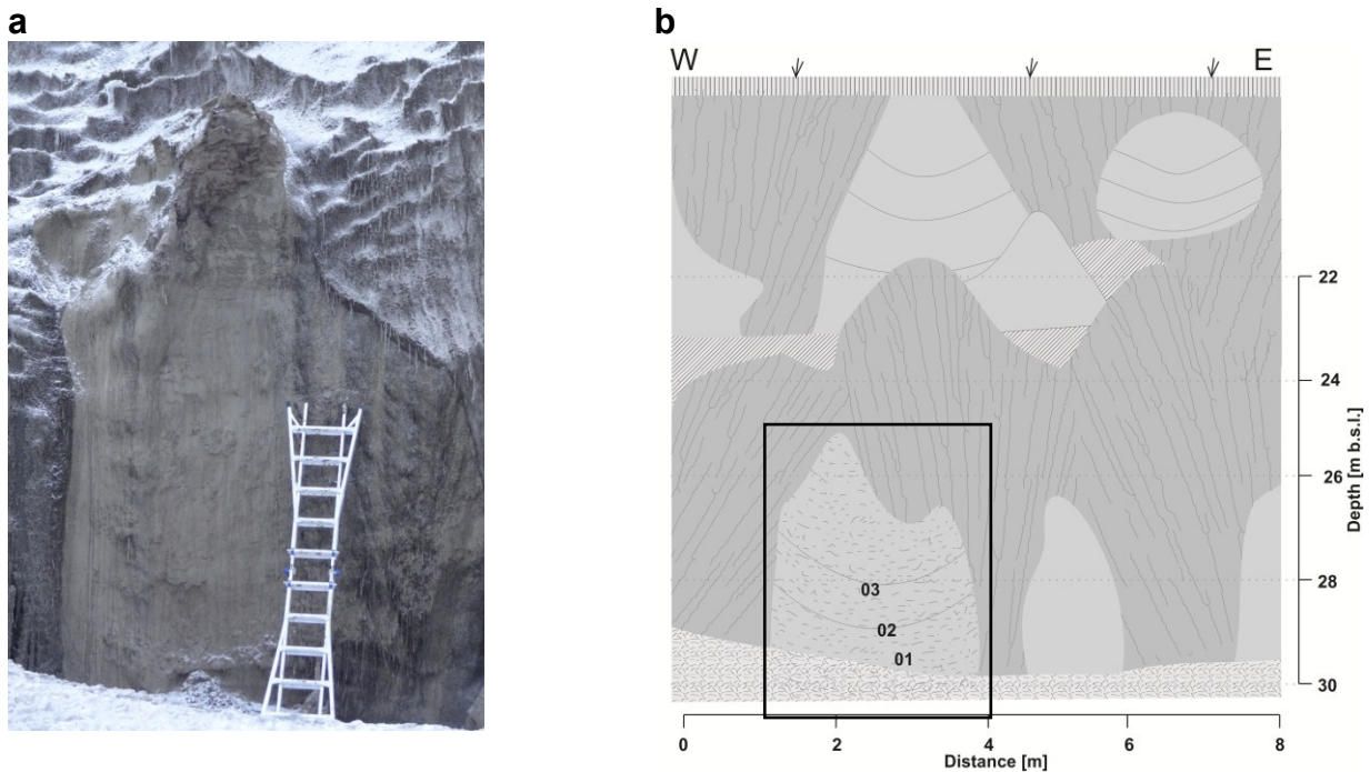
Fig. 1.15: a) Picture and b) schematic of sub-profile Itk-J; the box in b marks the extent of the photograph a. The scale in b is based on the front schematic and is not usable for the background. Picture by J. Strauss (May 2012).
