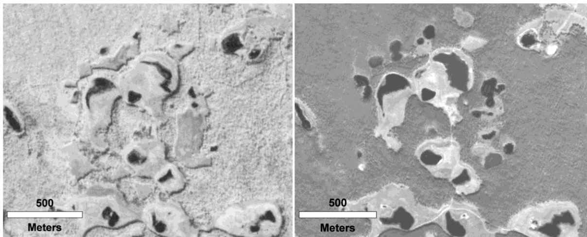
Fig. 2.3: Landscape evolution at the Yukechi study site. Several thermokarst lakes in the north and the southeast of the Yukechi alas have been developed since 1967 (left), in particular in areas which were used agriculturally before (Compare e.g. Point #8, #9, and #10 in Fig. 2.2A). Left: Close up of a Corona image, September 20, 1967. Right: AlosPrism close up, August 13, 2010.
