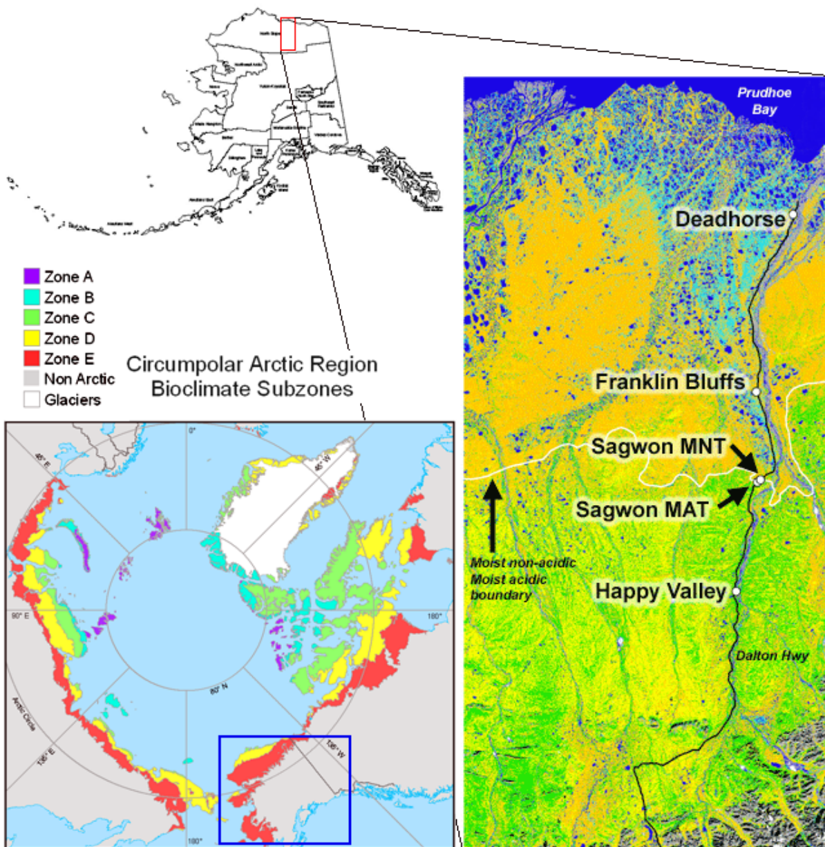
Fig. 3.5: Location of the study sites. The down left box shows the CAVM with the five bioclimate subzones. Note the blue rectangle which marks Alaska. The right box shows the four Low Arctic study areas. Images by AGC and Walker et al. [2005].
