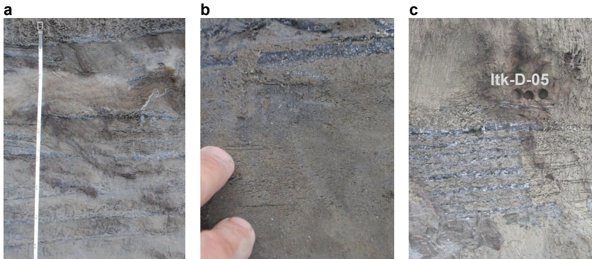
Fig. 1.18: Cryostructures close to profile Itk-C and Itk-D; picture of a) of ice bands >3 cm and b) ice
