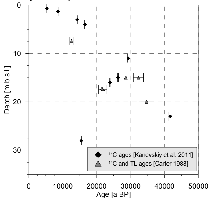
Fig. 1.24: Age-depth relationship of the Itkillik Yedoma, based on radiocarbon and thermoluminescence analyses
