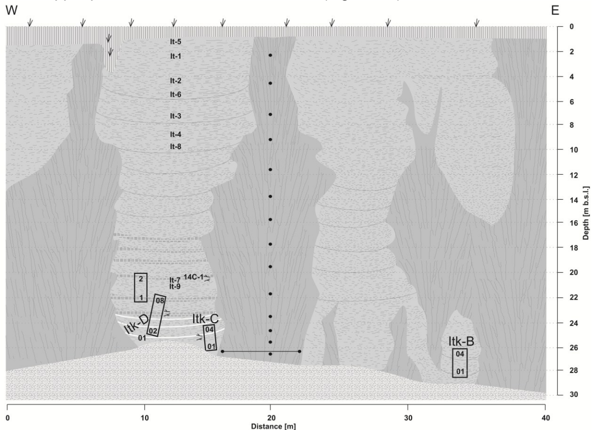
Fig. 1.16: schematic of the major profile with position of the sub-profiles (Itk-B, Itk-C, Itk-D and It) and sample sites). A picture of this sequence is shown in Fig. 1.17.
