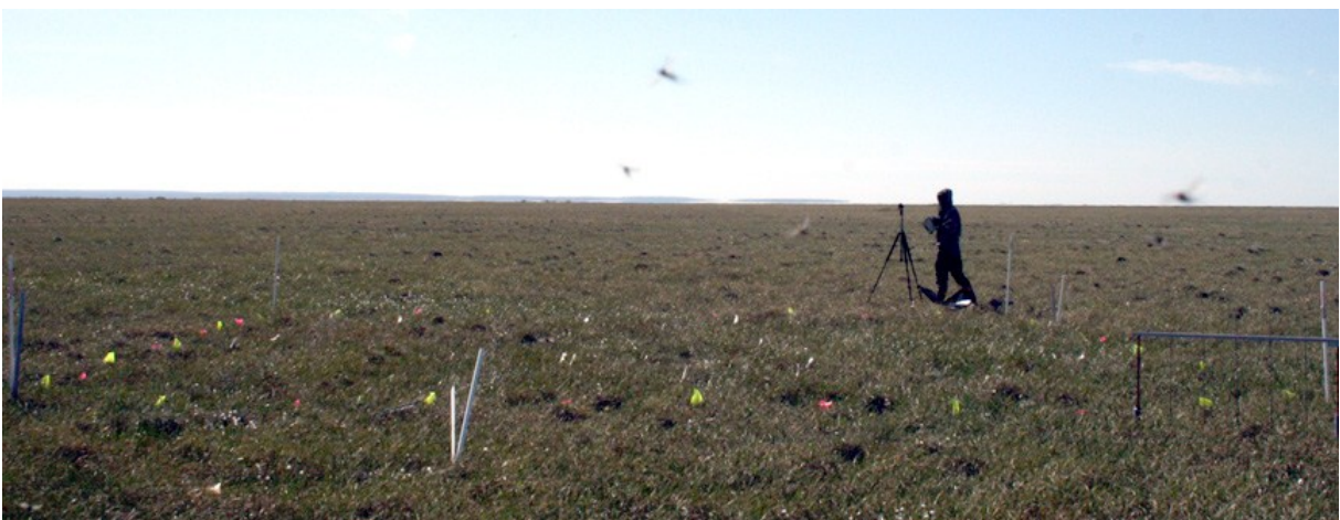
Fig. 3.14: The Deadhorse zonal (DH_zonal) study site. Life form description: moist graminoid, sedge, prostate dwarf-shrub tundra. Picture by M. Buchhorn.
