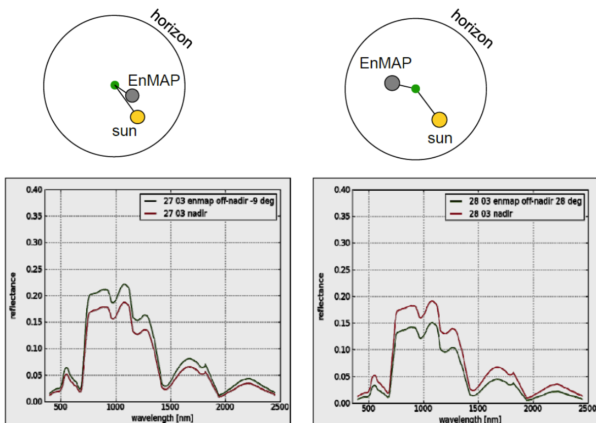
Fig. 3.18: Theoretical behaviour of the BRDF effect. Left: Higher reflectance values of the sensor looking in the backward scattering direction (green curve) than looking nadir (red curve). Right: Lower reflectance values of the sensor looking in the forward scattering direction (green curve) than looking nadir (red curve).
