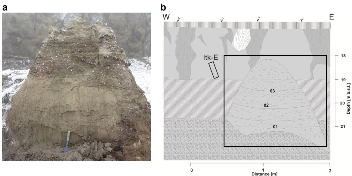
Fig. 1.19: a) Picture and b) schematic of the baidzharakh containing sub-profile Itk-F; figure b) also shows the relative position of sub-profile Itk-F to sub-profile Itk-E in the background of the baidzharakh. The scale in b is based on the baidzharakh; for the background, like the Itk-E profile, the scale of Fig. 1.21 has to be used. The box in b marks the extent of the photograph in a. Picture by J. Strauss (May 2012).
