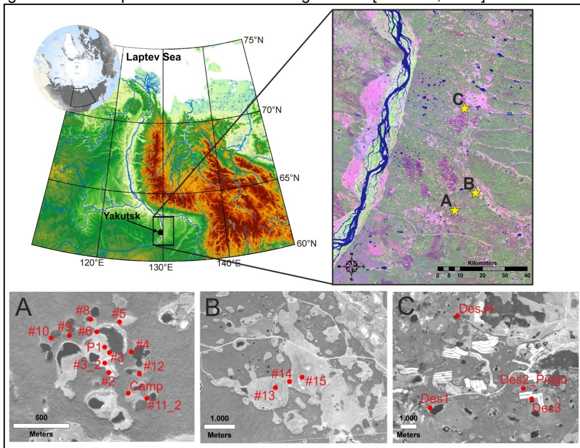
Fig. 2.2: Study region in Eastern Siberia within the zone of continuous permafrost and thermokarst key sites in the Lena-Aldan-Amga region explored during the journey. The labeled red points indicate GPS-located sites of detailed surface description and preliminary sedimentological surveys. A: Yukechi study site on the Abalakh terrace. B: Khara Bulgunakh alas on the Tyungyulyu terrace. C: Investigated sites around the Ulakhan Sekhan study site on the Tyungyulyu terrace. Upper left: Digital elevation model of East Siberia compiled by data of the ESA DUE Permafrost project; http://www.ipf.tuwien.ac.at/permafrost/ . Upper right: Close up of a Landsat-TM5 image, August 12, 2002; RGB 5-4-3. Below: AlosPrism close ups, August 13, 2010.
