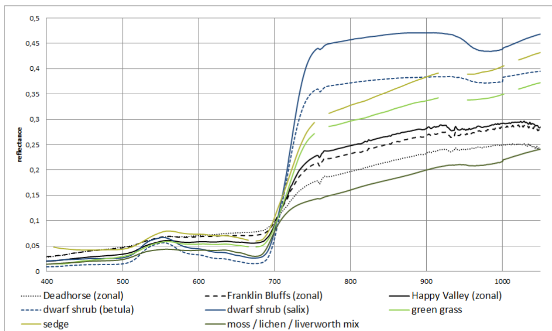
Fig. 3.16: Comparison of spectral signatures of typical low-growing Low Arctic vegetation communities and spectral signatures of pure plant species.
