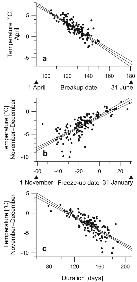
Fig. 3 Calibration of proxy variables by means of linear errors-in-variables regression; best fit with 95% confidence band ( solid lines ), data points ( dots ). a April temperature versus breakup date, b November–December temperature versus freeze-up date, c November–December temperature versus duration of ice cover
