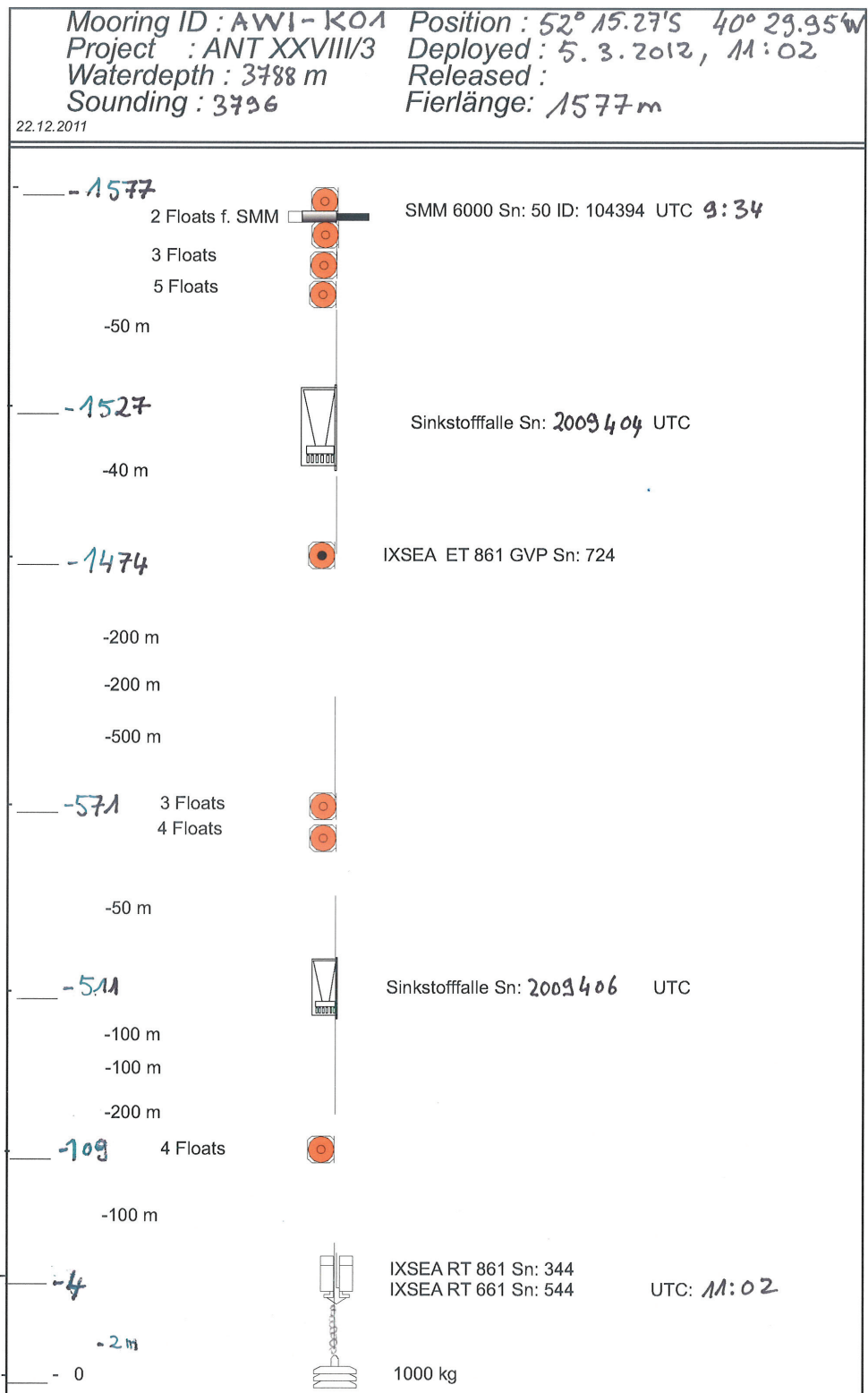
Fig. 14.3: Long-term (1 year) mooring deployed in the Georgia Basin
