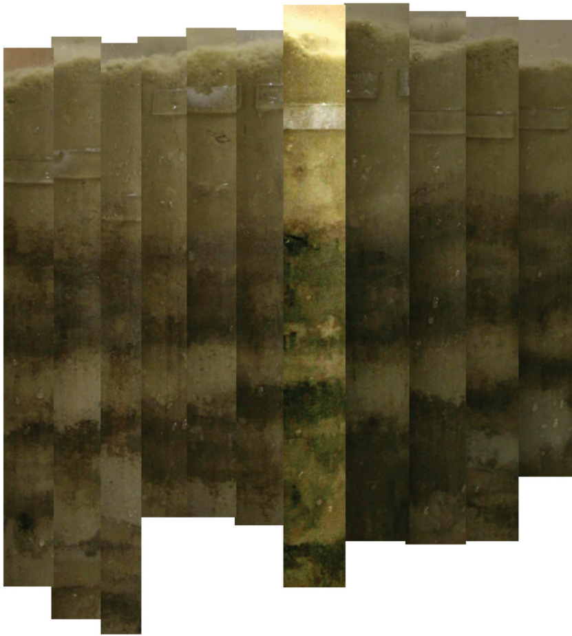
Fig. 16.1: Composed photography of all the cores collected on one MUC at station PS79/86. The layering was very characteristic of this station. The sediment core was well oxygenated.
