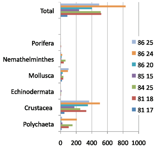
Fig. 19.3: Abundance of macrofaunal taxa in the EBS catches (raw data)
