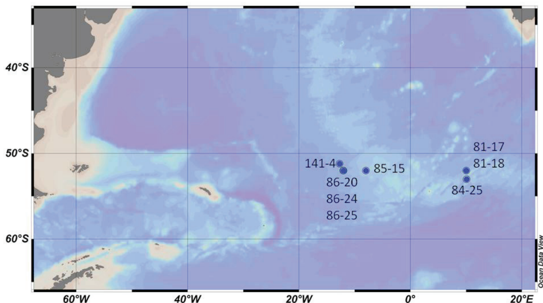
Fig. 19.2: SYSTCO II stations sampled by means of the epibenthic sledge
