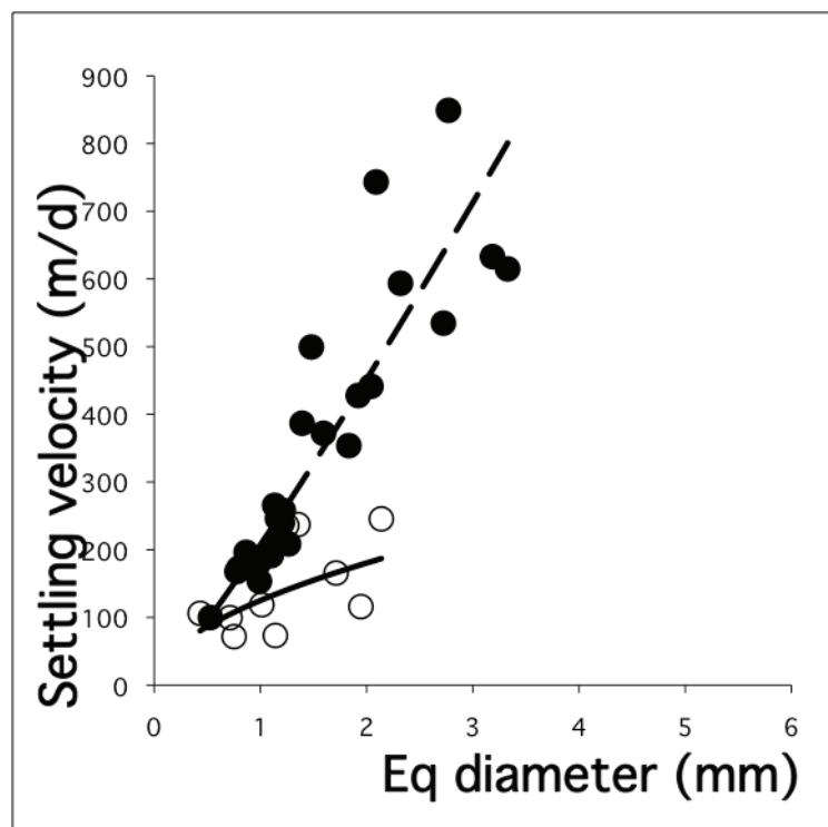
Fig. 14.2: Sinking speed of salp fecal pellets plotted over the equivalent spherical diameter (ESD). Two different pellet types were distinguished, solid freshly produced pellets (closed circles) and loose and possible partly degraded pellets (open circles). The regression for the solid pellets is: sinking speed = 207 * ESD^{1.12} , R^2 = 0.88 and for the loose pellet it is: sinking speed = 125 * ESD^{0.53} , R^2 = 0.31 .
