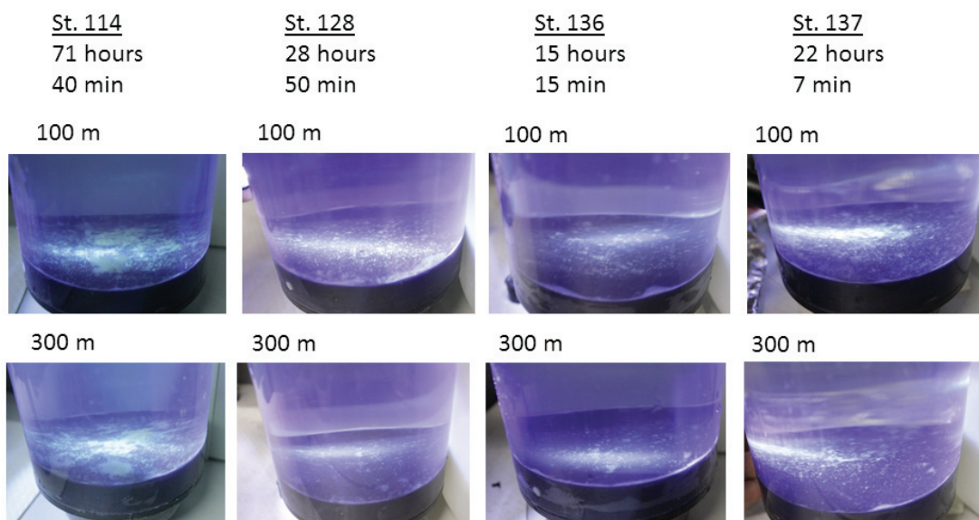
Fig. 14.1: Photographs of sediment trap cylinders with collected material from 100 and 300 m depths at four different stations. Station number, duration and depth of trap cylinder are indicated for each deployment above the photographs.
