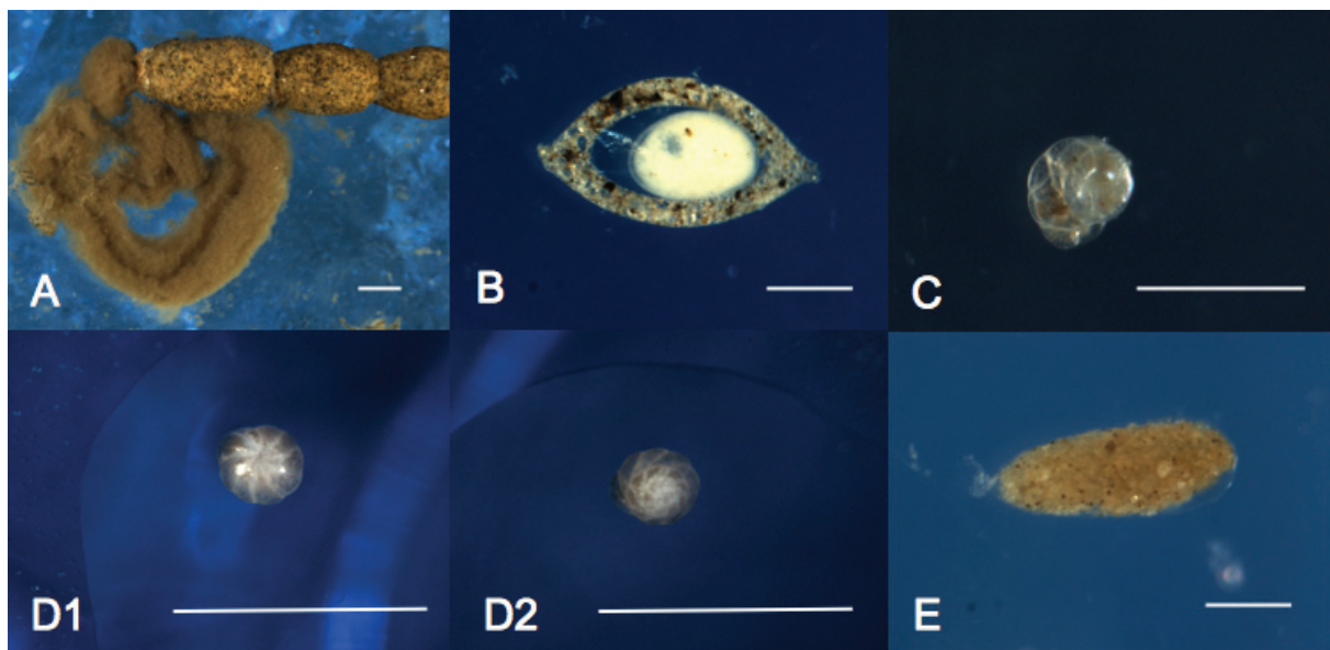
Fig. 17.2: Representative picked species. A „ Botellina “, B Vanhoeffenella , C Robertiniidae , D1 and D2 Epistominella apical and umbilical sides, E Gromiida . Scale bars are 250 micrometers long.
