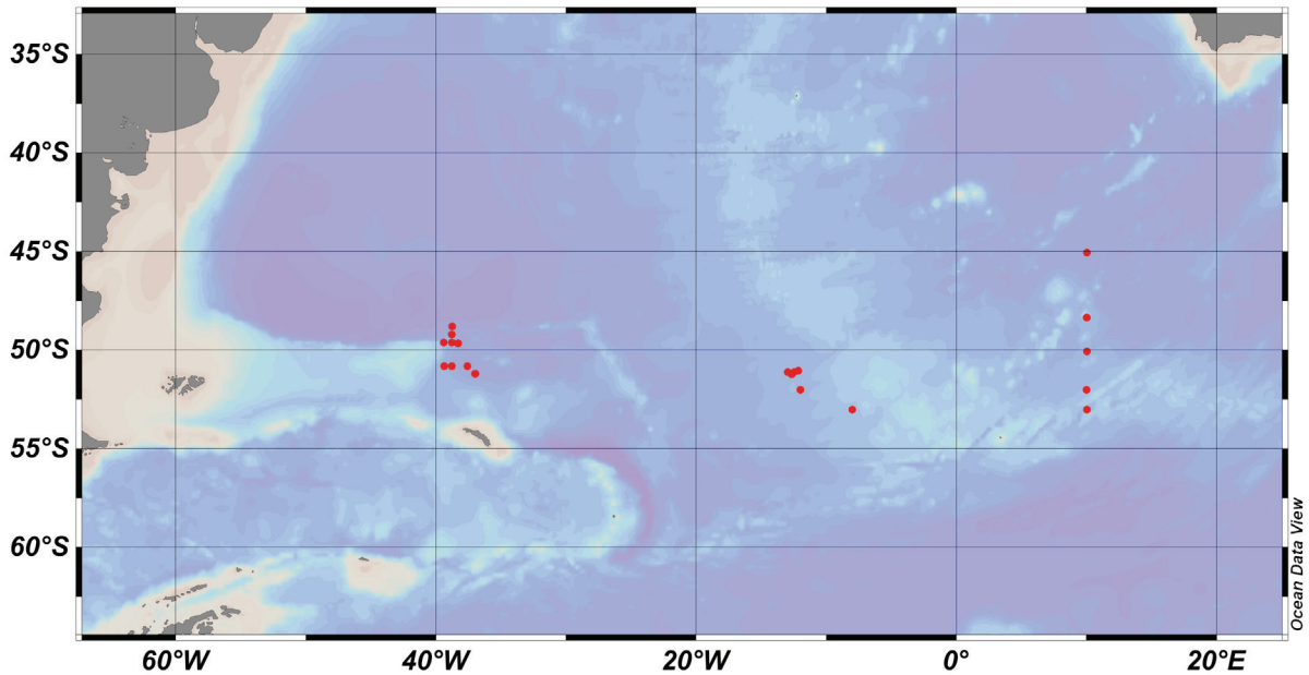
Fig. 6.1: Map of all sampled stations during the cruise track. In total, 26 CTD stations were sampled: PS79/60-5, 70-3, 73-2, 75-9, 81-11, 84-7, 85-3, 86-2, 91-5, 114-9, 128-10, 136-8, 137-7, 138-2, 139-3, 140-12, 147-1, 149-1, 155-1, 160-1, 165-5, 168-1, 169-1, 170-1, 174-9, 175-1.
