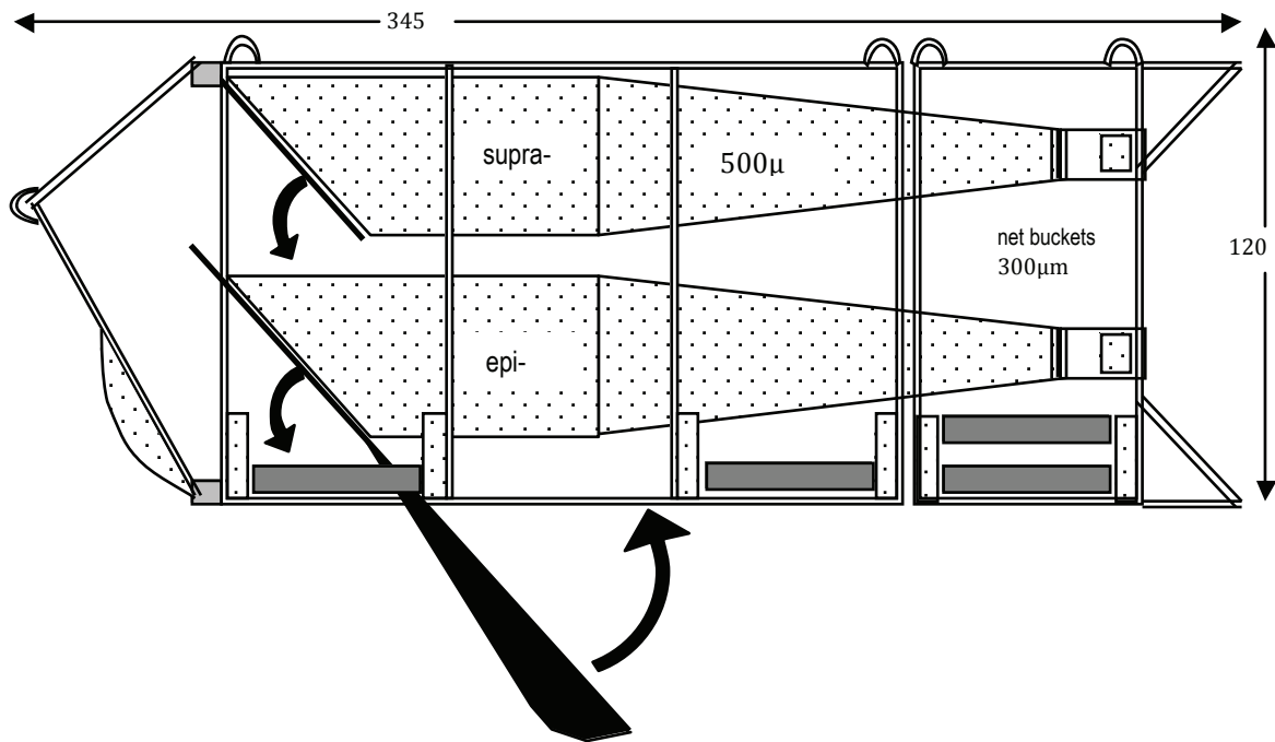
Fig. 19.1: Schematic illustration of the epibenthic sledge (Nils Brenke, DZMB)
