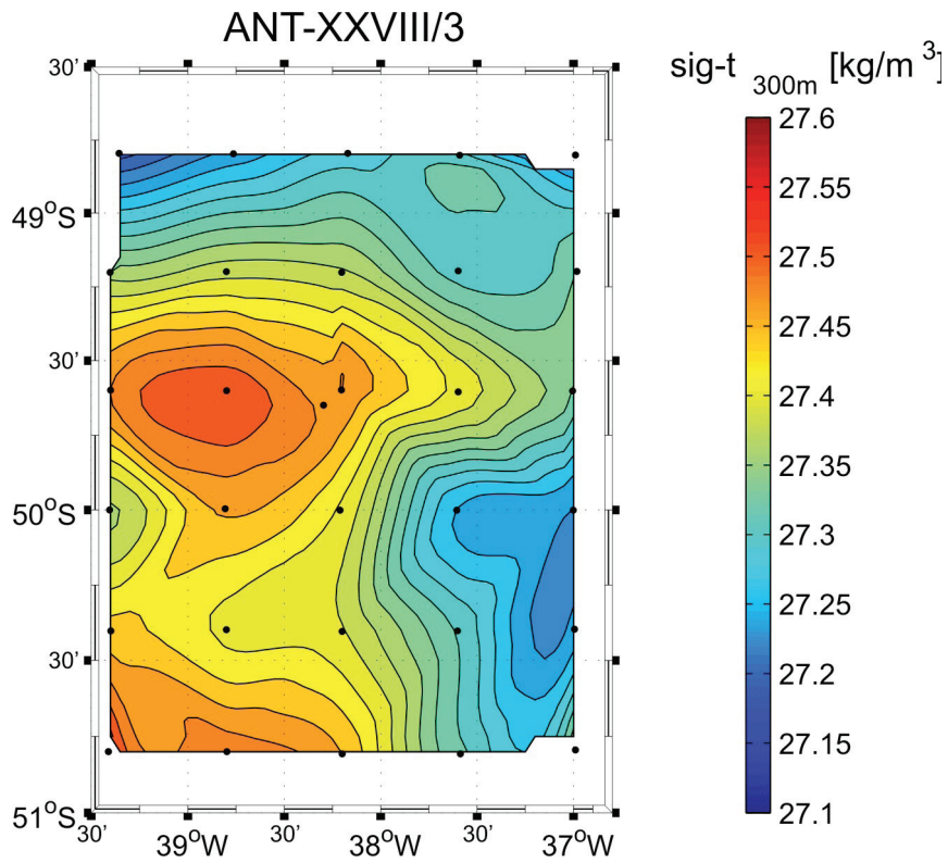
Fig. 3.6.1: Horizontal distribution of density \sigma_t at 300 m depth in the station grid north of South Georgia. The density contours also imply the geostrophic flow field, with streamlines running parallel to the density contours and the flow direction oriented in a way that the light water is located to the left. The flow speeds measured by the VM-ADCP (Section 3.3) in the northwest corner of the mapped area exceeded 100 \text{ cm s}^{-1} .
