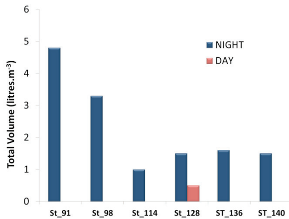
Fig. 13.3 Total volume of macrozooplankton collected at the eddy core of between 3 and 16 February
