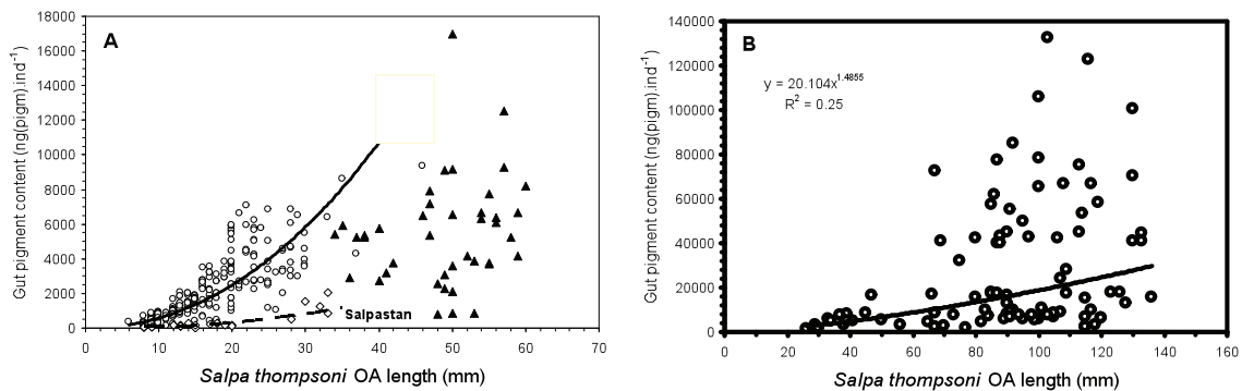
Fig. 12.3. Gut pigment content of Salpa thompsoni aggregates (A) and solitaries (B) during ANT-XXVIII/3. A: open diamonds – aggregates at Salpastaan; open circles – aggregates on any other station (10°E, 12°W and 37°W); solid triangles – aggregates classified as males.
