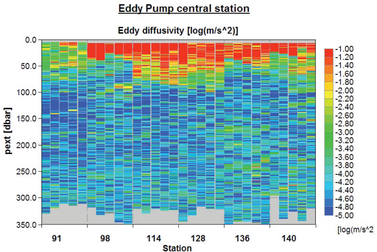
Fig. 5.1.2: Vertical distribution of the vertical diffusivity preliminarily derived from the MSS measurements at the indicated stations
