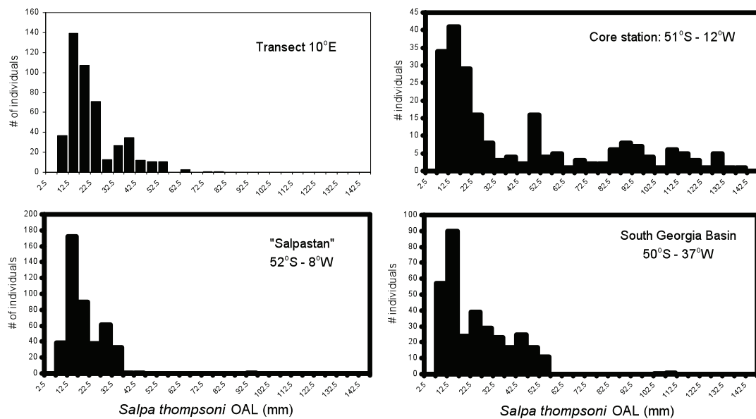
Fig. 12.1: Size frequency distribution of Salpa thompsoni populations in four main sampling areas
