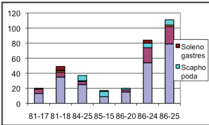
Fig. 27.1: Comparison in abundance of molluscan taxa between the different EBS stations in the first two regimes.
