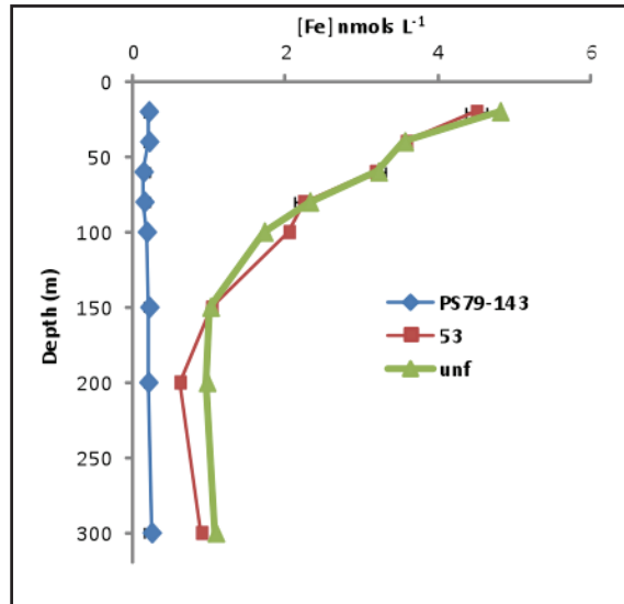
Fig. 7.3: Dissolved, > 53 mm and leachable particulate iron at station PS79/143 corresponding to the NE edge of the South Georgia shelf
