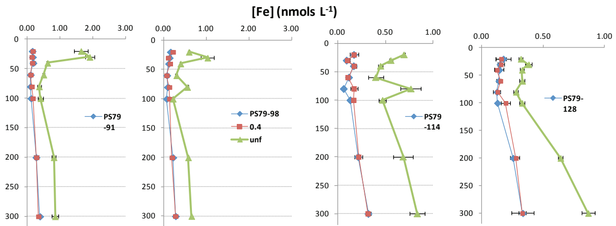
Fig. 7.2: Iron concentrations obtained in unfiltered, 0.2 mm filtered and 0.4 mm filtered samples form stations PS79/91 and 98. Iron concentrations in the fractions unfiltered, 0.2 mm filtered and 3 mm filtered samples from stations PS79/114 and 128.
