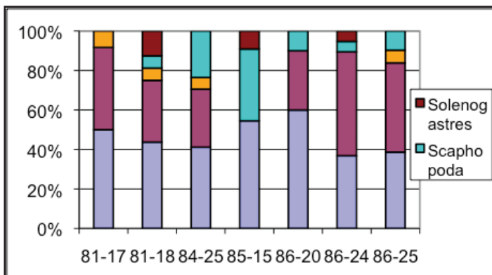
Fig. 27.2: Percentage of molluscan morphospecies from the different EBS stations in the first two regimes.
