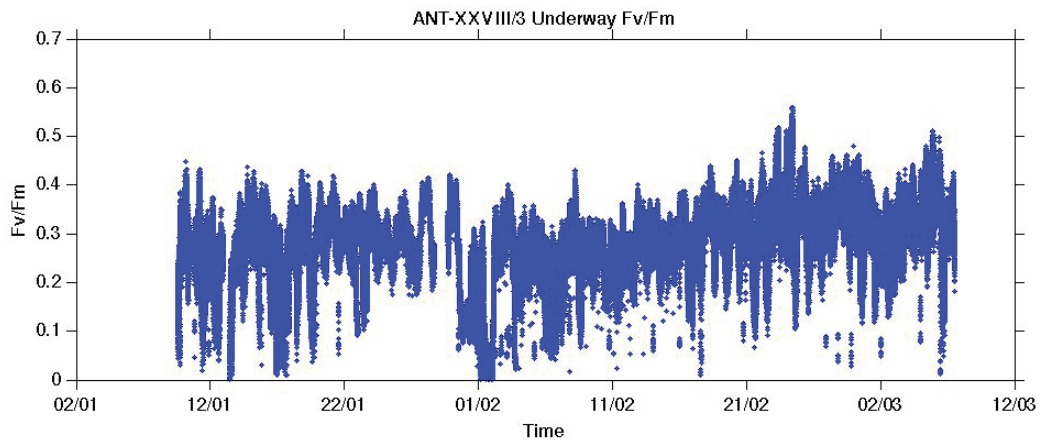
Fig. 10.1: Surface measurements of maximum photochemical efficiency of photosystem II (Fv/Fm) measured during the ANT-XXVIII/3 cruise on board Polarstern
