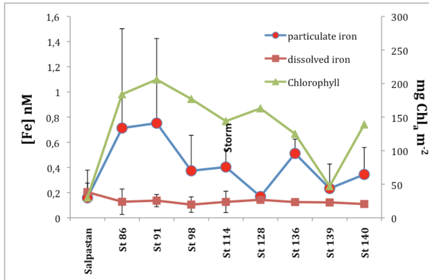
Fig. 7.1: Averaged dissolved and leachable particulate iron concentrations and chlorophyll concentrations integrated down to 120 m in the core stations. Station PS79/85 (Salpasthan) is added to study the effect of very low chlorophyll concentrations.
