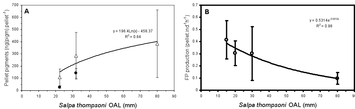
Fig. 12.4: Fecal pellet pigment content (A) and production (B) of Salpa thompsoni during ANT-XXVIII/3
