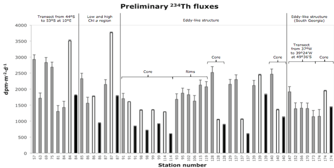
Fig. 1: Preliminary ^{234}\text{Th} fluxes derived from the water column at 100 m (grey columns) and fluxes obtained from the sediment traps at 100 or 120 m (white columns) and at 300 or 320 m (black columns), at all the sampled stations.
