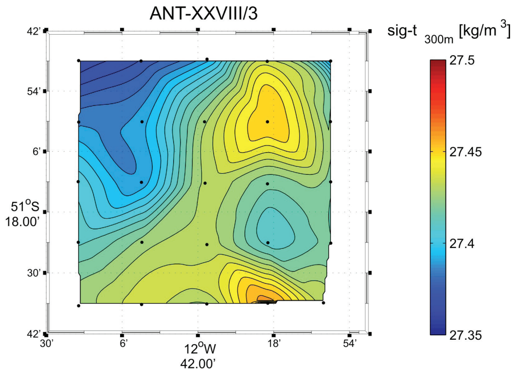
Fig. 3.1.2: Horizontal distribution of density \sigma_t at 300 m depth in the Eddy1 grid, based on CTD stations 98, 101 – 112 and 115 – 126 for synopticity reasons. The density contours also imply the geostrophic flow field, with streamlines running parallel to the density contours and the flow direction oriented in a way that the light water is located to the left (southern hemisphere). The flow speeds measured by the VM-ADCP (Section o.3) in the mapped area however were rather low and hardly exceeded 30 \text{ cm s}^{-1} .
