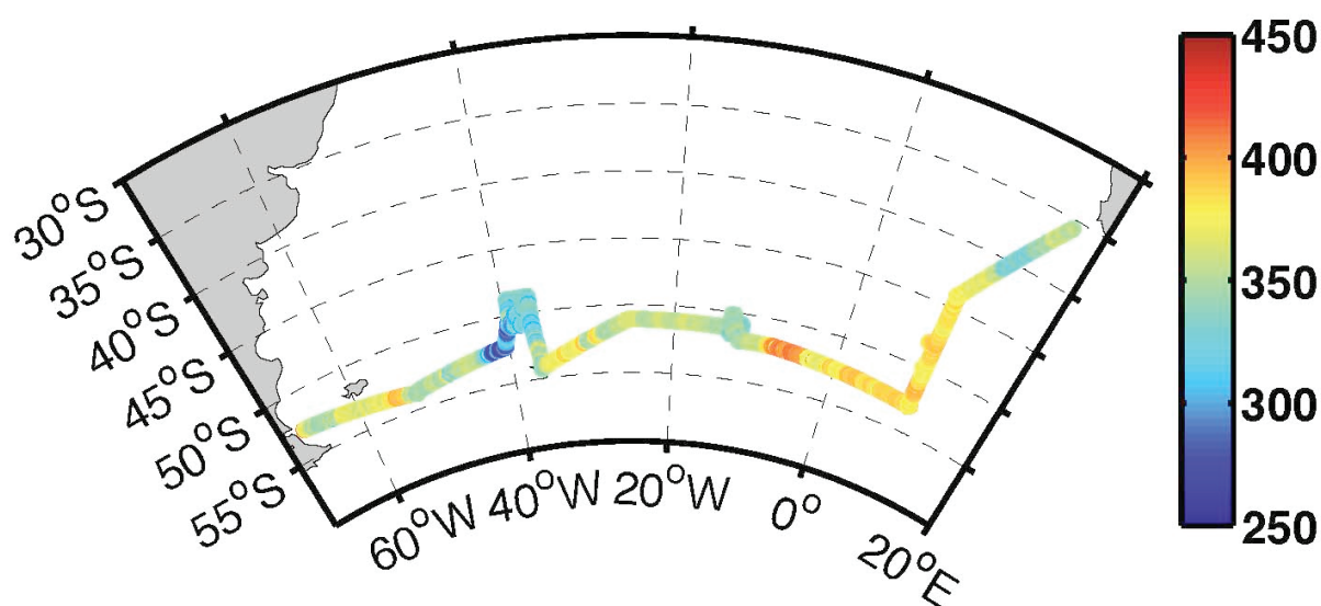
Fig. 5.1.1: Sea surface CO 2 (parts per million, ppm) along the ANT-XXVIII/3 cruise track
