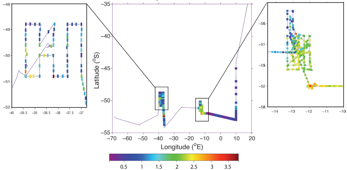
Fig. 11.1: Surface (8-10 m depth) Chl a concentrations in \mu\text{g L}^{-1} during ANT-XXVIII/3 (middle panel). Left and right panel illustrate the two main study areas visited during the cruise.
