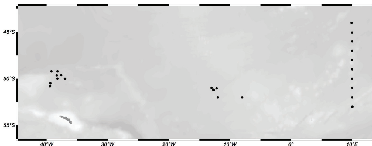
Fig. 13.1. Location of RMT sampling stations during ANT-XXVIII/3
