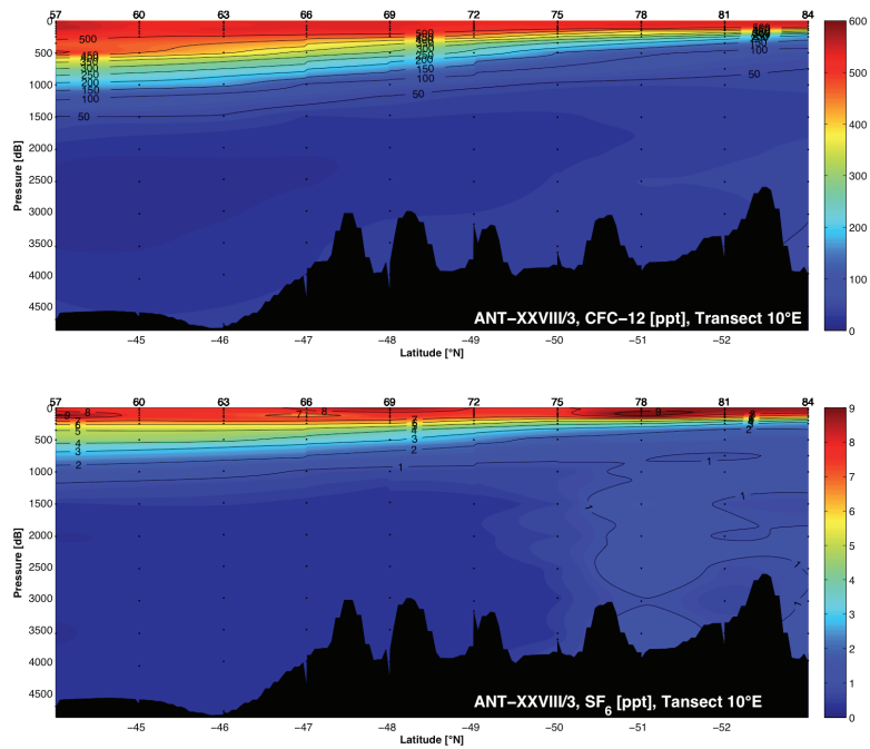
Fig. 5.4.1: Tracer concentrations along the 10°E transect
