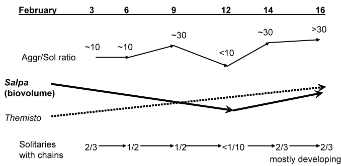
Fig. 12.2: Summary of salp biology at core station (51°S – 12°W) during February 3-16, 2012
