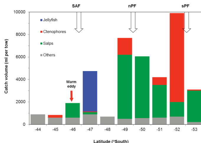
Fig. 13.2 Macrozooplankton community composition in RMT8 samples collected from Zone 1, a transect along 10 E. SAF - Sub-Antarctic Front; nPF and sPF - north and south Polar Front
