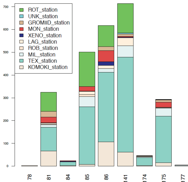
Fig. 17.1: Picked specimens of foraminiferans and related taxa for all stations. ROT: Rotaliids, UNK: not identifiable on board, GROMIID: Gromiids, MON: Monothalamiids, XENO, Xenophyophoreans, LAG: Lagenidae, ROB: Robertinidae, MIL: Miliolidae, TEX: Textulariids, KOMOKI: Komokiaceae.
