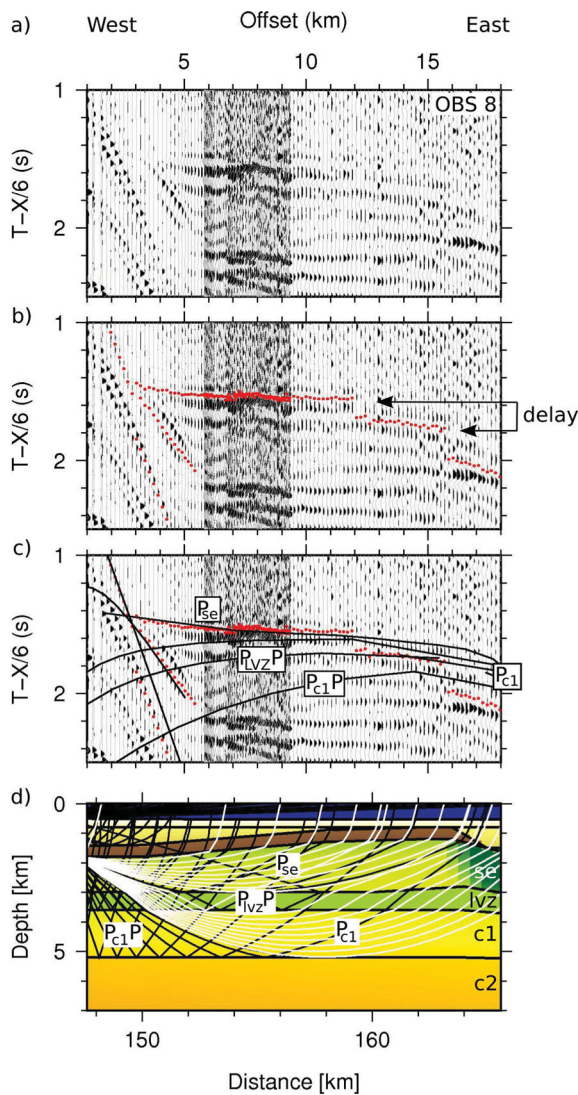
Figure 6. (a) Cutout of the seismic section of OBS 8, displayed with a reduction velocity of 6 km s -1 . (b) The same seismic section with picks in red. (c) The same seismic section with picks in red and calculated traveltimes in black. (d) P -wave velocity model with ray paths; black rays indicate reflected phases, white rays refracted phases; model layers are annotated.
