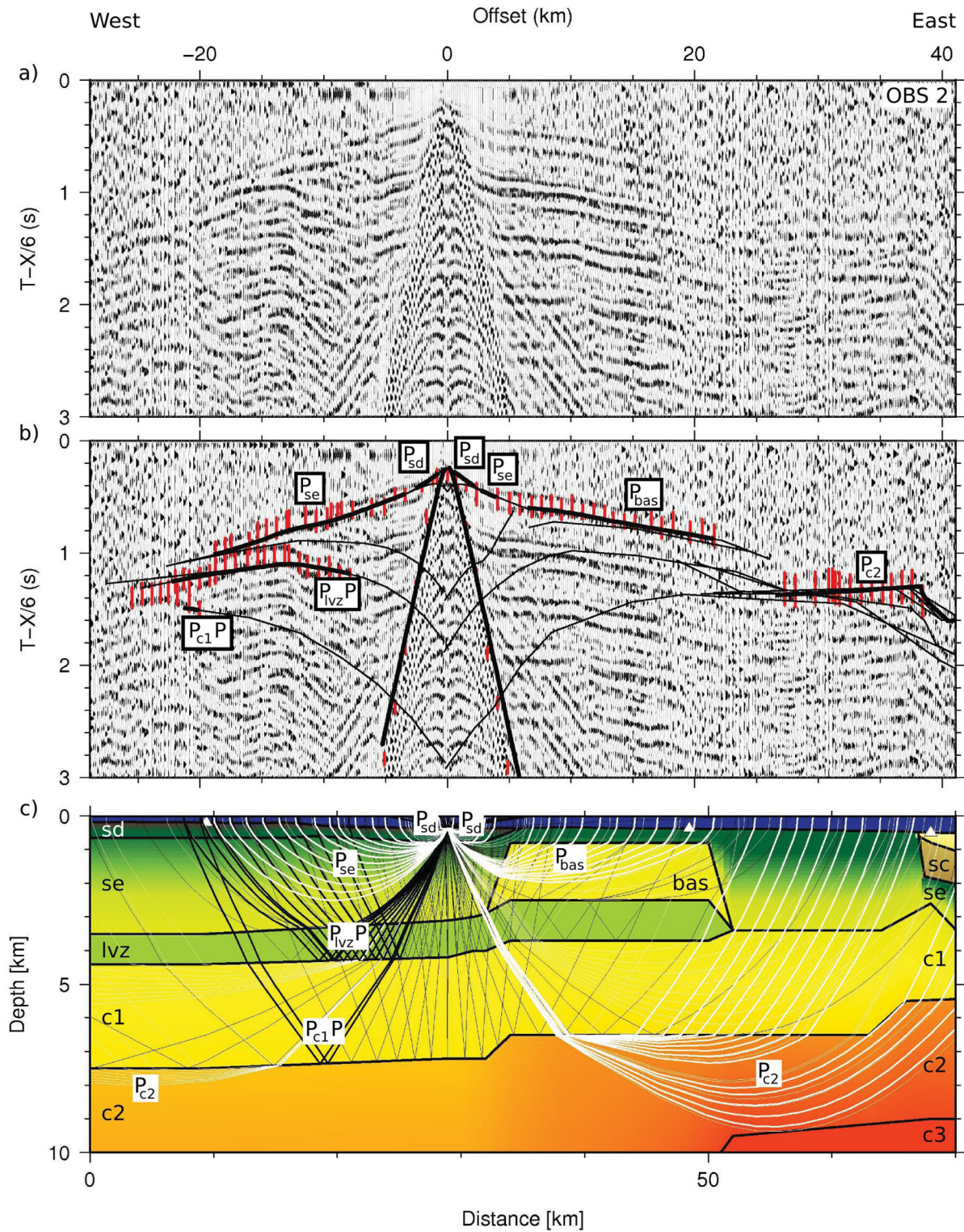
Figure 5. (a) Seismic section of OBS 2, displayed with a reduction velocity of 6 \text{ km s}^{-1} . (b) The same seismic section with picks in red; the pick length corresponds to the assigned pick uncertainty; calculated traveltimes are displayed in black with thick black lines corresponding to the picks. (c) P -wave velocity model with ray paths. Model layers are annotated; black rays indicate reflected phases, white rays refracted phases; thick lines correspond to the picks in the central panel.
