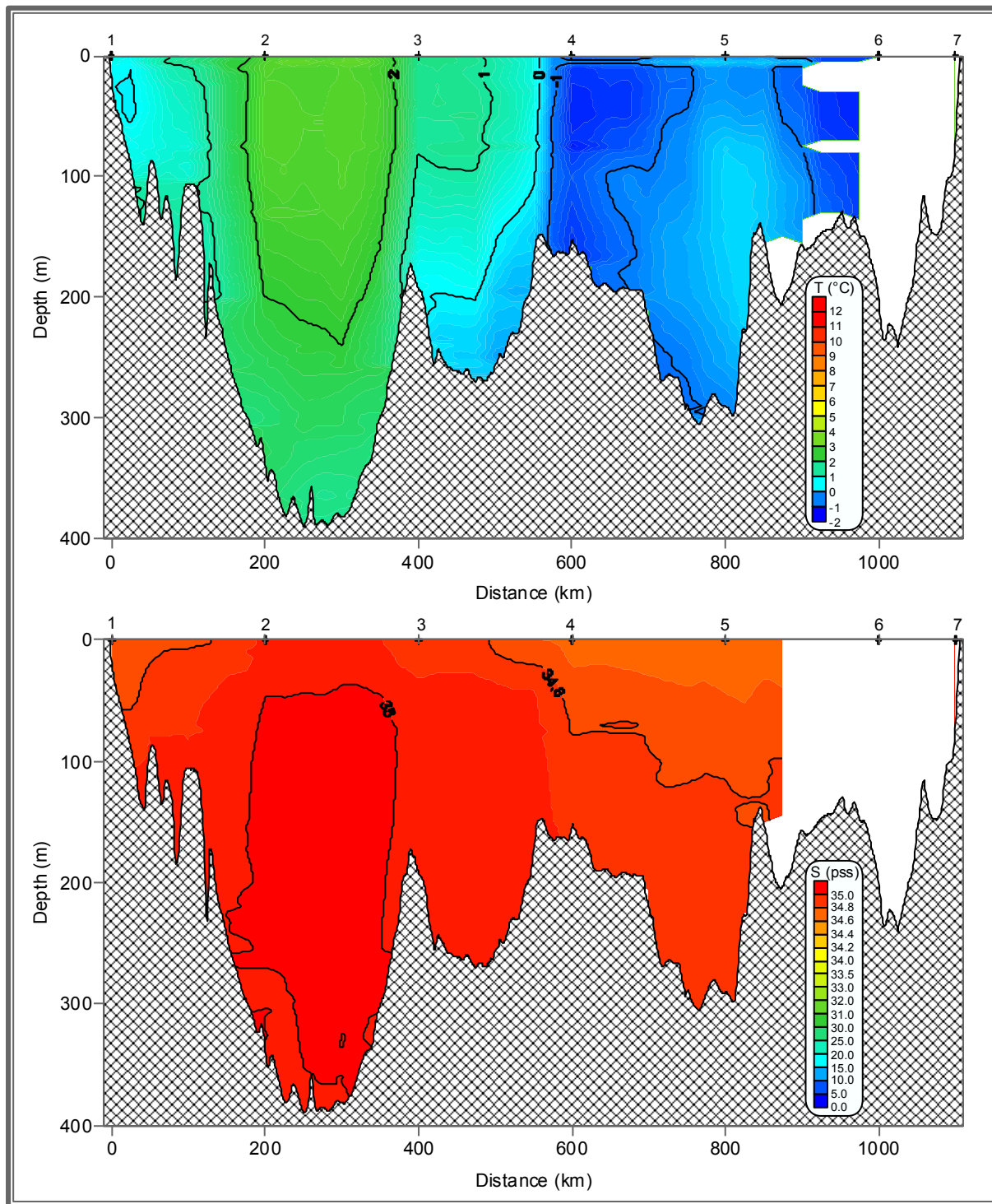
Temperature ( ^{\circ}\text{C} ), salinity (pss). May. Section B.
