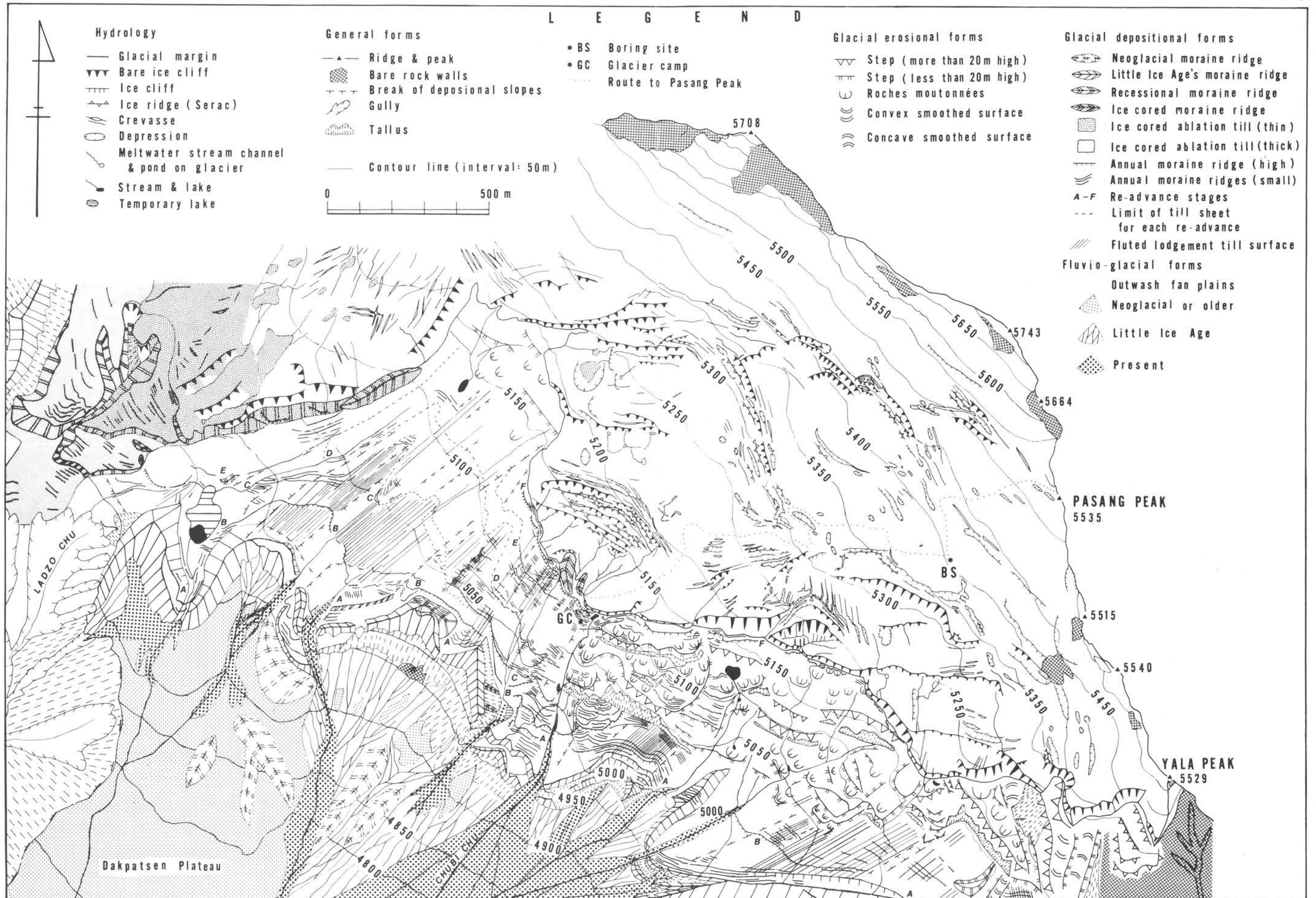
Figure 1 : Geomorphological Map of Proglacial Area of Yala (Dakpatsen) Glacier, Langtang Himal, Nepal.
