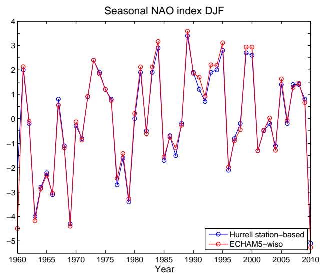
Figure 9. NAO winter (DJF) station index for the period 1960–2010, according to observations (blue line; Hurrell et al., 2013), and as simulated by the ECHAM5-wiso model (red line).
