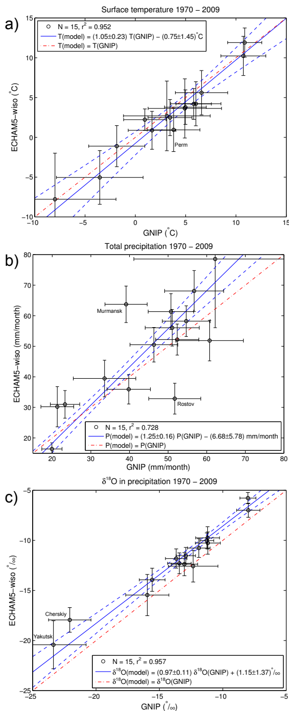
Figure 3. Comparison of mean values of (a) surface temperature, (b) precipitation amount, and (c) \delta^{18}\text{O} in precipitation for a selection of 15 GNIP stations located in Russia and the related ECHAM5-wiso model results (see text for details on station selection and mean value calculation at each station). Length of the error bars is \pm 2 standard errors of the estimated means. Straight lines are obtained from a weighted total least-squares algorithm accounting for uncertainties in both observations and model results (Krystek and Anton, 2007), dashed lines are 95 % confidence intervals for the fits.
