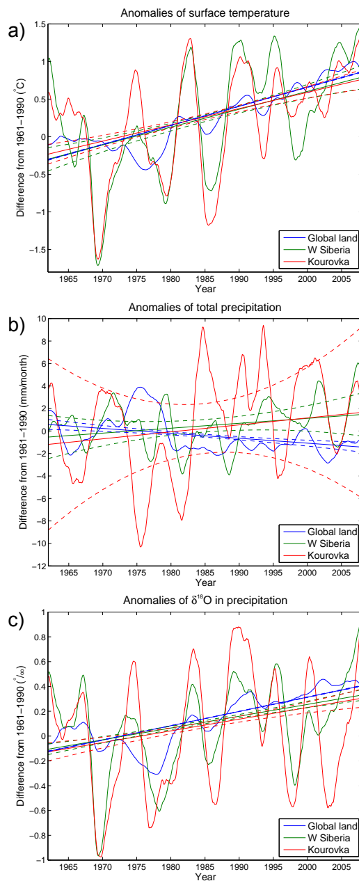
Figure 6. Simulated time series of (a) surface temperature, (b) precipitation, and (c) \delta^{18}\text{O} in precipitation for the period 1962–2008. Shown are anomalies from the climatological mean (reference period: 1961–1990). The ECHAM5-wiso results are averaged globally (blue line), for the region of western Siberia (green line), and interpolated to the location of Kourovka Observatory (red line). A zero-phase bidirectional low-pass filter with a length of 24 equally weighted months has been applied to the simulated monthly mean values for filtering short-term fluctuations. Straight lines are global (blue), regional (green) and local (red) trends obtained from least-square fits of annual-mean values for the period 1960–2010; dashed lines are 95 % confidence intervals for the trends. See also Table 2 for a summary of numerical results.
