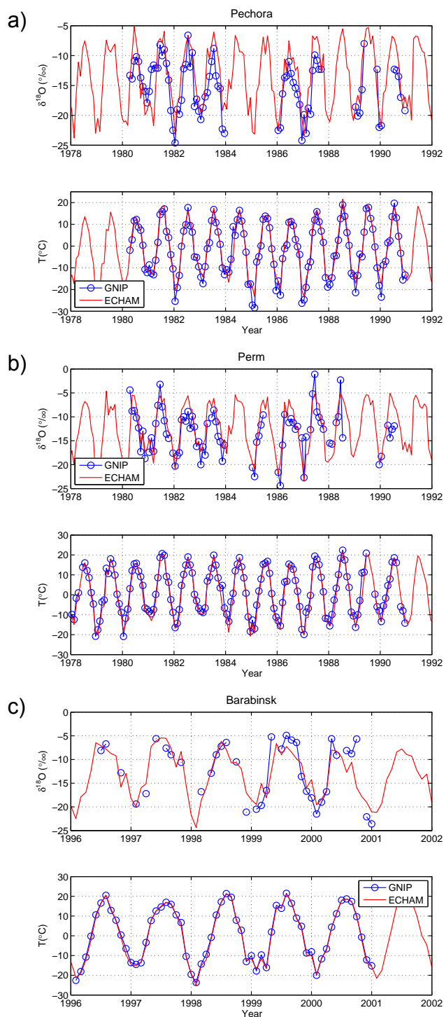
Figure 5. Observed versus modelled monthly \delta^{18}\text{O} values in precipitation for the period 1980–2000. Measurements of 3 GNIP stations located in western Siberia are plotted as blue circles: (a) Pechora, (b) Perm, (c) Barabinsk. The red line shows ECHAM5-wiso results corresponding to the same locations. Also shown are observed (blue) and modelled (red) surface temperatures.
