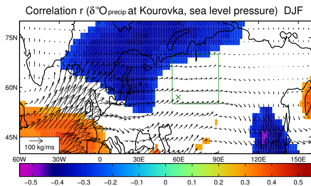
Figure 8. One-point correlation map showing the correlation between \delta^{18}\text{O} in precipitation at Kourovka and sea-level pressure during winter (DJF, correlation period is 1960–2010). Also shown is the average atmospheric moisture transport during DJF (vectors; only every second vector is drawn). The green box indicates western Siberia and the position of Kourovka is marked by a green cross.
