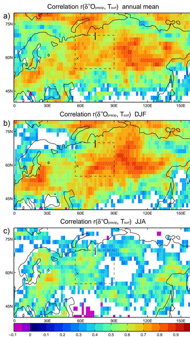
Figure 7. Temporal correlation between simulated values of \delta^{18}\text{O} in precipitation and surface temperatures for the period 1960–2010. Correlation coefficients are calculated for (a) annual mean, (b) winter (DJF), and (c) summer (JJA) values of temperature and \delta^{18}\text{O} . Statistically insignificant areas (where p \geq 0.05 applying a t test) are blanked.
