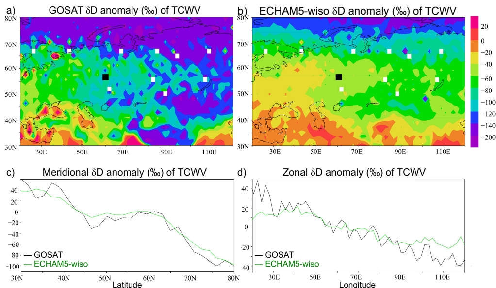
Figure 2. Distribution of annual-mean \delta D in total column water vapour, (a) as observed by the GOSAT satellite, (b) as simulated by ECHAM5, after collocation with GOSAT observations and convolution with the corresponding averaging kernels. In (a) and (b) the global average of \delta D has been subtracted to highlight spatial patterns, and the black squares indicate the location of Kourvka Observatory; white squares are grid cells with low-quality observations. (c) Meridional transects of observed (black) and simulated (green) \delta D averaged over the longitude band 50–70° E around Kourvka. The annual-mean \delta D value averaged over the area 30–80° N, 50–70° E has been subtracted to highlight the meridional variations. (d) Zonal transects of observed (black) and simulated (green) \delta D averaged over the latitude band 50–64° N around Kourvka. The annual-mean \delta D value averaged over the area 50–64° N, 20–120° E has been subtracted to highlight the zonal variations.
