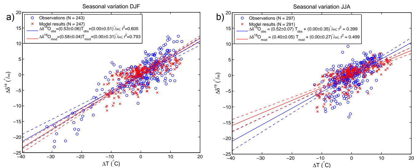
Figure 4. Relationship between \delta^{18}\text{O} and surface temperature. Shown are monthly anomalies ( \Delta\delta^{18}\text{O} and \Delta T ) according to monthly observations from 15 GNIP stations in Russia (circles) and the related ECHAM5-wiso model results (crosses), (a) winter season and (b) summer season. Solid lines are obtained from a least-squares linear fit of observations and model results; dashed lines indicate 95 % confidence intervals for the fits.
