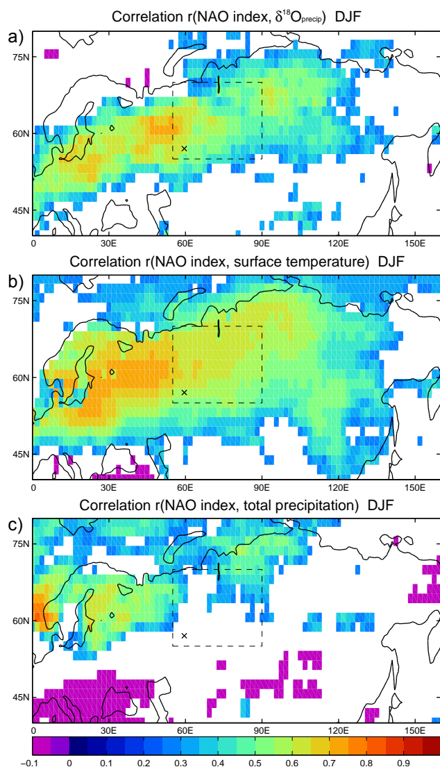
Figure 10. Temporal correlation between station-based NAO winter (DJF) index and (a) \delta^{18}\text{O} in precipitation, (b) surface temperature, and (c) total precipitation amount. Statistically insignificant areas (where p \geq 0.05 applying a t test) are blanked.
