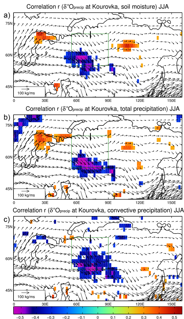
Figure 11. One-point correlation map showing the correlation between \delta^{18}\text{O} in precipitation at Kourovka during summer (JJA) with (a) soil moisture, (b) total precipitation, and (c) convective precipitation. Also shown is the average atmospheric moisture transport during JJA (vectors; only every second vector is drawn). The green box indicates western Siberia and the position of Kourovka is marked by a white cross. The correlation period is 1960–2010. Statistically insignificant areas (where p \geq 0.05 applying a t test) are blanked. See also Table 3 for numbers.
