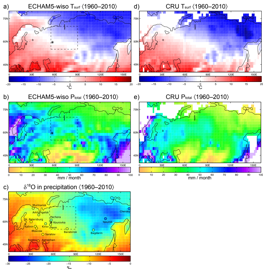
Figure 1. Left column: simulated mean annual values of (a) surface temperature, (b) precipitation, and (c) \delta^{18}\text{O} in precipitation, averaged over the period 1960–2010. Right column: CRU data of (d) surface temperature, and (e) precipitation amount, averaged over the same period. The circles in Fig. 1c mark the position of the various GNIP stations used for analyses in this study.
