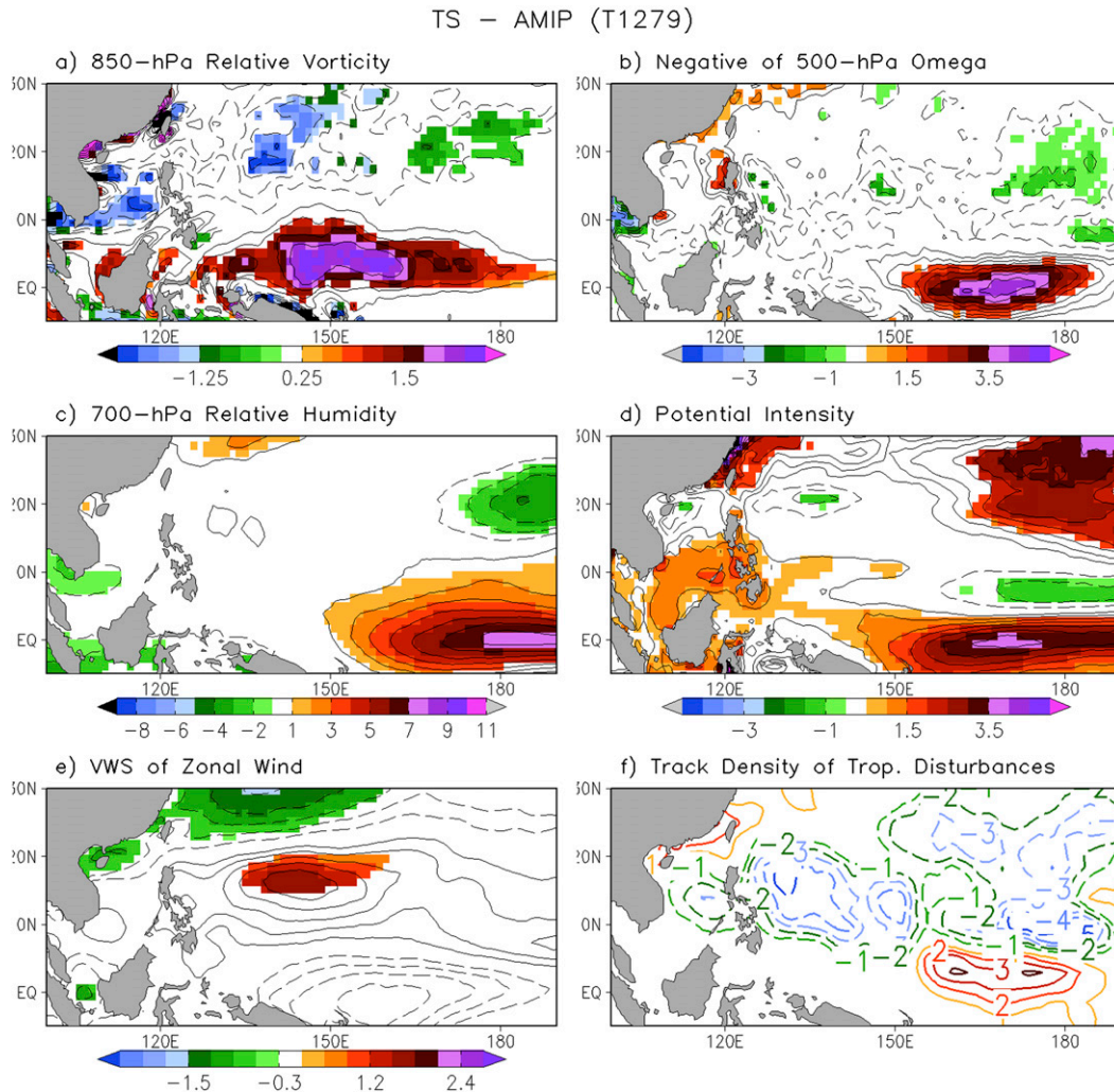
FIG. 8. MJJASON mean projected future change (TS – AMIP) in (a) 850-hPa relative vorticity ( 10^{-6} \text{ s}^{-1} ), (b) negative of 500-hPa \omega ( 10^{-2} \text{ Pa s}^{-1} ), (c) 700-hPa relative humidity (%), (d) potential intensity ( \text{ms}^{-1} ), (e) vertical shear of zonal wind ( \text{m s}^{-1} ; no absolute value taken), and (f) track density of synoptic-scale tropical disturbances (number density per season per unit area equivalent to a 5^\circ spherical cap) for IFS at T1279 based on the 47-yr simulations. In (a)–(e) shading shows changes significant at the 95% confidence level using a two-sided Student's t test. In (f) contour interval is 1.0. Positive (negative) contours are solid (dashed) with the starting value of 1.0 (–1.0).
