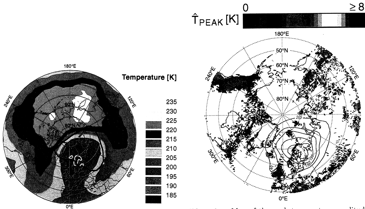
Plate 3. Map of the peak temperature amplitudes of mountain lee waves \hat{T}_{\text{PEAK}} at 50 hPa on February 1998 at 1200 UT. The data are obtained by simulations with a mountain wave forecast model [Bacmeister et al. , 1994]. The blue contours are the synoptic temperature isolines (absolute temperature [K]).
