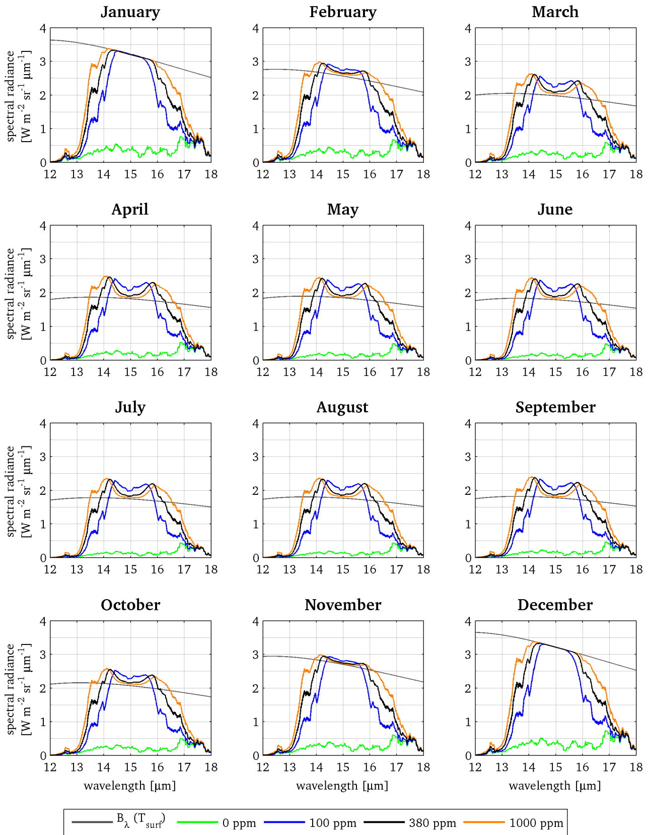
Figure 2.21: \text{CO}_2 -band of surface long-wave downwelling spectral radiance modelled with ALFIP. The spectra were calculated for south-polar clear-sky atmospheric conditions and various \text{CO}_2 concentrations. The spectra are low-pass filtered for clarity. The grey lines indicate the upward flux (Planck curves of surface skin temperature).
