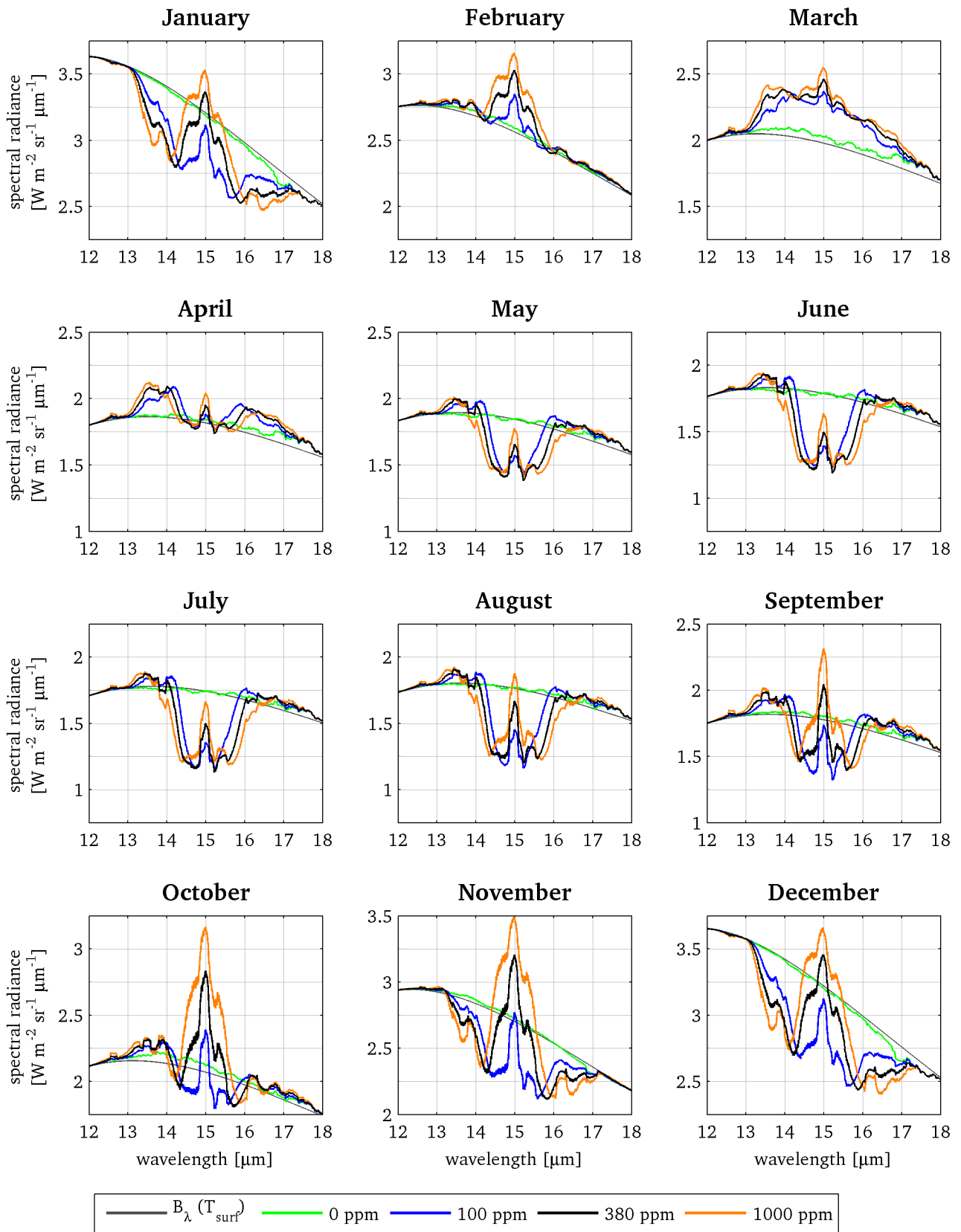
Figure 2.18: CO 2 -band of top of atmosphere long-wave emission modelled with ALFIP. The spectra were calculated for south-polar clear-sky atmospheric conditions and various CO 2 concentrations. The spectra are low-pass filtered for clarity. The grey lines indicate the surface emission (Planck curves of surface skin temperature).
