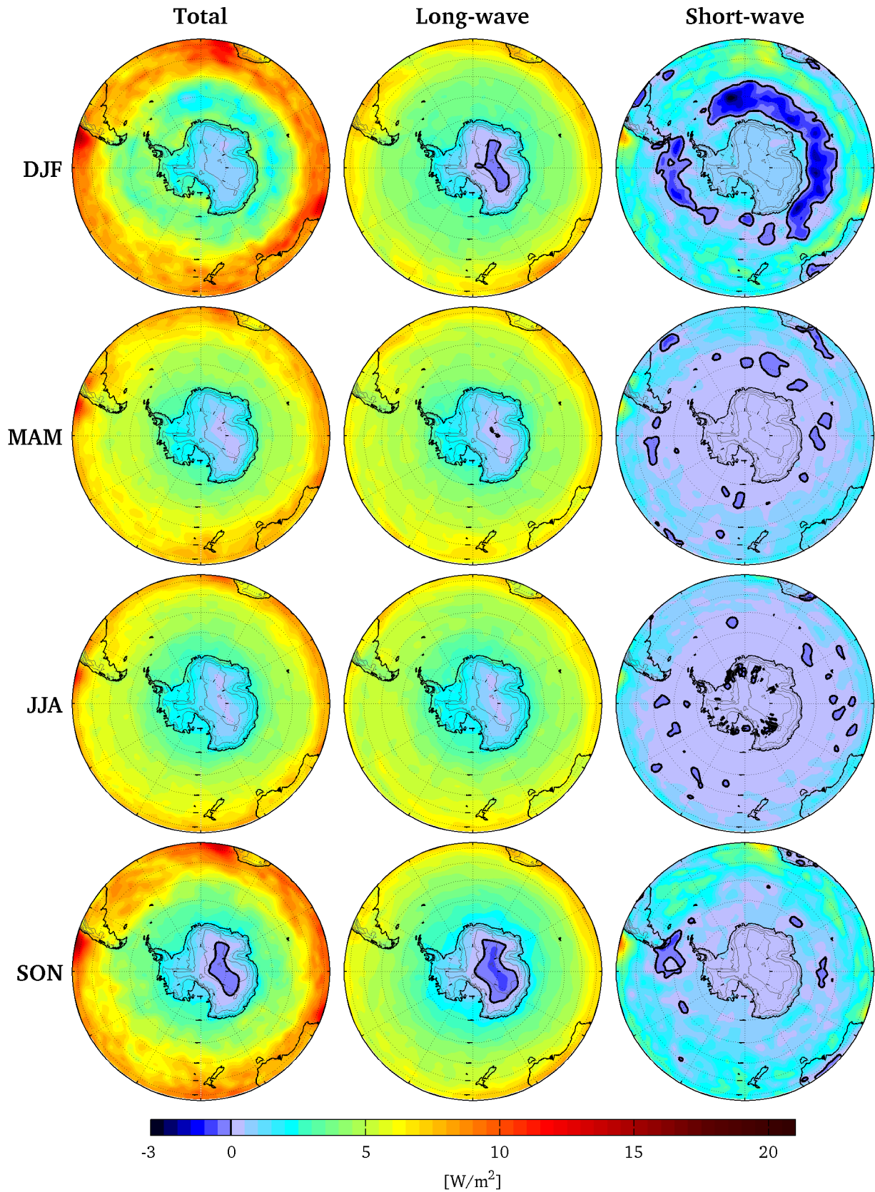
Figure 2.25: Changes in TOA outgoing radiative flux 15 days after quadrupling CO 2 in an ECMWF experiment for each season: summer (DJF), autumn (MAM), winter (JJA) and spring (SON). The fields shown are the differences "control run minus 4xCO 2 run" and were calculated as average over the years 1989 - 2010. The panels entitled Total are the sum of Long-wave and Short-wave . The black contour lines denote 0 W/m 2 . Surface elevation contour lines are shown in 1000 m intervals.
