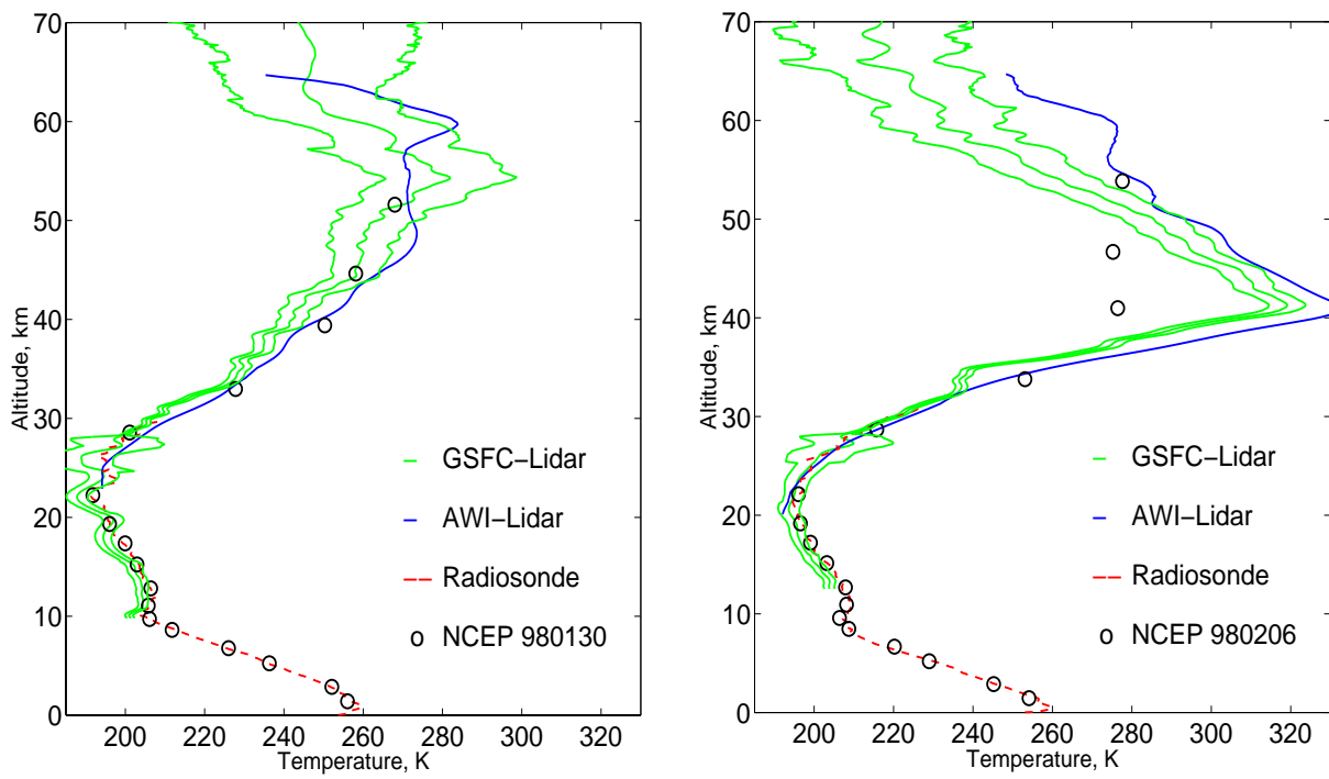
Fig. 3. Temperature profiles and NCEP analysis for 30 Jan. 98 (2a, left) and 6 Feb. 98 (2b, right). Light gray: GSFC lidar, black: AWI lidar, dashed: radio sonde, circles: NCEP analysis.
