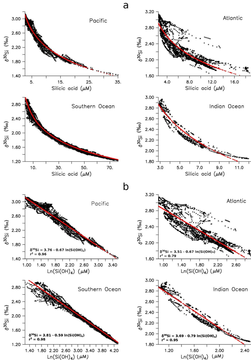
Figure 8. (a) \delta^{30}\text{Si} (‰) in upper 90 m water column versus silicic acid concentration ( \mu\text{M L}^{-1} ) in four different ocean basins and (b) \delta^{30}\text{Si} (‰) versus natural logarithm of silicic acid concentration ( \mu\text{M L}^{-1} ) in the according ocean basins. The red lines are linear regression curves of \delta^{30}\text{Si} versus \ln(\text{Si}(\text{OH})_4) in all panels, and the y intercepts of the regression lines are in per mil (‰) unit.
