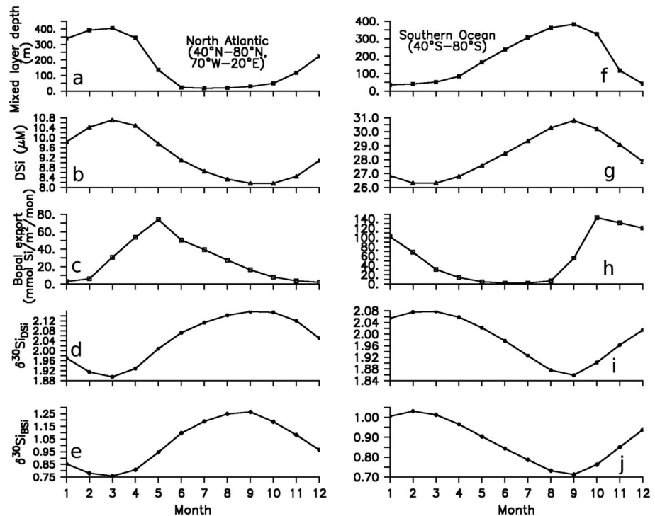
Figure 10. Seasonal variations of the (a, f) mixed layer depth (m), (b, g) silicic acid concentration ( \mu\text{mol L}^{-1} ) (averaged in the upper 90 m water depth), (c, h) biogenic opal export ( \text{mmol Si m}^{-2} ), (d, i) the \delta^{30}\text{Si} (‰) of silicic acid (averaged in the upper 90 m water depth), and (e, j) the \delta^{30}\text{Si} (‰) of biogenic opal (averaged in the upper 90 m water depth) in the North Atlantic (Figures 10a–10e) and in the Southern Ocean (Figures 10f–10j).
