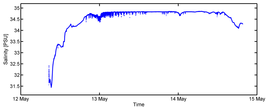
Figure 8: Salinity after despiking.
