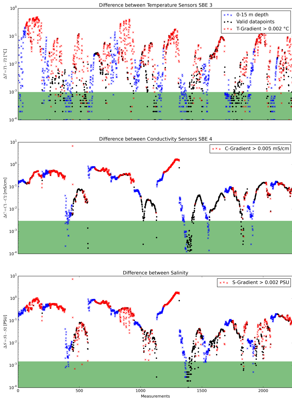
Figure 2: Data accuracy of sensor pairs HE459
