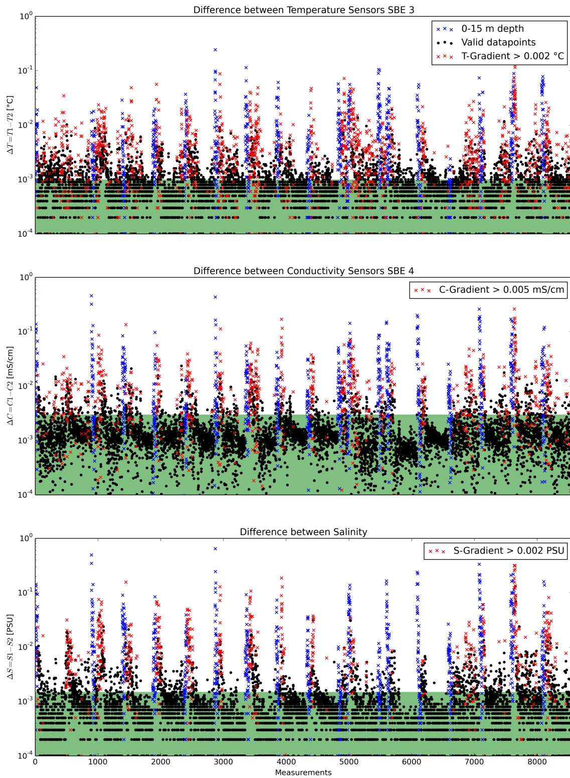
Figure 2: Data accuracy of sensor pairs HE462
