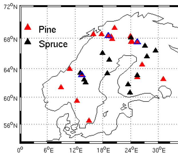
Fig. 1 The map of the study area and the locations of 34 tree-ring MXD chronologies covering the period of 1901–1978. Blue colors mark the locations of three millennium-long chronologies
