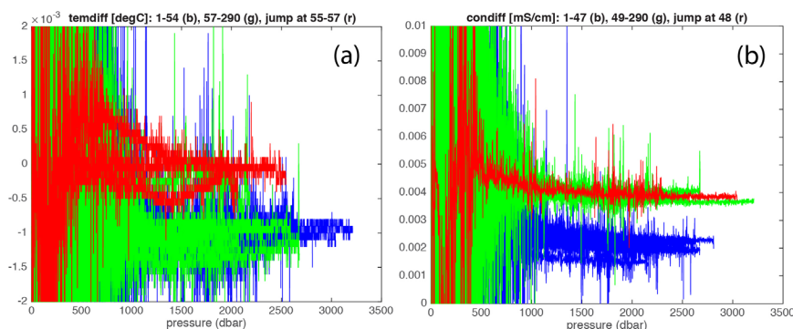
Fig. 3.3: (a) Difference in temperature sensors (secondary - primary) in large volume CTD. Station 1-54 in blue, station 55-57 in red, station 57-290 in green. (b) Difference in conductivity sensors (secondary - primary) in large volume CTD. Station 1-47 in blue, station 48 in red, station 49-290 in green.
