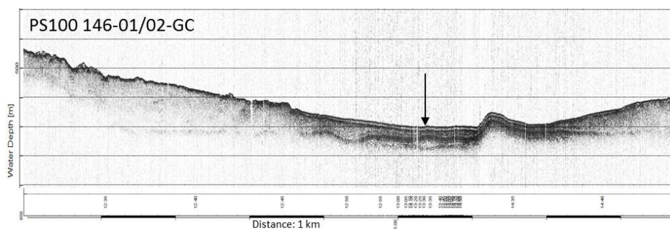
Fig. 4.3: A thicker sedimentary record with over 20m of sedimentary infill and four on-lapping units visible at core site PS 100 146-01-GC.
