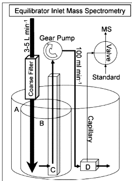
Fig. 6.2.2. Setup of the Equilibrator Inlet Mass Spectrometry. The large seawater reservoir (A) sits in a sink. After going through an inline coarse filter (500 µm pore size), seawater flows into the inner reservoir (B) at a rate of 3-5 L min -1 (large arrow). Most of the water running into B overflows into A, which is used as a water bath thermostated to the temperature of ambient seawater. A small fraction (100 mL min -1 ) of the high flow rate is pulled with a gear pump through a filter sleeve (C), with 100 and 5 µm pore size on the outside and inside, respectively. From the gear pump, the seawater flows through the equilibrator (D). The equilibrator sits in reservoir A to keep its temperature identical to that of the incoming seawater. A capillary, attached to the headspace of the equilibrator, leads to a multiport Valco valve. This valve alternates between admitting gas from the equilibrator and ambient air to the quadrupole mass spectrometer. An optode (not shown) in container B measures total oxygen saturation. Also not shown is a water flow meter located downstream of the equilibrator and thermocouples monitoring temperatures through the system (from Cassar et al., 2009).
