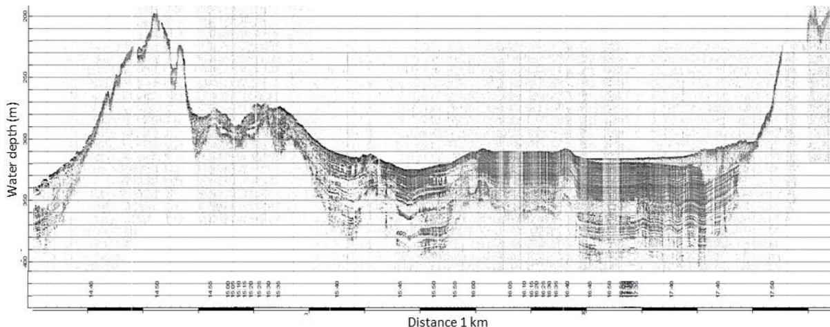
Fig. 4.7: A stratified basin infill typical of the inner Norske Trough. The stratified sediments are typically composed of alternating/banded red and grey clays. Overlying the stratified sediments are debris flows fed from the adjacent slopes (right hand side of image).
