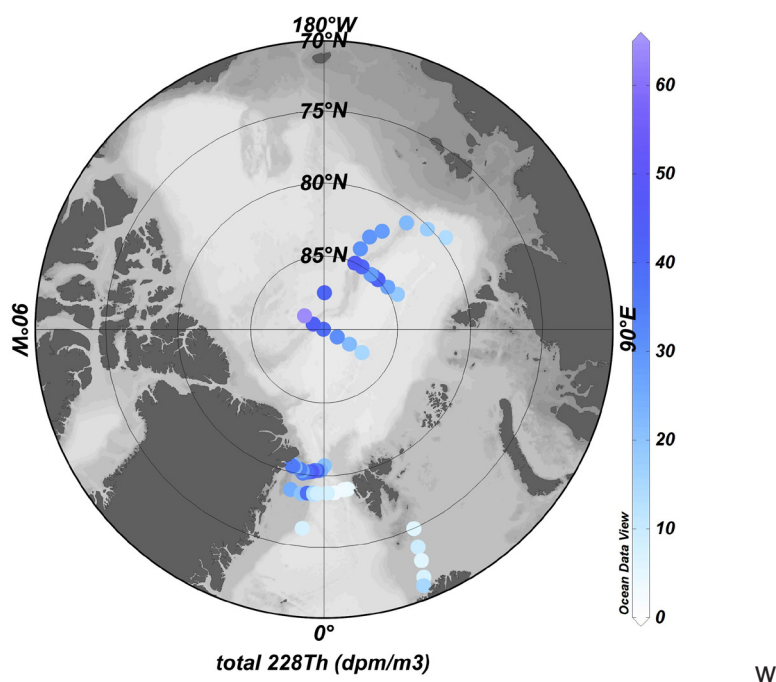
Fig. 6.7.1: Distribution of total ^{228}\text{Th} in surface water combining the data of expedition PS94 (ARK-XXVIII/3) and of the present cruise PS100 (ARK-XXX/2) up to station 120 showing the large contrast between the low concentrations in the inflowing Atlantic water and the high values in the East Greenland Current, likely derived from the Transpolar Drift.
