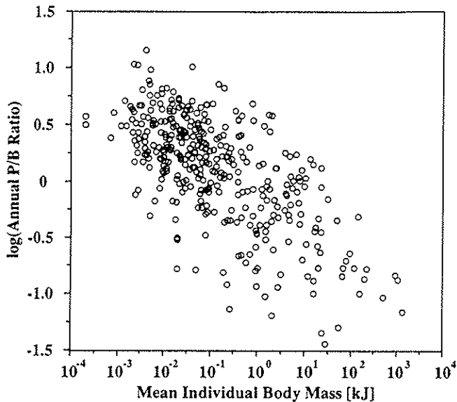
Fig. 3. Plot of \log(P/B) against \log(\text{Body Mass}) . (Regression: \log(P/B) = -0.124 - 0.252 * \log(M) ; r = 0.667 , n = 363 .)
