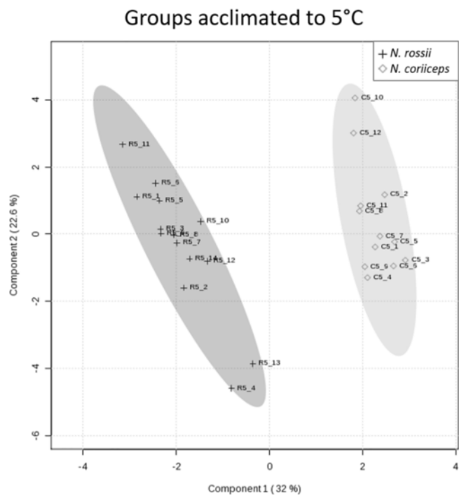
Fig. 4. PLS-DA Score plot for the normalised concentrations of assigned metabolites from gill tissue extracts of notothenioids acclimated to 5 °C. Ellipses correspond to a confidence interval of 95% for each group.
