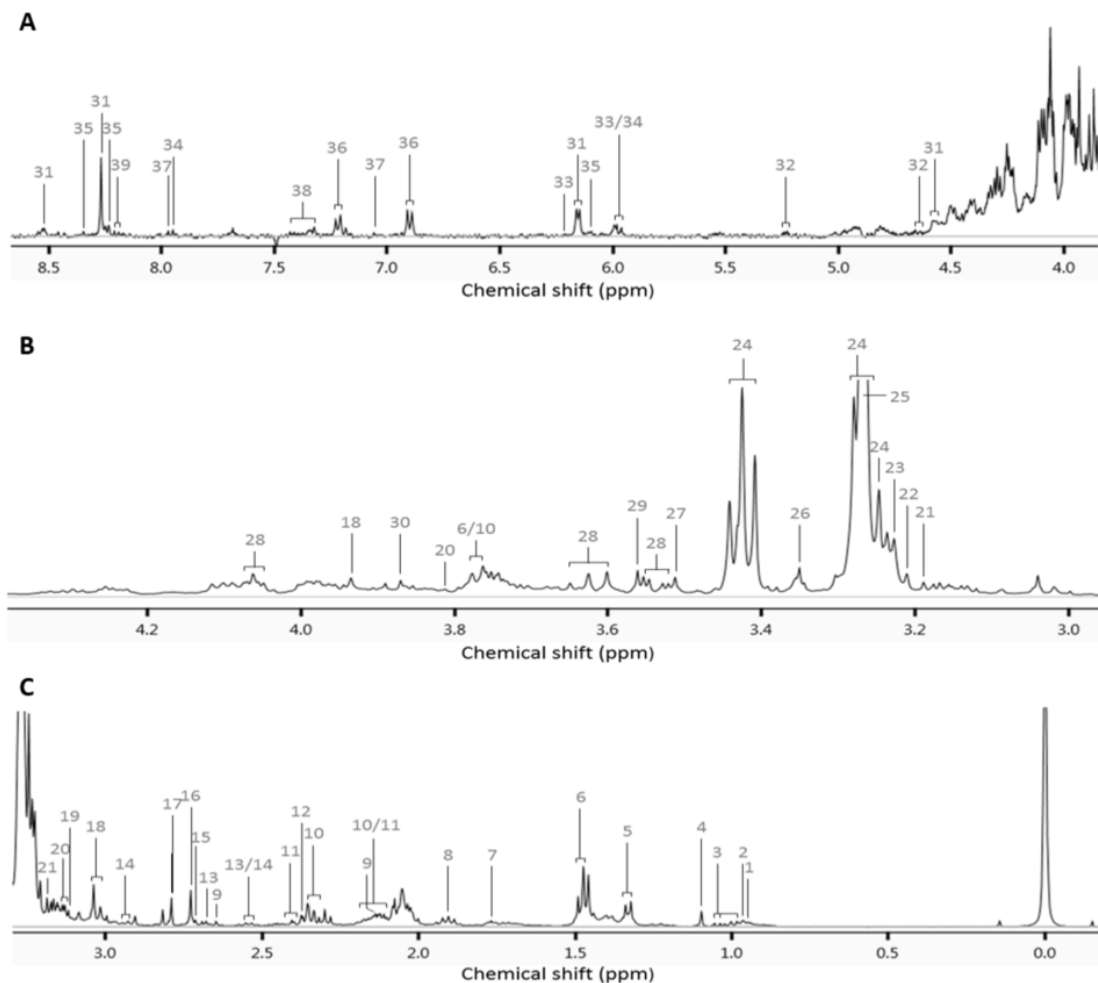
Fig. 1. Representative one dimensional 400 MHz CPMG ^1\text{H} -NMR spectra of gill tissue extract from Notothenia rossii acclimated to 0 °C with vertical expansion of the different regions (A-C). Keys: 1 Isoleucine; 2 Leucine; 3 Valine; 4 Unknown 1; 5 Lactate; 6 Alanine; 7 Putrescine; 8 Acetate; 9 Methionine; 10 Glutamate; 11 Glutamine; 12 Succinate; 13 Citrate; 14 Glutathione; 15 Dimethylamine (DMA); 16 Sarcosine; 17 Unknown 2; 18 Creatine/Phosphocreatine; 19 Malonate; 20 Ethanolamine; 21 Choline; 22 Phosphocholine; 23 Glycerophosphocholine; 24 Taurine; 25 Trimethylamide-N-oxide (TMAO); 26 Unknown 3; 27 Unknown 4; 28 myo-Inositol; 29 Glycine; 30 Betaine; 31 ATP/ADP; 32 Glucose; 33 NADH/NADPH; 34 UDP-Glucose; 35 Inosine; 36 Tyrosine; 37 Histidine; 38 Phenylalanine; 39 Hypoxanthine. Signals in the area between 4 and 4.5 ppm resulted from various alpha amino acids, alcohols, polyols and saccharides.
