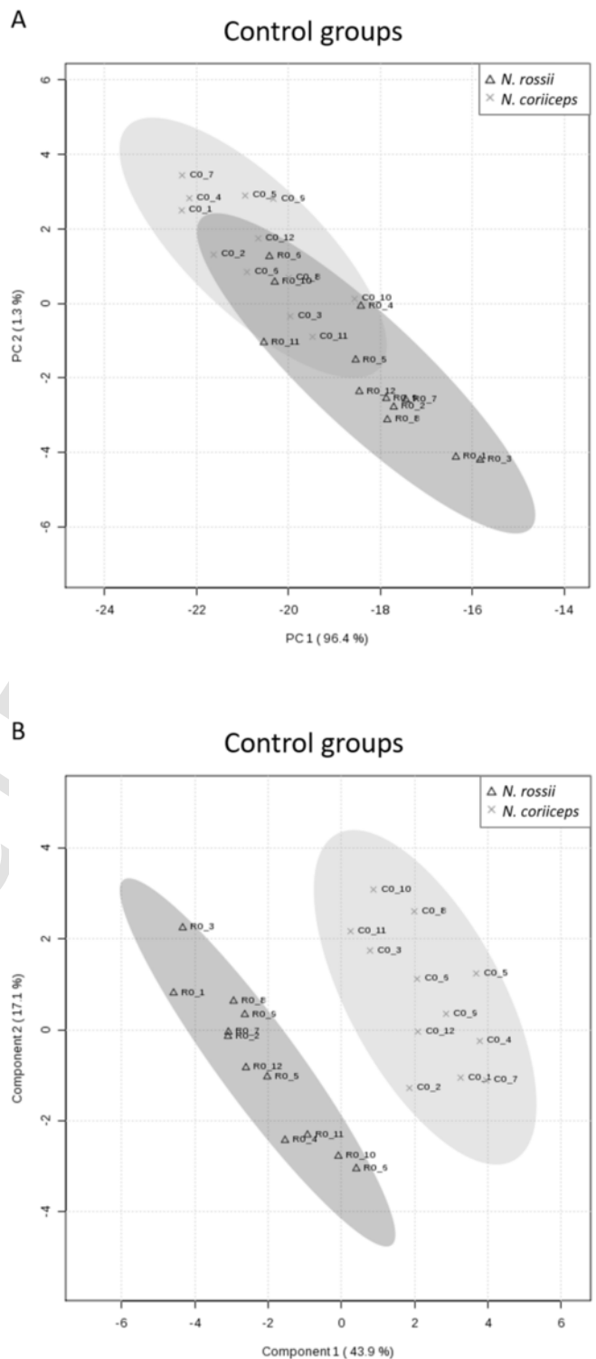
Fig. 2. A. Principal component analysis (PCA) of the normalised concentrations of assigned metabolites in the control groups acclimated to 0^\circ\text{C} . B. Score Plot of the PLS-DA model for the normalised concentrations of assigned metabolites from gill tissue extracts in control groups of the two Antarctic fish species acclimated to 0^\circ\text{C} . Ellipses correspond to a confidence interval of 95% for each group.
