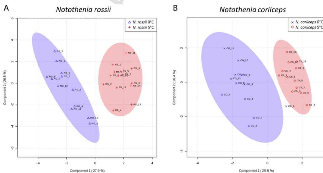
Fig. 3. Score Plot of the PLS-DA model for the normalised concentrations of assigned metabolites of gill tissue extracts of Notothenia rossii (A) and Notothenia coriiceps (B) acclimated to 0 °C and 5 °C. Ellipses correspond to a confidence interval of 95% for each group.
