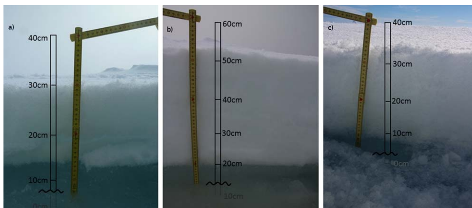
Figure 7. Snow pits with flooded snow pack on Floe 4 on 14 June 2015 on three different sites. (a) Close to the ship, water level at 0.075 m, wet snow until 0.14 m, total snow depth 0.30 m. (b) Water level at 0.13 m, wet snow until 0.19 m, total snow depth 0.53 m. (c) Water level at 0.06 m, wet snow until 0.09 m, total snow depth 0.34 m.
