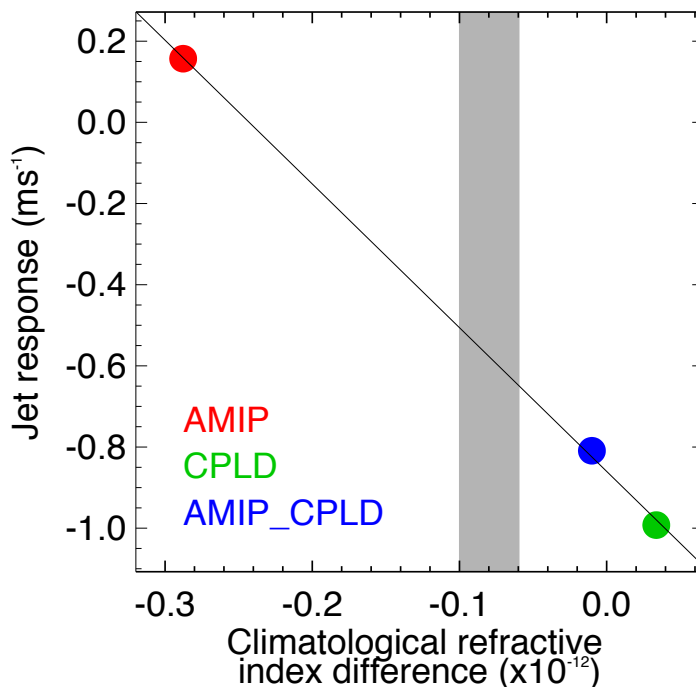
Figure 14. Dependence of Atlantic jet response on the background climatological refractive index difference between mid (25-35oN) and high (60-80oN) latitudes at 200 hPa. Grey shading shows the observed range from the ERA-Interim and NCEP II reanalyses. The Atlantic jet response is defined as the difference in zonal mean zonal wind at 200 hPa over the region 60-0oW, 50-60oN between model experiments with reduced and climatological Arctic sea ice. Experiments were performed with the same model but with three different configurations: atmosphere only (AMIP); fully coupled (CPLD); and atmosphere only but with SST biases from the coupled model (AMIP_CPLD). An “emergent constraint” is obtained where the observed refractive index difference (grey shading) intersects the simulated response (black line), suggesting a modest weakening of the Atlantic jet in response to reduced Arctic sea ice (Figure from Smith et al. 2017).
