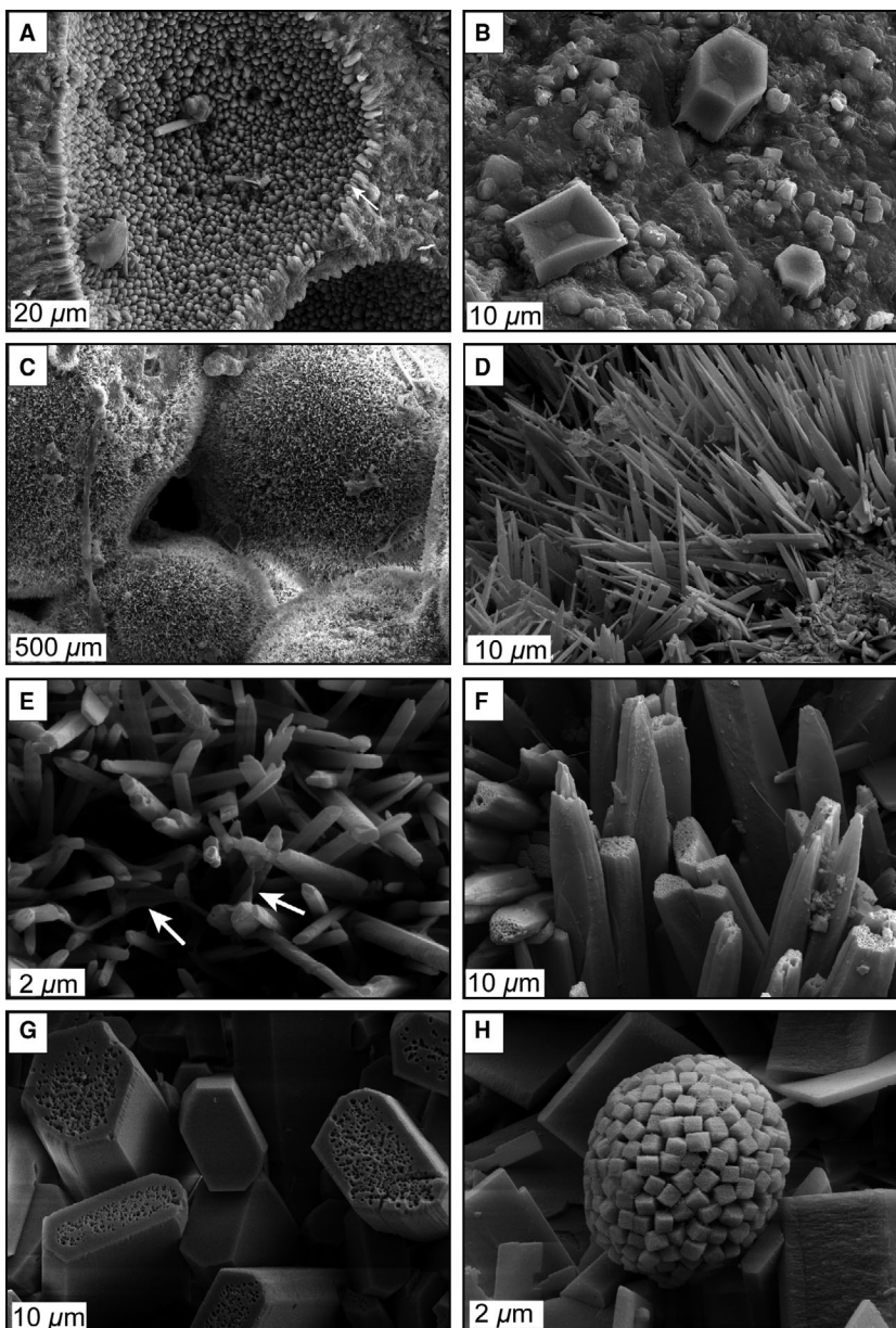
Fig. 12. Scanning electron microscope (SEM) images of various cement types from the Abu Dhabi lagoon and intertidal sabkha. (A) Micritic and rhombic high-Mg calcite cements within a bioclast chamber from the Khawr as Sadiyat (KAS) middle lagoon. (B) Polygonal gypsum cements covering a grain surface from the KAS middle lagoon. (C) Acicular aragonitic cement covering oolitic and peloidal sediment from the KAS outer lagoon. Note the microbial filaments. (D) Acicular (needle) aragonitic cements from the high-energy settings of the Al Gharbia (AG) inner lagoon. (E) Outer KAS lagoon fibrous aragonitic cements, with associated microbial filaments (arrowed). (F) Fibrous aragonitic cements with small holes at the termination, Khawr Qantur (KQ) inner lagoon. (G) KAS inner lagoon cements showing elongated prismatic aragonite cements with voids at the (001) (termination) surface. (H) Platy aragonitic cements associated with framboids in the KAS inner lagoon.
