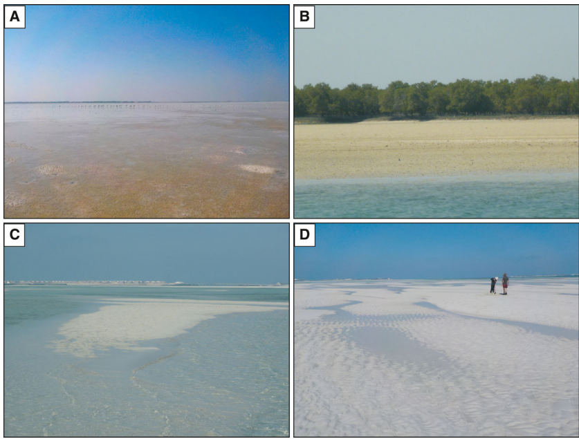
Fig. 5. Field photographs from the middle and outer lagoon. (A) Extremely shallow water with localized exposure at the Khawr as Sadiyat (KAS) middle lagoon during low tide. The width of the image in the foreground is ca 5 m. (B) Localized mangroves in the KAS middle lagoon. The mangroves are ca 3 m high. (C) Exposed ooid shoal during low tide at the KAS outer lagoon. The width of the image in the foreground is ca 6 m. (D) Wave ripples and tidal creeks on the crest of a Shalil al Ud (SAU) outer lagoon ooid shoal (persons to the right are ca 1.8 m tall).
