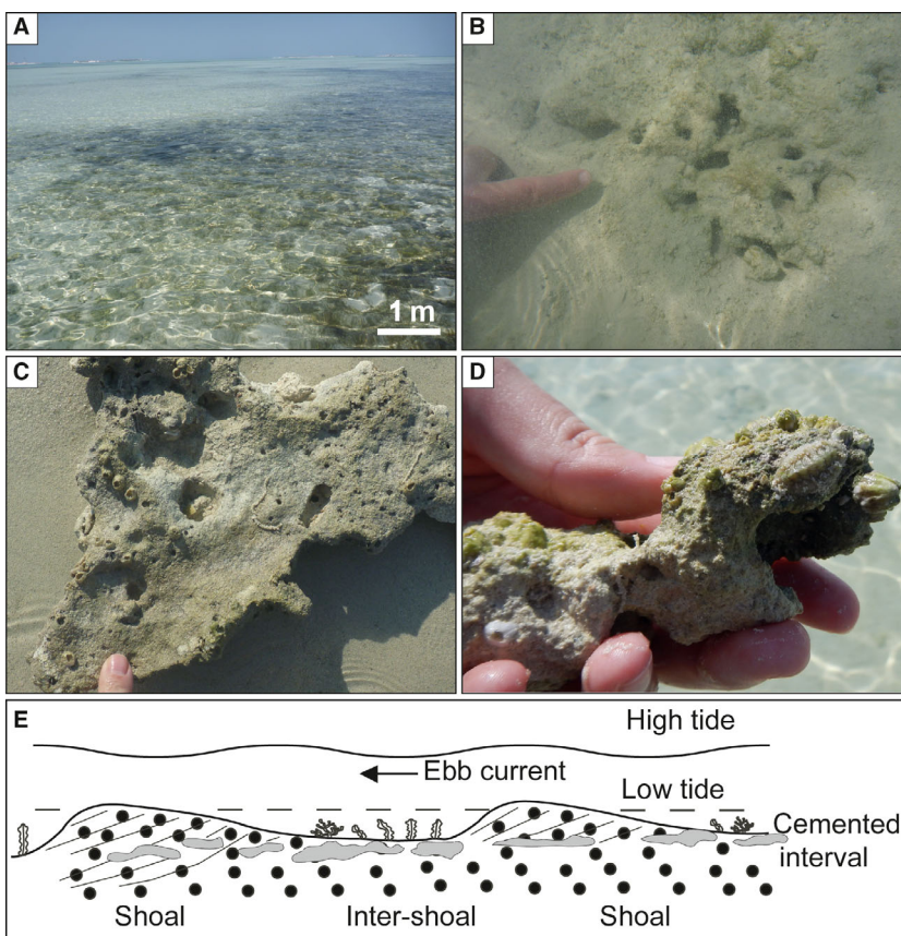
Fig. 10. Cemented intervals from the ooid shoal environment. (A) Shallow water depth and seagrass colonization (dark areas). The width of the image in the foreground is ca 7 m. (B) Subaqueous concretionary cemented decapod burrow network interval. Note the holes formed due to unconsolidated sediment removed by currents. (C) The upper surface of an encrusted, ooid shoal-associated cemented interval. (D) The typical irregular morphology of a lithified decapod burrow. (E) Schematic of hardground occurrence in the ooid shoal setting. Grey colour refers to cemented burrow network.
