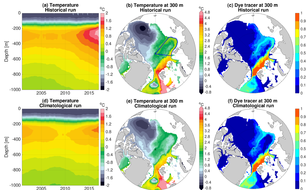
Figure 4. (a) Hovmöller diagram of temperature averaged over the eastern Eurasian Basin (indicated by the blue box in (b)) in the historical run. (b) Temperature at 300 m depth averaged over the last 3 years in the historical run. (c) Dye tracer at 300 m depth averaged over the last 3 years in the historical run; the tracer is released in the Atlantic Water layer east of 0°E at Fram Strait. (d, e, f) The same as (a)–(c), respectively, but for the climatological run.
