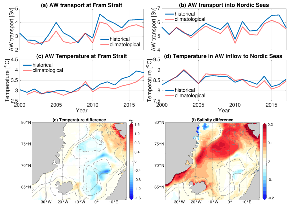
Figure 2. Atlantic Water volume transport through (a) Fram Strait ( >2\text{ }^{\circ}\text{C} ) and (b) into the Nordic Seas at the Iceland-Faroe-Scotland Ridge (IFSR, >4\text{ }^{\circ}\text{C} ). The temperature threshold values were suggested based on observations by Beszczynska-Moeller et al. (2012) and Hansen et al. (2015) for the Fram Strait and Nordic Seas inflow, respectively. Atlantic Water temperature at (c) Fram Strait and (d) IFSR. (e) Difference of temperature between the two runs (historical minus climatological runs) averaged over the upper 300 m and the last 10 years. (f) The same as (e), but for salinity.
