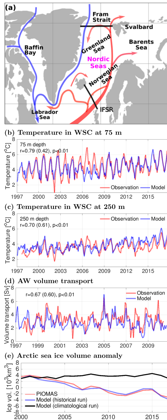
Figure 1. (a) Schematic of Arctic Ocean-North Atlantic exchange currents. The red arrows indicate the currents carrying the Atlantic Water (AW), and the blue arrows indicate freshwater export from the Arctic Ocean. The Fram Strait and Iceland-Faroe-Scotland Ridge (IFSR) are indicated with black lines. (b, c) Temperature in the West Spitsbergen Current (WSC) core (averaged over the three easternmost moorings) at different depths in Fram Strait in the historical run and mooring observations. The Fram Strait mooring observations are described by Beszczynska-Moeller et al. (2012) and von Appen et al. (2016). (d) AW ( > 2^{\circ}\text{C} ) volume transport in the WSC at the Fram Strait in the historical run and observations. The observed volume transport and the argument for the temperature threshold of the AW are provided by Beszczynska-Moeller et al. (2012). (e) Anomaly of Arctic sea ice volume in the PIOMAS reanalysis (Schweiger et al., 2011) and in the two model runs. The anomalies of PIOMAS and the historical run are referenced to their respective mean values averaged over the shown period, and the anomaly of the climatological run is referenced to the mean value of the historical run. In (b)–(d) the correlation coefficients between the two time series are shown for both monthly data and 13-month running means (in parenthesis).
