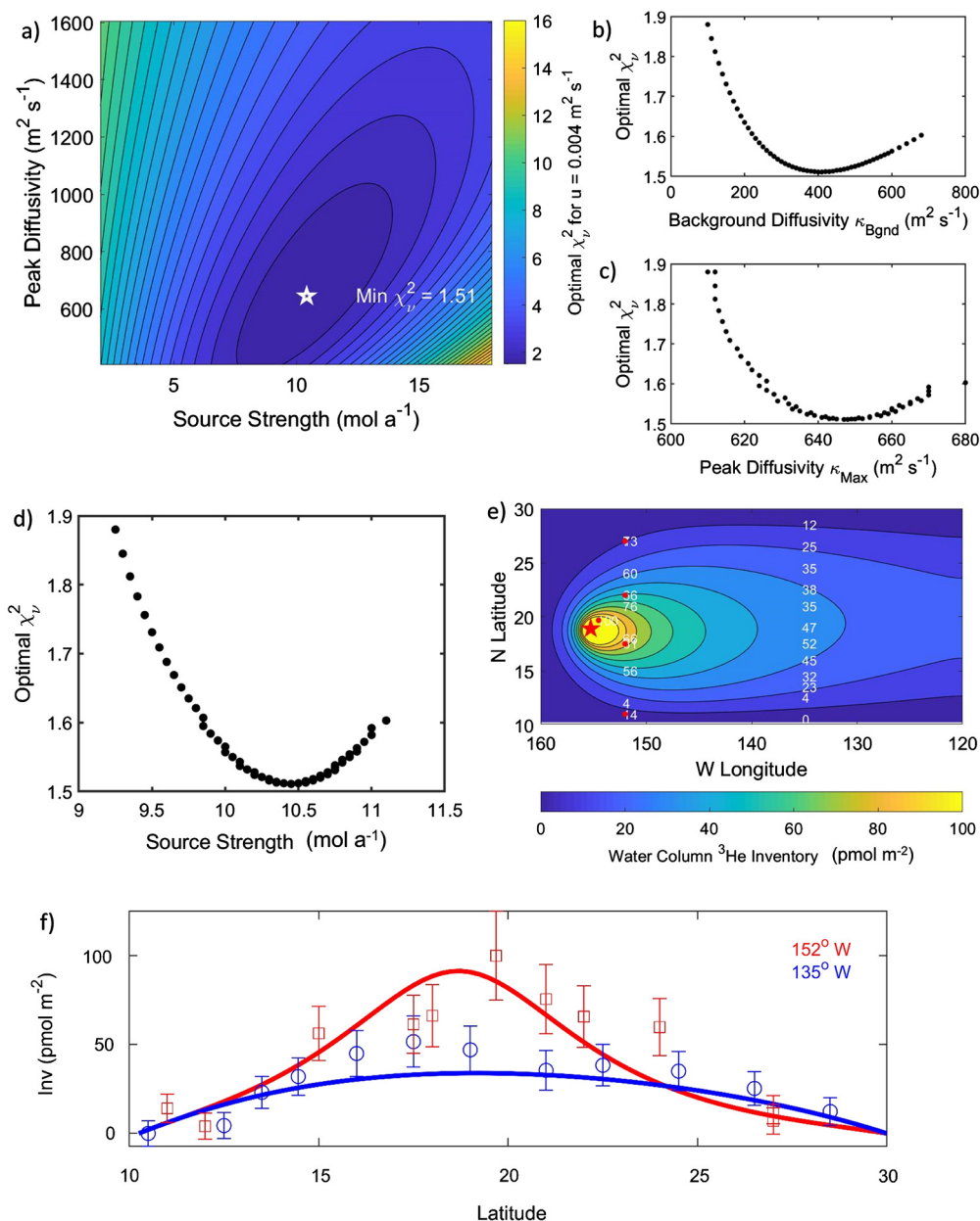
Fig. 9. (a) A contour plot \chi^2_{\nu} (model-data misfit) as a function of ^3\text{He} source strength (Loihi flux) and peak horizontal diffusivity of the case of an eastward velocity of 0.004 \text{ m s}^{-1} and optimized background diffusivity of 405 \text{ m}^2 \text{s}^{-1} . (b) The variation of optimal \chi^2_{\nu} as a function of background diffusivity, (c) peak diffusivity, and (d) source strength. (e) The model Loihi ^3\text{He} plume inventory distribution for the globally optimal case of 10.43 \text{ mol a}^{-1} source strength, background diffusivity of 405 \text{ m}^2 \text{s}^{-1} and 645 \text{ m}^2 \text{s}^{-1} peak horizontal. Observed inventories used to constrain the optimization are posted in \text{pmol m}^{-2} (white numbers). (f) a comparison of measured inventories (open symbols with error bars) and optimum model prediction for the two sections ( \sim 152^\circ \text{W} red, \sim 135^\circ \text{W} blue) as a function of latitude.
