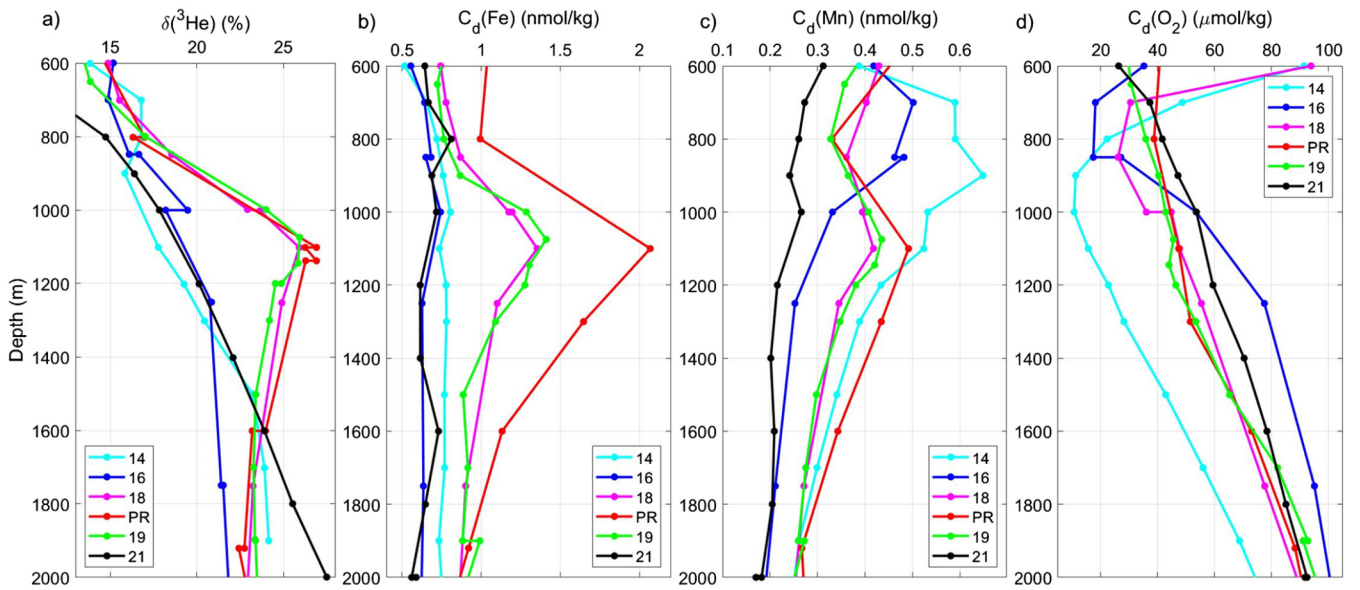
Fig. 5. Composite depth profiles at the distal stations of a, \delta^3\text{He} in %, b, dissolved Fe in \text{nmol kg}^{-1} , c, dissolved Mn in \text{nmol kg}^{-1} , and d, dissolved oxygen in \mu\text{mol kg}^{-1} for the more distant stations shown in Fig. 1 (not including the Loihi station). From north to south they are station 14 (cyan), 16 (blue), 18 (magenta), Puna Ridge (red), 19 (green), and 21 (yellow). Note the pronounced maxima in \delta^3\text{He} , dFe, and dMn at 1100 m depth identified in \delta^3\text{He} by Lupton (1996) as the Loihi plume for the “nearby” stations (Puna Ridge, 18, and 19). Also, note the aberrant behavior for the dMn (and to a lesser extent dFe) for station 14.
