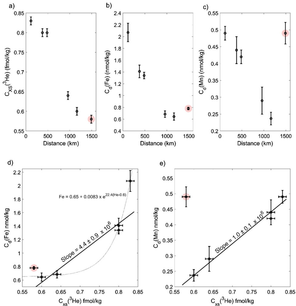
Fig. 6. The distal excess ^3\text{He} , dissolved iron, and manganese concentration variation vs. distance from Loihi for a. excess ^3\text{He} in \text{fmol kg}^{-1} , b. dissolved Fe in \text{nmol kg}^{-1} , and c. dissolved Mn in \text{nmol kg}^{-1} . Correlation with excess ^3\text{He} for d. dissolved Fe and for e. dissolved Mn. Error bars, which combine analytical and interpolation uncertainties, are 1\sigma for both variables. The solid lines are from type-II weighted linear regressions (excluding station 14, highlighted in pink for Fe and Mn). The dashed line in d is an exponential fit for comparison.
