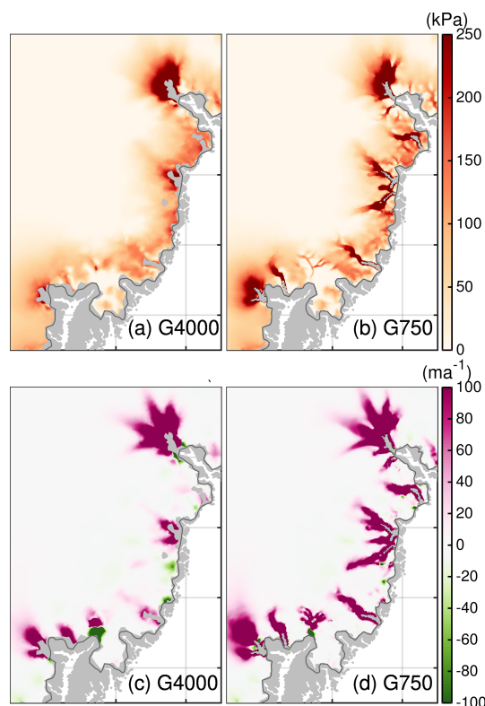
Figure 12. (a, b) Difference in effective pressure between 2100 and 2015 for the southeast region. (c, d) Difference in basal velocity between 2100 and 2015 for the southeast region. Region subsets are shown in Fig. 2. Dark grey line indicates the initial ice extent. Thin black line indicating the grounding line is not visible as it falls together with the calving front. The grey silhouette shows the Greenland land mask from BedMachine v3.
