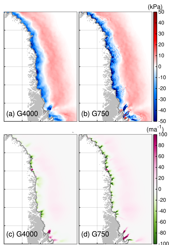
Figure 13. (a, b) Difference in driving stress between 2100 and 2015 for the northwestern region. (c, d) Difference in basal velocity between 2100 and 2015 for the northwestern region. Region subsets are shown in Fig. 2. Dark grey line indicates the initial ice extent. Thin black line indicating the grounding line is not visible as it falls together with the calving front. The grey silhouette shows the Greenland land mask from BedMachine v3.
