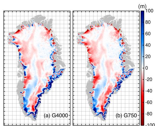
Figure 7. Difference in ice thickness between 2100 and 2015 for the ctrl run. (a) G4000 simulation and (b) G750 simulation. The grey silhouette shows the Greenland land mask from BedMachine v3. Positive values represent thickening, and negative values show thinning. Thin yellow line shows the grounding line in the year 2100.
