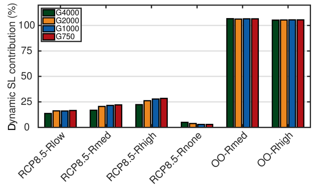
Figure 9. Mass loss partitioning for the conducted experiments. The bars indicate the relative dynamic contribution to sea level, calculated as the residual of the total of the mass change and the integrated SMB anomaly. The residual is a composition of front retreat and ice discharge.
