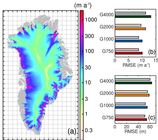
Figure 5. Simulation results and error estimate of model output at the end of the historical run compared to observations. (a) Simulated surface velocity of the GrIS ( \text{m a}^{-1} ) from the G750 simulation. The grey silhouette shows the Greenland land mask from BedMachine v3. Thin black lines show the grounding line. (b) Root mean square error (RMSE) of the horizontal velocity magnitude compared to MEaSUREs. (c) RMSE of ice thickness (not corrected with ctrl) compared to BedMachine v3. In panels (b) and (c) , light and dark colours represent diagnostics at the initialization and end of the historical experiment, respectively. The diagnostics have been calculated on the regular MEaSUREs and BedMachine grids, respectively.
