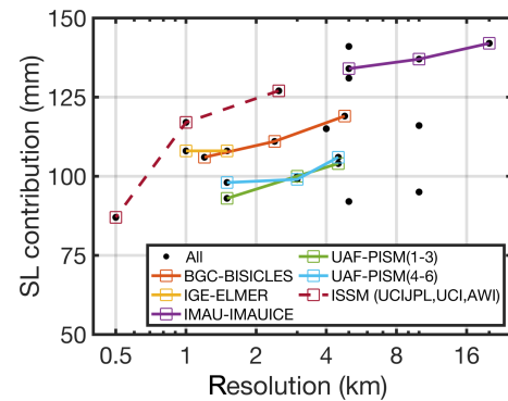
Figure 1. Results from the initMIP-Greenland exercise (Goelzer et al., 2018). Sea-level contribution vs. (minimum) horizontal grid resolution of each participating ISM. Equal model versions but different grid resolutions are connected with a coloured line. ISSM model versions are connected with a coloured dashed line. Note the logarithmic scale of the x axis. For unstructured meshes the finest resolution is displayed.
