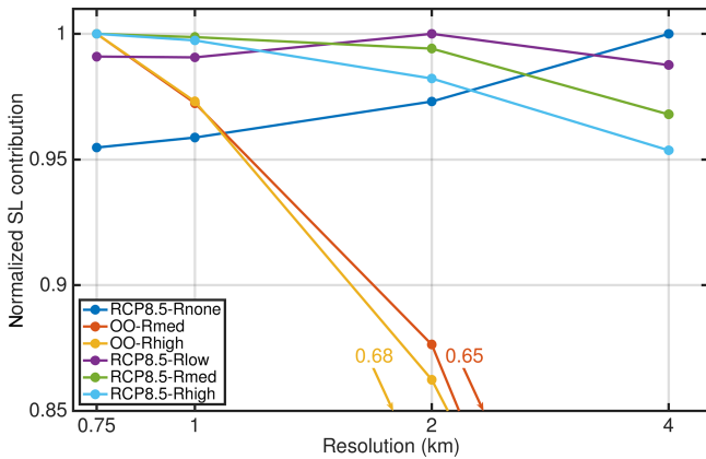
Figure 8. Projected sea-level contribution in 2100 of the Greenland ice sheet as a function of the horizontal grid size. Values are normalized to the maximum of each experiment (coloured lines). Note the logarithmic scale of the x axis.
