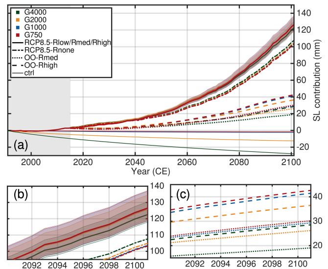
Figure 6. Projected sea-level contribution of the Greenland ice sheet based on MIROC5 RCP 8.5 climate data (a) . Coloured lines indicate the different grid resolutions employed, while the individual scenarios are indicated with different line styles. The mass loss trends are corrected with the ctrl run relative to the reference time. The grey-shaded box shows the historical period. (b) Enlargement of the RCP8.5-Rlow, RCP8.5-Rmed, RCP8.5-Rhigh and RCP8.5-Rnone scenarios. (c) Enlargement of the OO-Rmed and OO-Rhigh scenarios.
