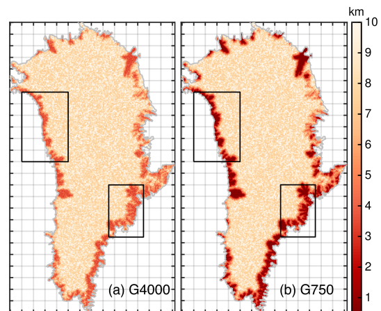
Figure 2. Horizontal mesh resolution (km) used for G4000 (a) and G750 (b). Data are clipped at 0.5 and 10 km. The horizontal resolution of a triangle is defined by its minimum edge length. The grey line delineates the initial ice domain. Grey grid lines indicate 100 km. The black boxes indicate the northwestern and southeast subsets used in following figures.
