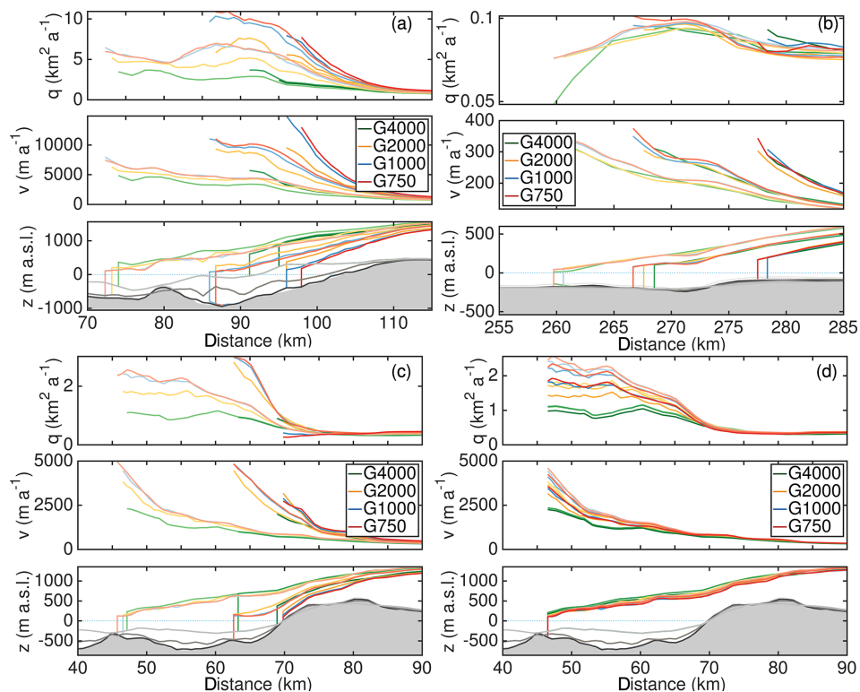
Figure 11. Response of outlet glaciers. Colour scheme is the same as in previous figures, and light to dark colours indicate the years 2015, 2070 and 2100. (a) Helheim Glacier under RCP8.5-Rhigh forcing. (b) Humboldt Glacier under RCP8.5-Rhigh forcing. (c) Store Glacier under RCP8.5-Rhigh forcing. (d) Store Glacier under RCP8.5-Rnone forcing. Upper rows show the transient behaviour of the ice discharge q , the middle rows the surface velocity v and lower rows the evolution of the ice geometry. In the lower rows, the grey-shaded area depicts the bedrock topography from the G750 simulation. The grey lines from dark to light indicate the bedrock topography from the G1000, G2000 and G4000 simulation. None of the quantities are corrected with the ctrl run. Distance is relative to an arbitrary point.
