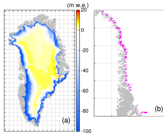
Figure 4. Atmospheric and oceanic forcing. (a) Spatial pattern of the cumulative (2015–2100) SMB anomaly based on MIROC5 RCP 8.5 and downscaled with MAR (Fettweis et al., 2020). (b) Retreat of marine-terminating outlet glaciers in the northwestern region under RCP8.5-Rhigh scenario. Purple areas indicate retreated areas in 2100. Region subsets are shown in Fig. 2.
