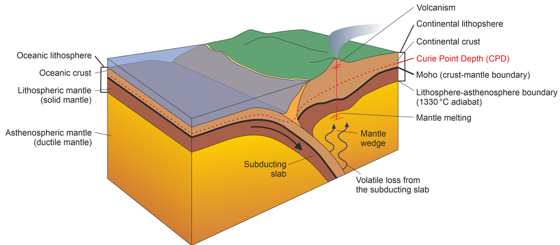
Figure 2. Basic illustration of a subduction zone at a convergent margin between oceanic and continental lithosphere to clarify the geological concepts and terms used in this paper.
