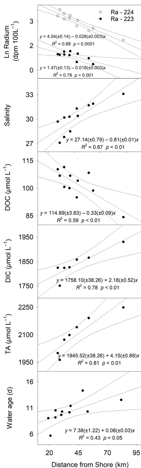
Fig 3. Offshore coastal transects of radium isotopes, salinity, TA, DIC and DOC in seawater sampled in May 2018. Water ages were calculated from ^{224}\text{Ra} : ^{223}\text{Ra} ratios. \Delta\text{TA} and \Delta\text{DIC} were used to estimate shelf scale outwelling as shown in Fig S1.
