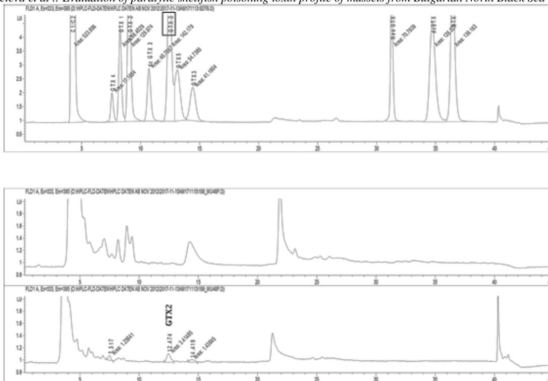
Fig. 3. HPLC-FD with post column derivatization PCOX chromatograms of a PSP standard mix containing B1, C1/2, GTX1-4, dcGTX2/3, NEO, dcSTX and STX(top) and extract of cultured mussel sample MU48P without derivatization (middle) and with derivatization (bottom).
