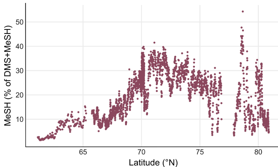
Fig. 5. Latitudinal variation of the MeSH fraction to the total sulphur compounds measured (DMS+MeSH)
