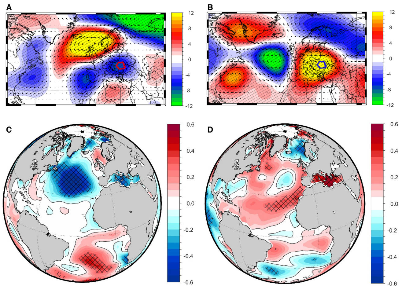
Fig. 7 a The composite map between high TRW index (> 1 SD) and April/May/June (AMJ) Geopotential height at 500 mb (Z500—Shaded colored areas) and AMJ 500 mb wind vectors (black arrows); b the composite map between low TRW index (< -1 SD) and AMJ geopotential height at 500 mb (Z500—Shaded areas) and AMJ 500
