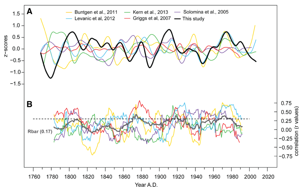
Fig. 9 Comparison with other hydroclimatic records from central and south-eastern Europe, A low-frequency variability—each curve represents a 21-yr. low-pass filter; B A 31 yrs. moving correlation between this study and five hydroclimatic raw data records (dotted line marks the positive correlation significance level at p < 0.05 , the grey line is the mean inter-series correlation ( R_{bar} ) between all individual hydroclimatic records over 31 year moving windows
