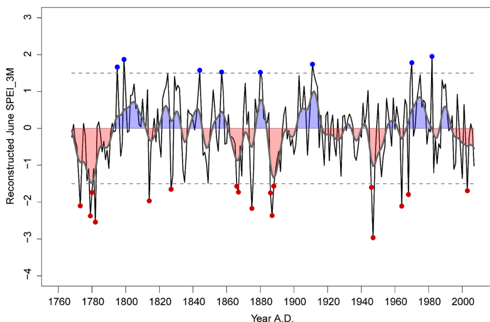
Fig. 5 The rescaled reconstructed June SPEI3 drought index for the 1768–2007 period. The gray line represents a 11-yr low-pass filter and the dashed lines depict (extreme events threshold detection) \pm 1.5 SPEI threshold, while the values above/below dashed line corresponds to very wet/dry years (additionally marked with blue and red dots)
