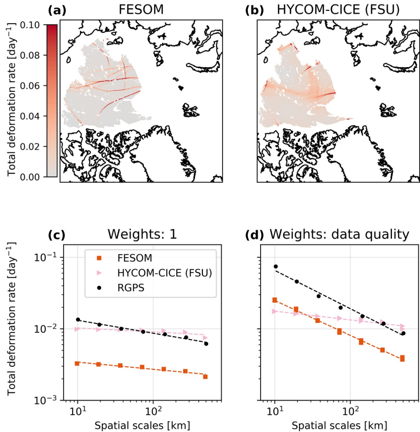
Figure 6. Top: Total deformation field snapshot for 28–30 January 1997 (in day ^{-1} ) for (a): FESOM, and (b): HYCOM-CICE (FSU); bottom: spatial scaling of total deformation rates estimated at T = 3 days in January-February-March 1997, using either (c): weights equal to one, or (d): weights equal to the signal-to-noise ratios (data quality) of the deformation estimates.
