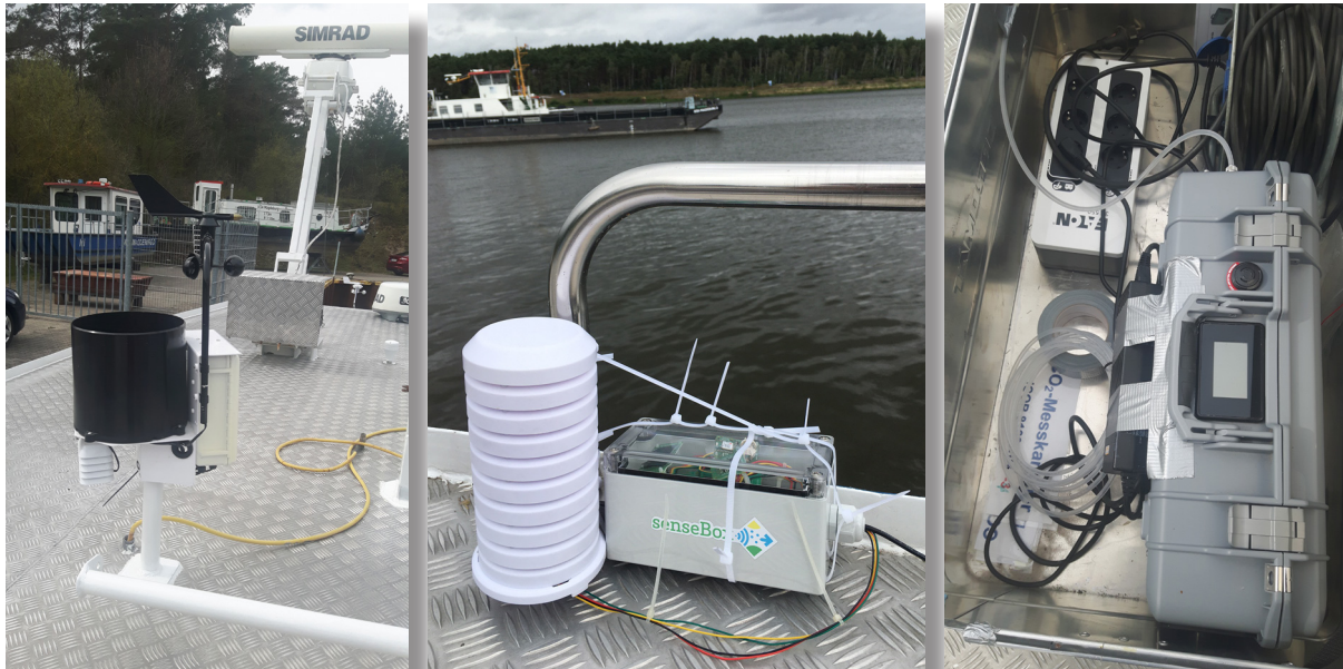
(a) WatchDog 2700 weather station; photo: U.Koedel
