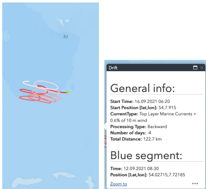
Fig. 9.5: Four day back-trajectories of water mass for a point at 54N, 7.9 E (left): The green dot indicates the start position and start time of the water mass. The red colour represents the start time, white colour depicts the position 4 days before.
