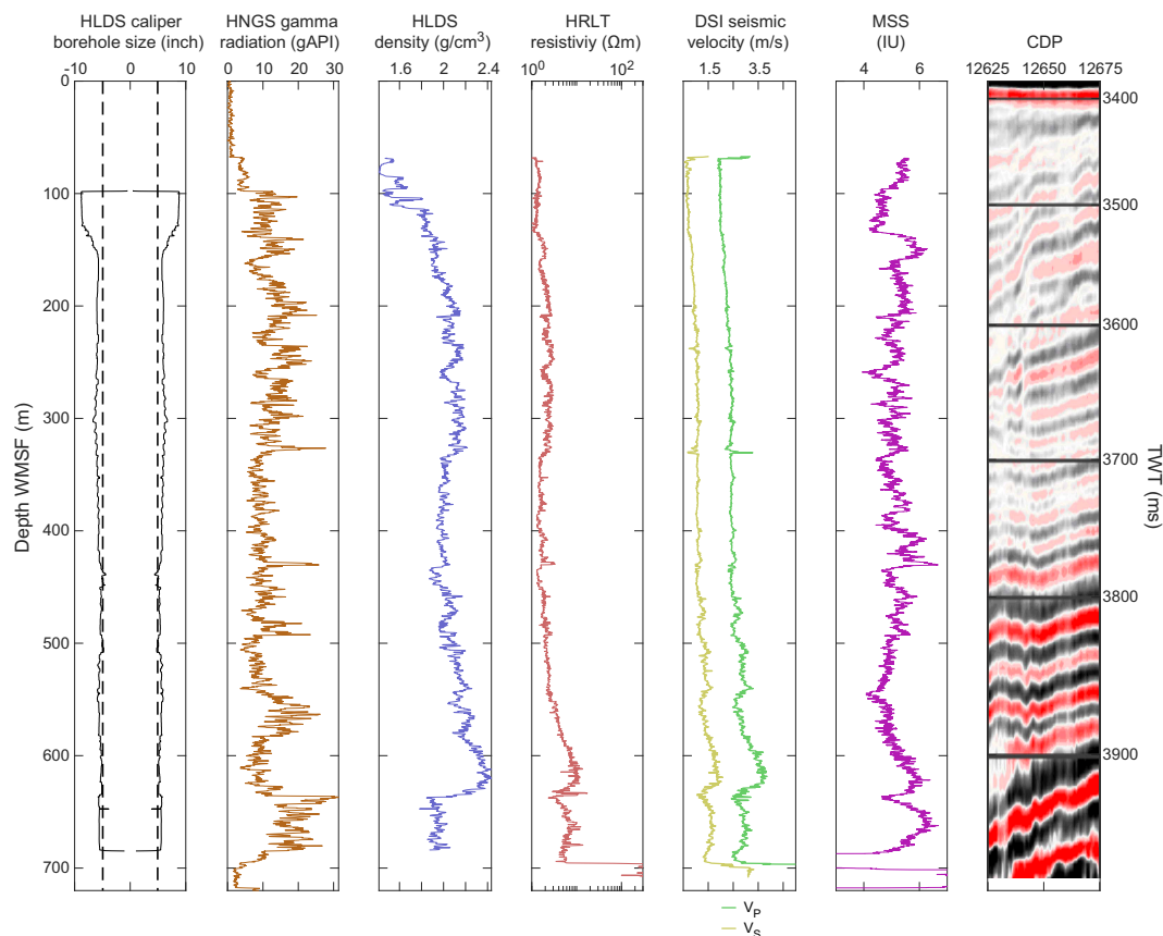
Figure F51. Downhole wireline logging results, Hole U1579D. Right column shows part of Seismic Profile AWI-20050201 in two-way travelttime (TWT) (50 traces around Site U1579, located at common depth point [CDP] 12,650). HRLT = High-Resolution Laterolog Array.
