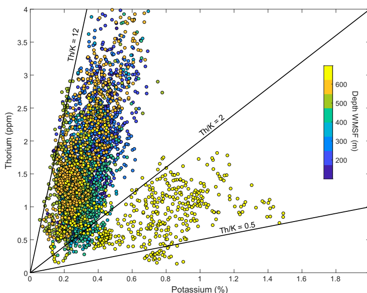
Figure F53. Crossplot of K vs. Th abundance data from the HNGS log, Hole U1579D.
