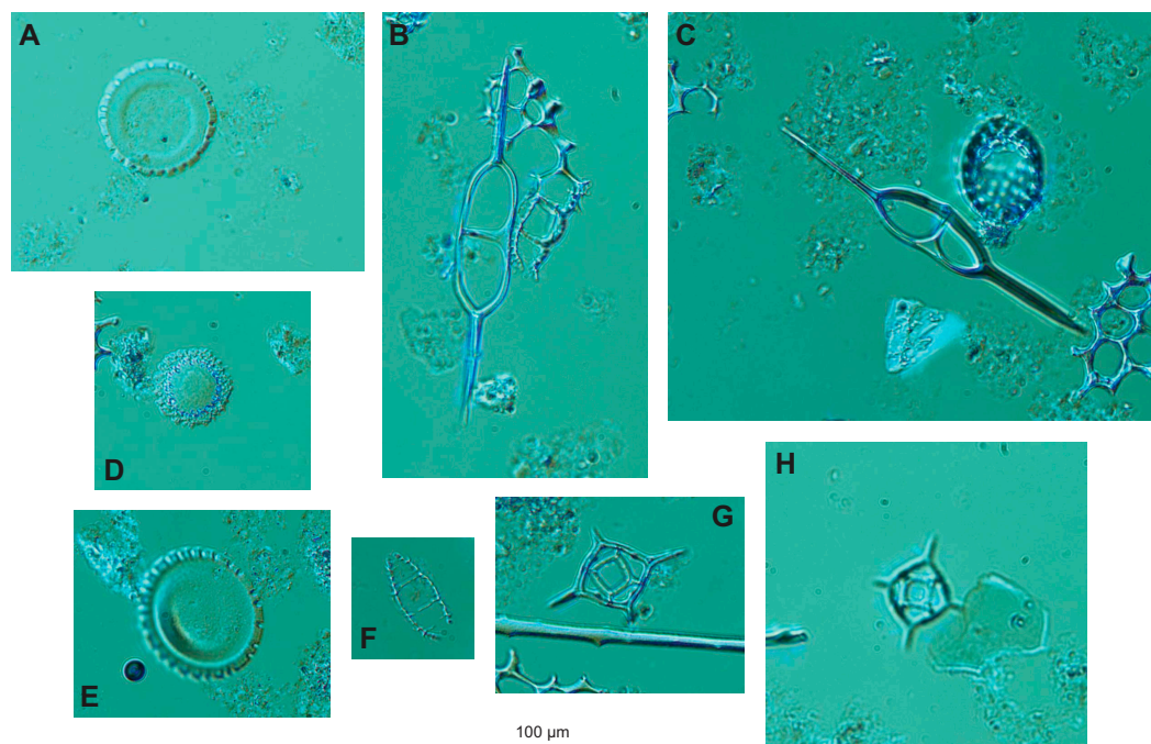
Figure F21. Selected siliceous microfossils. A, D, E. Liostephania sp. stage diatom frustules; (A) 392-U1579A-27X-CC; (D) 392-U1579D-5R-CC; (E) 392-U1579D-5R-CC. B, C. Naviculopsis biapiculata (392-U1579D-5R-CC). F. Hemiaulus sp. fragment (392-U1579D-5R-CC). G, H. Distephanus crux (392-U1579D-5R-CC).
