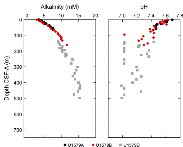
Figure F39. Alkalinity and pH, Site U1579.
