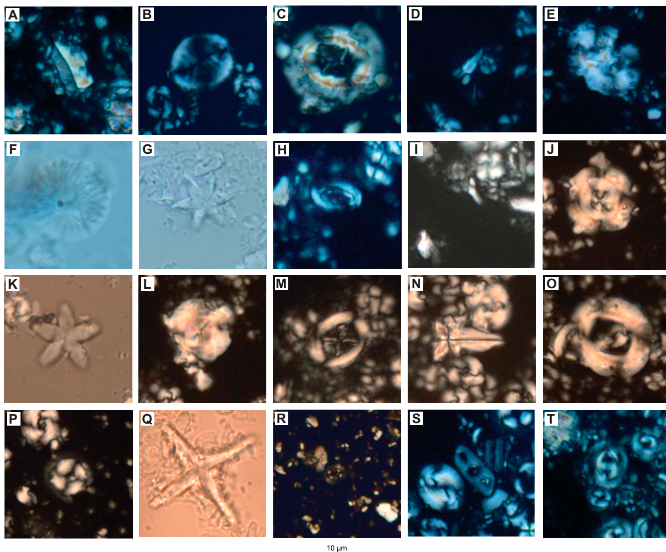
Figure F17. Select Paleogene calcareous nanofossils. Scale bars = 10 µm. A. Zygrhablithus bijugatus (392-U1579D-19R-CC). B. Reticulofenestra oamaruensis (392-U1579C-25X-1, 13 cm). C. Pletolithus gigas (392-U1579D-11R-2, 105 cm). D. Furcatolithus distentus (392-U1579A-6R-CC). E. Ellipsolithus macellus (392-U1579D-15R-CC). F. Discoaster multiradiatus (392-U1579D-19R-CC). G. Discoaster lodoensis (392-U1579D-12R-3, 80 cm). H. Campylosphaera eodela (392-U1579D-15R-CC). I. Furcatolithus ciproensis (392-U1579A-4H-CC). J. Reticulofenestra isabellae (392-U1579D-6R-CC). K. Discoaster tanii? (392-U1579B-27X-CC). L. Reticulofenestra bisecta > 10 µm (392-U1579B-26X-2, 57 cm). M. Chiasmolithus altus (392-U1579A-8H-CC). N. Sphenolithus pseudoradians (392-U1579B-24F-CC). O. Reticulofenestra umbilicus > 14 µm (392-U1579B-26X-CC). P. Coccolithus formosus (392-U1579B-25X-CC). Q. Nannotetrina fulgens (392-U1579D-10R-CC). R. Cruciplacolithus primus (392-U1579D-33R-5, 70–71 cm). S. Isthmolithus recurvus (392-U1579D-5R-CC). T. Toweius eminens (392-U1579D-19R-CC).
