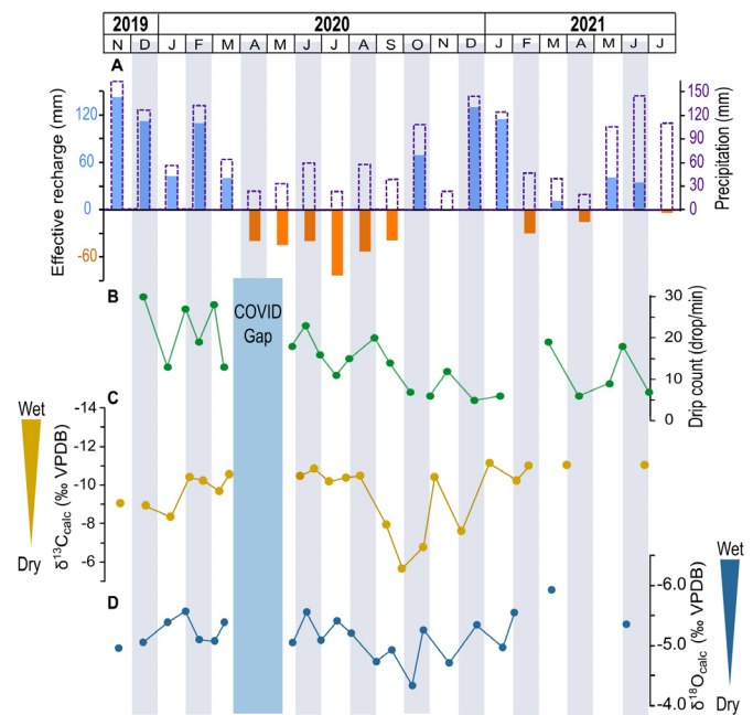
Fig. 6. Monthly precipitation and effective recharge at station Rouen-Boss; Data source: Météo France (A), compared to CAU-2 drip rate (B), modern carbonate \delta^{13}\text{C} (C), and modern \delta^{18}\text{O} (D). Effective recharge is calculated using the Thornthwaite equation (Palmer & Havens, 1958). The significant increase in \delta^{13}\text{C} values between September and December 2020 might reflect the hydrological (increased PCP) response to the prolonged lack of infiltration over the spring and summer of 2020 (shown in A).
