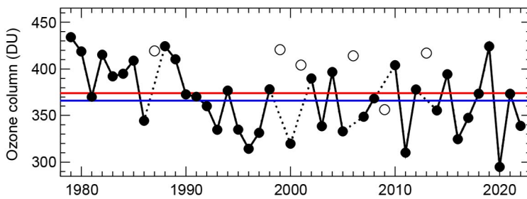
Fig. 5.32. Minimum of the daily average total ozone column (Dobson units, DU) for Mar poleward of 63°N equivalent latitude (Butchart and Remsberg 1986). Open circles represent years in which the polar vortex was not well-defined in Mar, resulting in relatively high values owing to mixing with lower-latitude air masses and a lack of significant chemical ozone depletion. Red and blue lines indicate the average total ozone column for 1979–2021 and 2005–21, respectively. Ozone data for 1979–2019 are based on the combined NIWA-BS total column ozone database version 3.5.1 (Bodeker and Kremser 2021). Ozone data for 2020–22 are from OMI. Adapted from Müller et al. (2008) and WMO (2022), and updated using ERA5 reanalysis data (Hersbach et al. 2020) to determine equivalent latitude.
