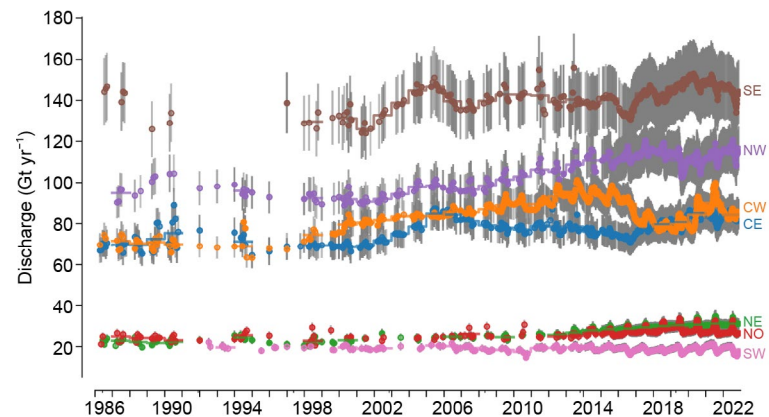
Fig. 5.18. Solid ice discharge (Gt yr -1 ) based on ice velocity and thickness (Mankoff et al. 2020) by region of the Greenland Ice Sheet, as shown in Fig. 5.16a. Gray bars show uncertainty of \pm 10\% .
