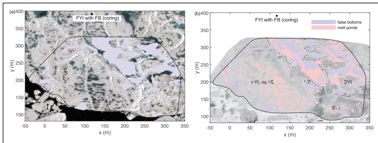
Figure 10. Locations of false bottoms and surface melt ponds. (a) Co-location of a satellite image of the ice floe from Planet Lab, Inc. (from Webster et al., 2022) and (b) ice draft from remotely operated vehicle (ROV) multibeam sonar, from July 1. Blue-shaded areas show estimate of false bottom (FB) coverage, and red-shaded areas show estimate of melt ponds (MP) within ROV scans. The ROV scan overlap area is encompassed by a solid black line.
