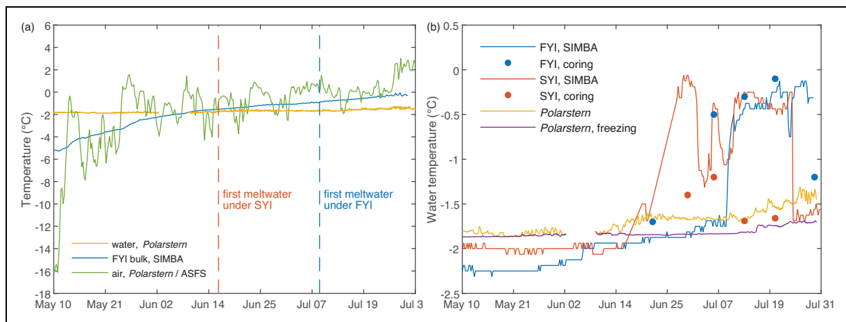
Figure 3. Evolution of air, ice, and water temperatures. (a) The 6-hour mean air temperature from Polarstern , first-year ice (FYI) bulk temperature from sea ice mass balance array (SIMBA) over the whole ice column, in situ water temperature from the Polarstern thermosalinograph at 11-m depth, and (b) ice bottom temperature from SIMBA and coring sites, in situ water temperature and freezing temperature estimated from salinity measurements from the Polarstern thermosalinograph at 11-m depth. While Polarstern left the MOSAiC floe from mid-May to mid-June 2020, air temperature measurements were provided by an Atmospheric Surface Flux Station (ASFS).
