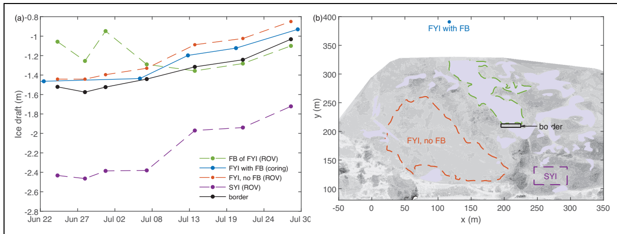
Figure 6. Ice draft evolution from remotely operated vehicle (ROV) multibeam sonar. (a) Draft evolution of false bottom (FB) below first-year ice (FYI), of FYI with and without false bottom, of second-year ice (SYI), and of the border between under-ice meltwater layers measured by ROV multibeam sonar, and (b) locations of corresponding ice types.
