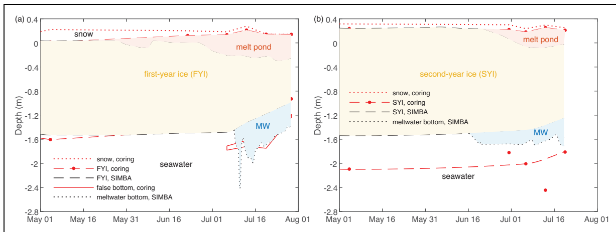
Figure 5. Depth evolution of snow, sea ice, meltwater, and false bottoms during melt season. Depth of snow, sea ice, meltwater (MW), and false bottom interfaces from coring and from sea ice mass balance arrays (SIMBAs) for (a) first-year ice (FYI) and (b) second-year ice (SYI). The depth for SIMBAs was estimated with an assumption of equal bottom melt for coring and for SIMBAs sites. The layer between meltwater and seawater shown by dotted lines represents the estimate of false bottom location, identified by a significant vertical temperature gradient as in Figure 2b .
