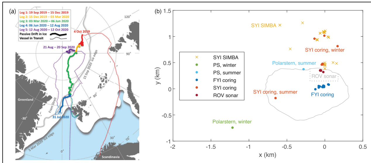
Figure 1. Locations of the Central Observatory and the main observation sites during MOSAiC. (a) Locations of the drifting Central Observatory (solid) and Polarstern cruise track (dotted) during MOSAiC, with the sea ice edge at the annual maximum and minimum, from Shupe et al. (2020), and (b) locations of first-year ice (FYI) and second-year ice (SYI) coring sites, the remotely operated vehicle (ROV) sonar scan area, and Polarstern relative to the snow ice mass balance array (SIMBA) buoys in the MOSAiC Central Observatory during summer 2020, with the FYI SIMBA buoy at (0,0). The gray line represents Central Observatory floe outlines for July 22, 2020.
