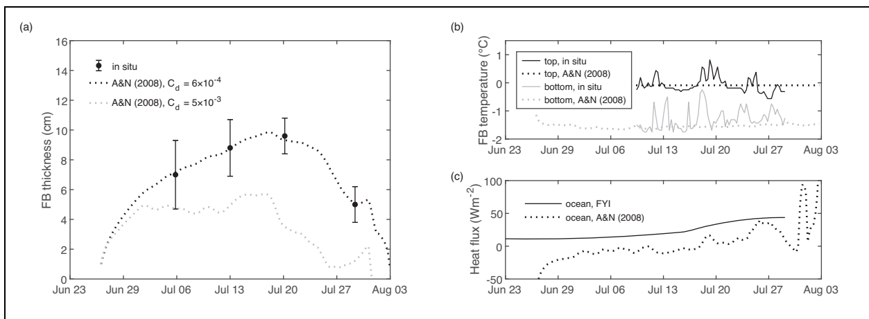
Figure 8. False bottom temperature, thickness, and ocean heat flux. We used the false bottom thermodynamic model from Alexandrov and Nizovtseva (A&N) (2008) with forcing from in situ measurements of drift speed, seawater temperature and salinity from Polarstern . (a) False bottom (FB) thickness, measured in situ at the first-year ice (FYI) coring site and estimated using the model, (b) top and bottom temperature of false bottom measured by FYI SIMBA and estimated using the model, and (c) ocean heat flux, estimated from FYI SIMBA measurements and from the model.
