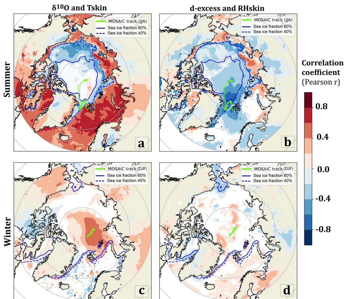
Figure 3. Seasonal correlation maps (Pearson's r at 99.9% confidence interval) of water vapor \delta^{18}O and skin temperature T_{skin} (a, c) and d-excess and relative humidity RH_{skin} (b, d). Panels (a) and (b) show the Arctic summer (JJA), c and d the winter season (DJF). The blue lines mark the area of sea fraction higher than 80% (solid) and 40% (dashed), respectively. Correlation coefficients were calculated based on the 3hr resolution data sets at all locations north of 60^\circ N , assuming no time lag.
