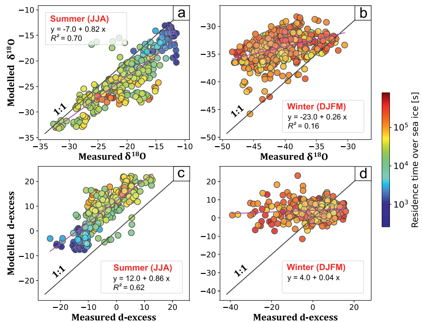
Figure 6. Seasonal scatterplots illustrating the relationships between measured and modeled \delta^{18}\text{O} (a, b) and d-excess (c, d) in summer (JJA, left) and winter (DJFM, right) respectively. The data are aggregated at 6 hr time resolution and they are colored in logarithmic scale based on the residence time (s) over sea-ice retrieved from the 10-day FLEXPART backward trajectories. Linear regressions are shown as pink solid lines.
