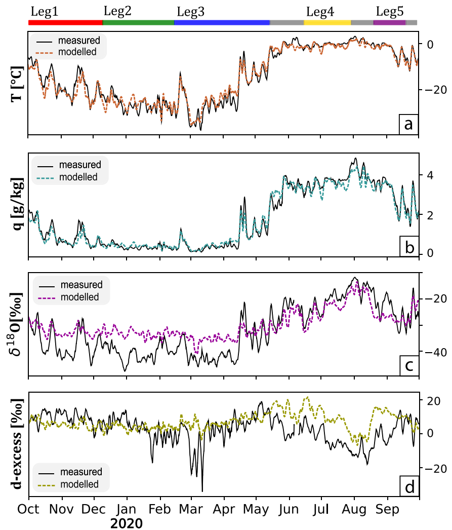
Figure 5. Time series (from 1 October 2019 to 30 September 2020) of ECHAM6-wiso model results of the nearest surface grid box, and observations along the track of RV Polarstern during the Multidisciplinary drifting Observatory for the Study of Arctic Climate expedition. The subplots report modeled and measured (a) air temperature T ( ^{\circ}\text{C} ); (b) water vapor specific humidity q ( \text{g kg}^{-1} ); (c) water vapor \delta^{18}\text{O} ( \text{‰} ); and (d) water vapor d-excess ( \text{‰} ). All values are averaged over a moving window of 48 hr.
