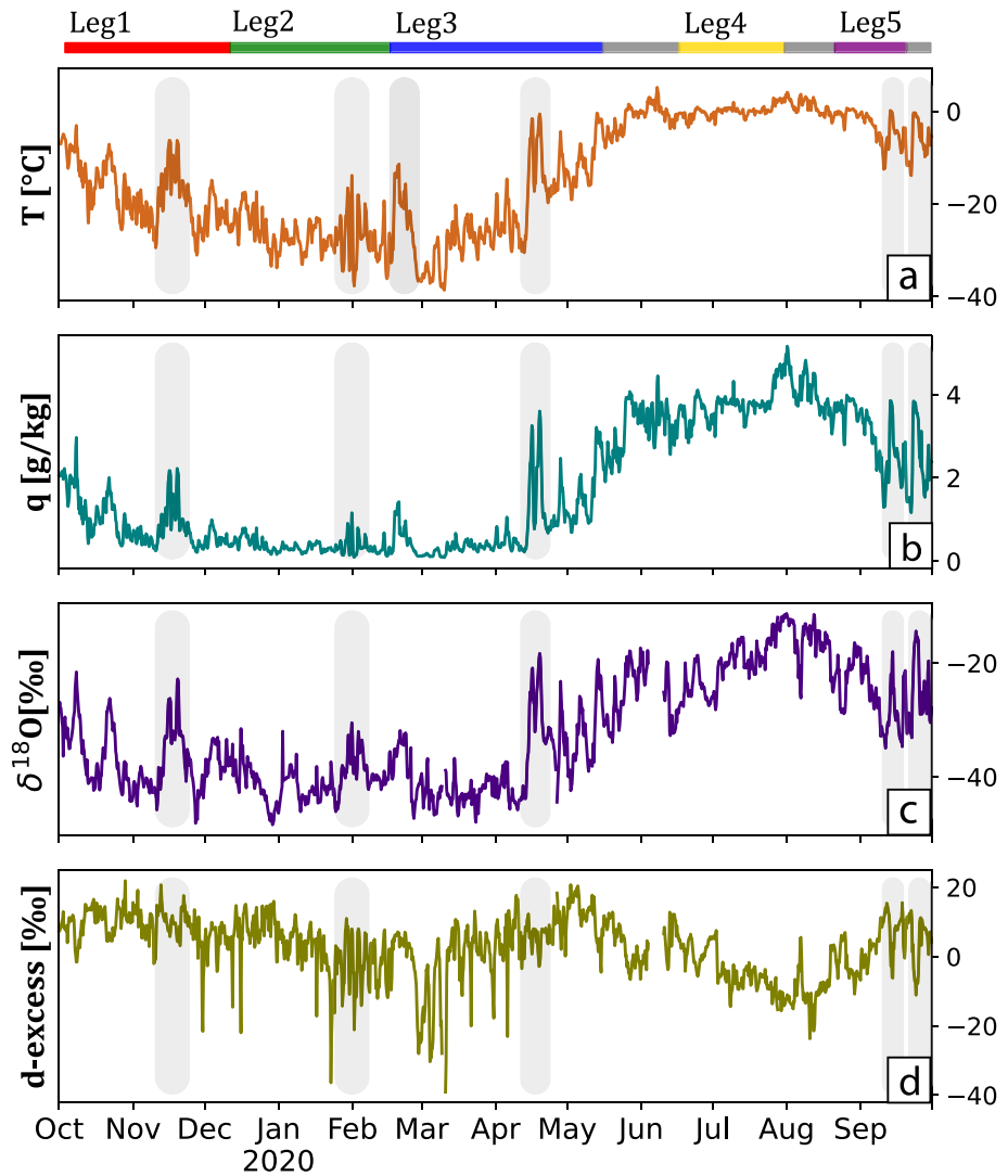
Figure 2. From top to bottom: (a) temperature T , (b) humidity q , (c) \delta^{18}\text{O} , and (d) d-excess of atmospheric water vapor measured at 19 m on the mast of RV Polarstern during the Multidisciplinary drifting Observatory for the Study of Arctic Climate expedition in the Central Arctic, aggregated here at 6 hr resolution. The time span of each phase of the expedition (named Legs, Figure 1) is illustrated in the upper bar, the active transfer of RV Polarstern is shown as a gray phase. Vertical shaded gray bars in panels (a–d) mark the occurrence of synoptic warm air intrusions.
