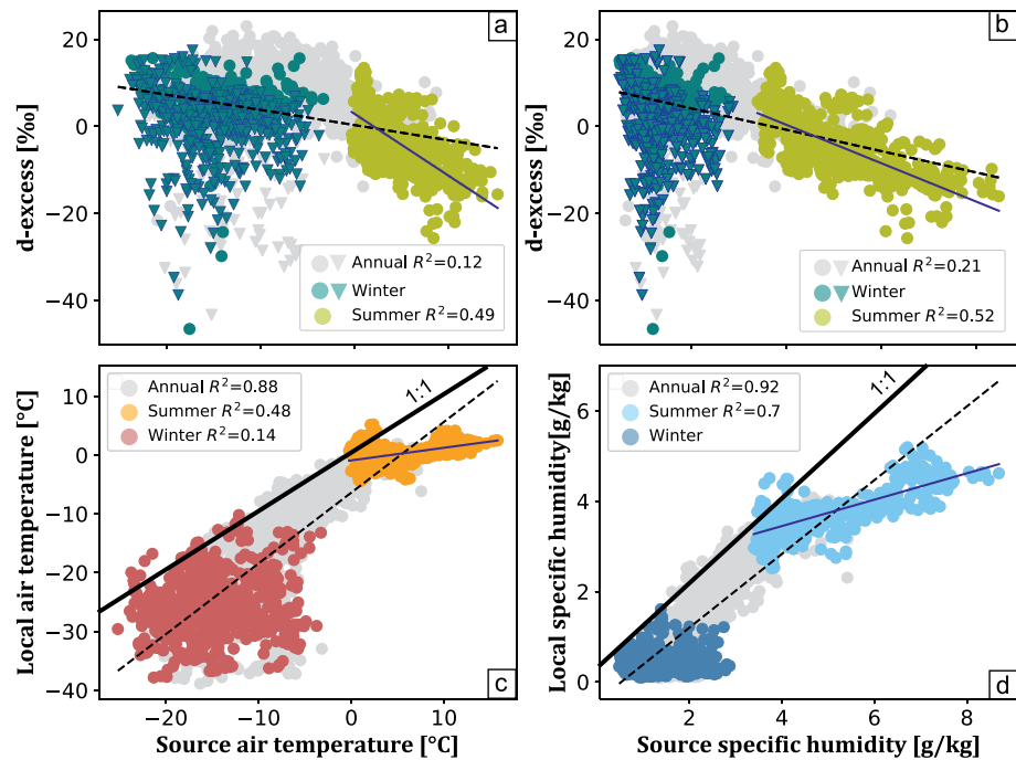
Figure 8. Upper panels: scatterplots of atmospheric water vapor d-excess and air temperature (a) and specific humidity (b) averaged over the moisture uptake regions. Lower panels: scatterplots of local and source air temperature (c) and specific humidity (d). The local meteorological data are obtained from the weather station operated on board of Polarstern, the source meteorological data are obtained from the ERA5 reanalyses from the European Centre for Medium-range Weather Forecasts. All data sets are aggregated at 3 hr time resolution. Regression lines for the annual data sets are illustrated as a dashed black line while regression lines for the summer values are illustrated by the blue solid line.
