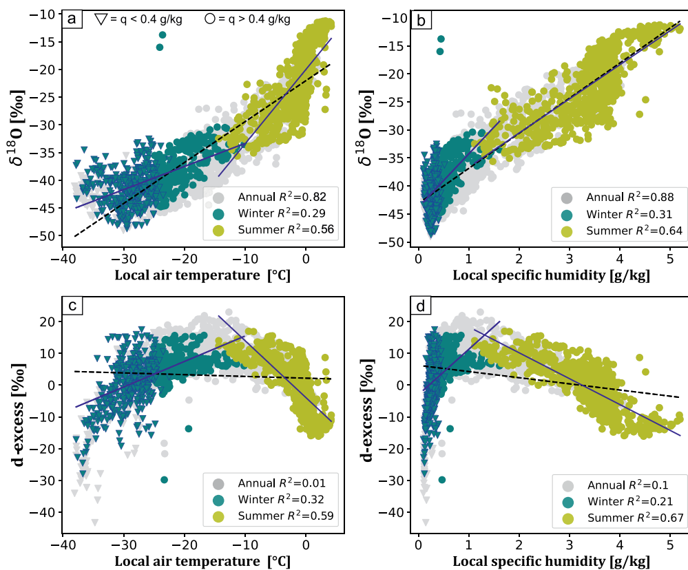
Figure 7. Scatterplots of water vapor \delta^{18}\text{O} (top) and d-excess (bottom) versus local air temperature (left) and local specific humidity (right), here aggregated at 3 hr resolution. The annual data set (October 2019–September 2020) is displayed in gray, summer (JJA) values are colored in light green and winter (DJF) values in teal. Values retrieved in humidity conditions lower than 0.4 \text{ g kg}^{-1} are marked as triangles, else as circles. The linear regression line for the annual data set is illustrated as a black dashed line; seasonal linear regressions in blue.
