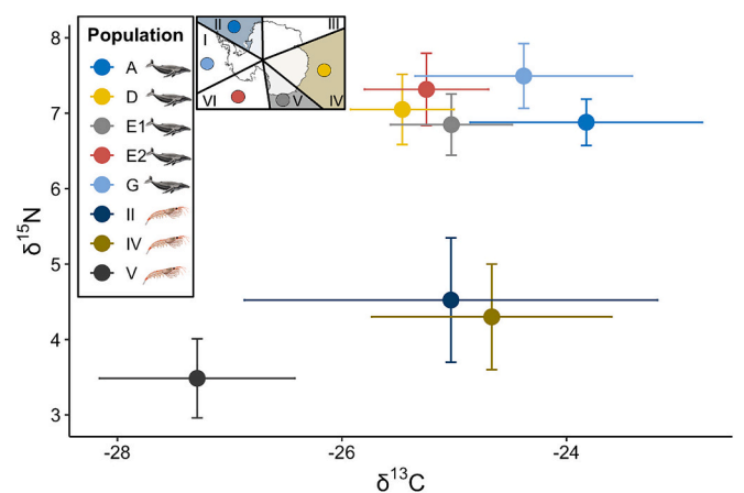
Fig. 4. Biplot showing the mean and standard deviation of skin (S) \delta^{13}\text{C} and \delta^{15}\text{N} of A, D, E1, E2 and G (S = 30, 40, 21, 26, 27; sampled off Brazil, west Australia, east Australia, New Caledonia and Colombia in 2019, respectively) humpback whale populations and \delta^{13}\text{C} and \delta^{15}\text{N} of whole krill caught in IWC management areas II, IV and V ( n = 36, 8, 3 , respectively). IWC management areas (denoted by Roman numerals I-VI) where krill samples were caught are shown as shaded areas in the map insert, which also indicates the areas in which each population (denoted with coloured circles) is thought to feed during the austral summer.
